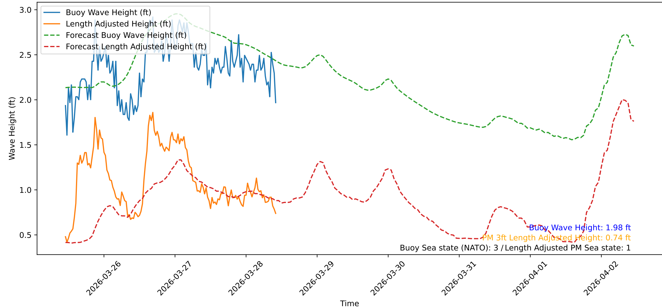
Wave Heights over Time for Oceanside Harbor at 2026-03-28 11:00:31
