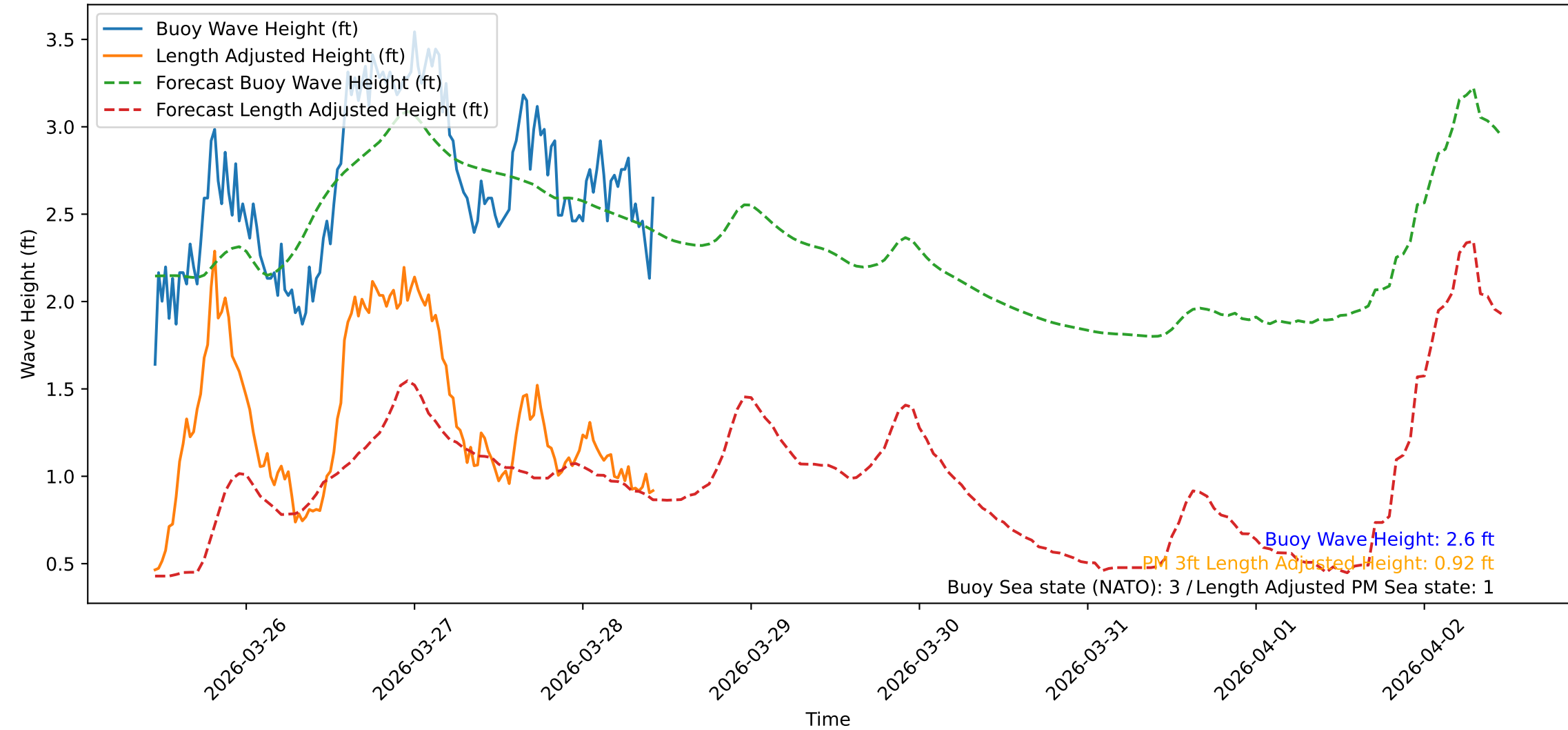
Wave Heights over Time for Green Beach at 2026-03-28 11:01:10
