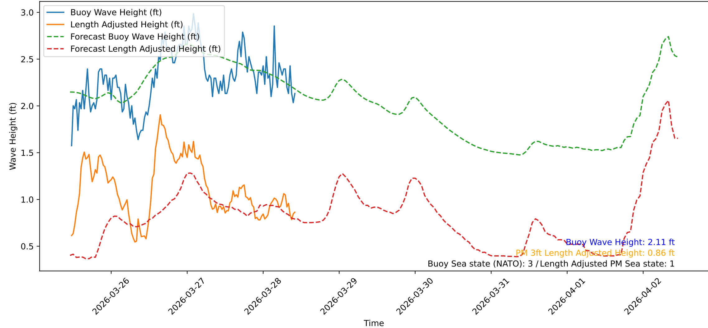
Wave Heights over Time for Red Beach at 2026-03-28 11:00:47
