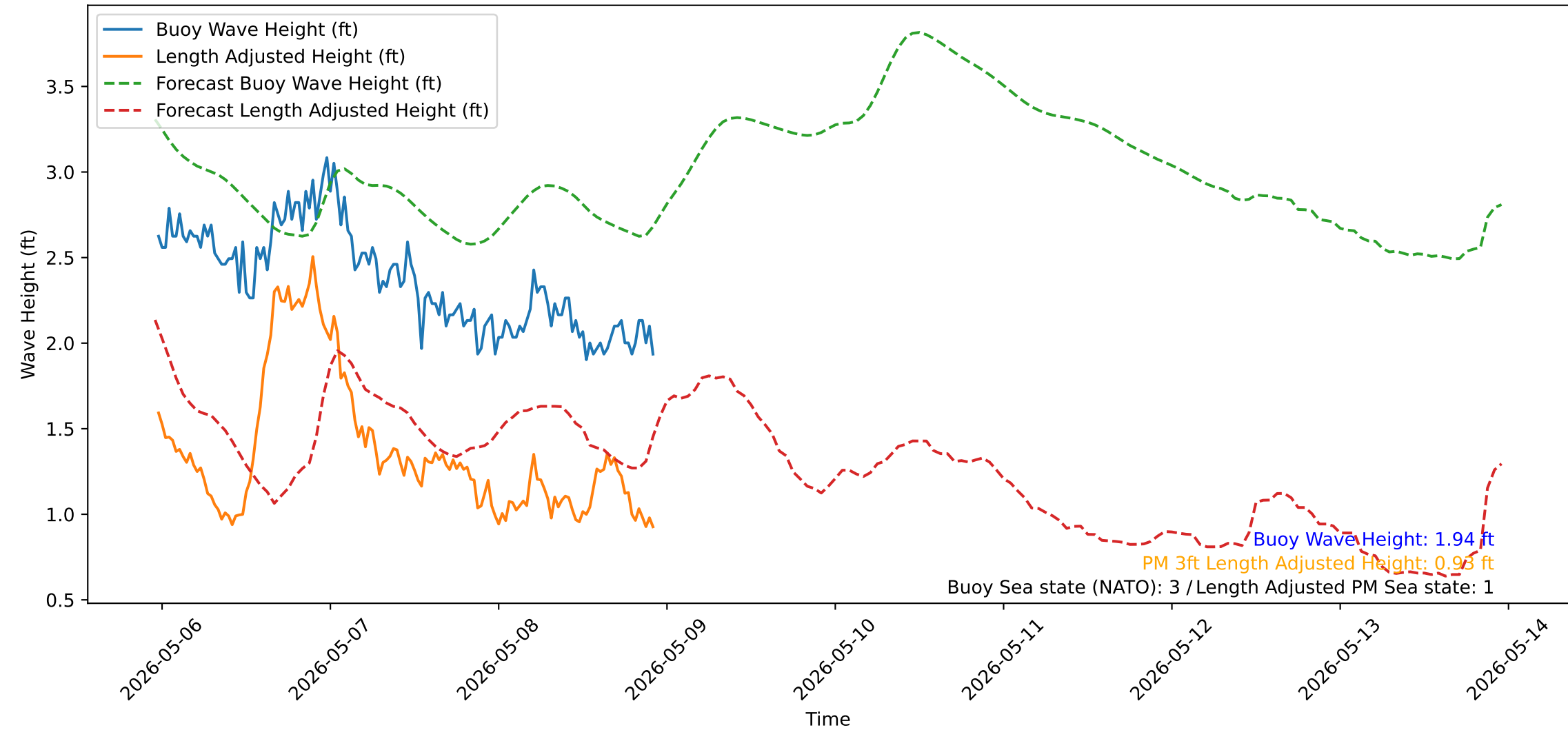
Wave Heights over Time for Red Beach at 2026-05-08 23:00:51
