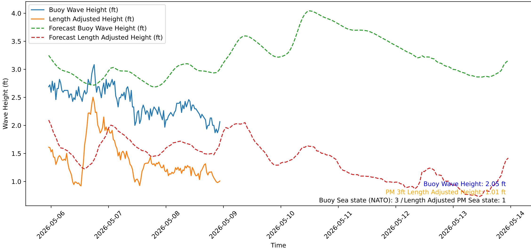
Wave Heights over Time for Oceanside Harbor at 2026-05-08 23:00:31
