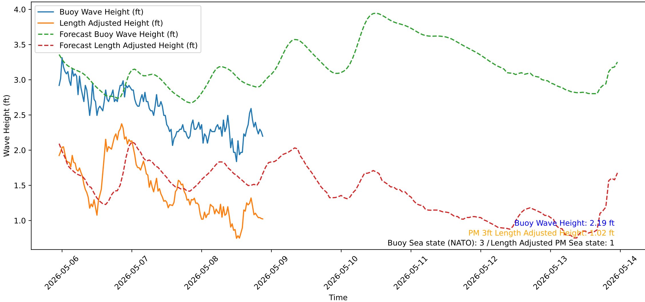
Wave Heights over Time for Green Beach at 2026-05-08 23:01:13
