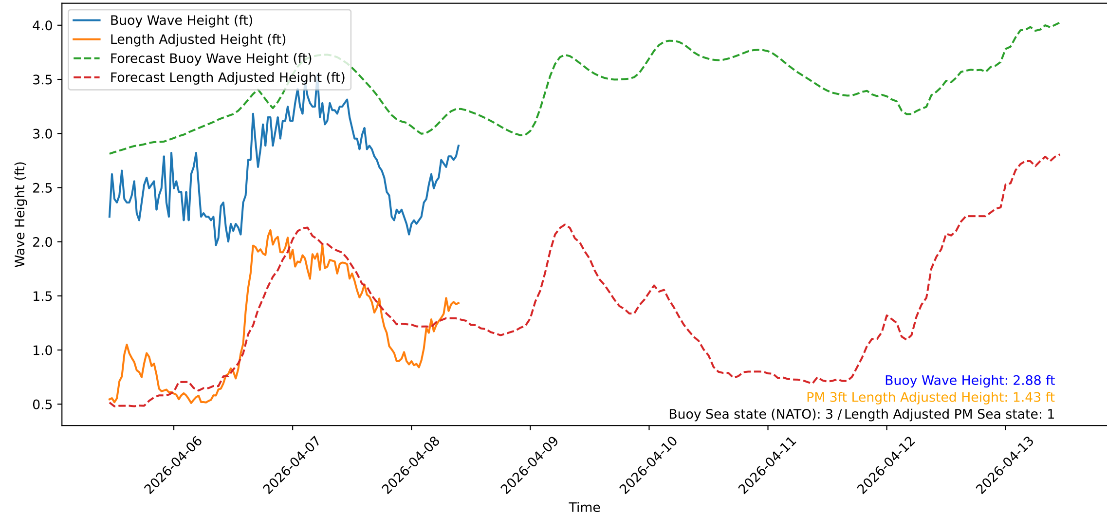
Wave Heights over Time for Red Beach at 2026-04-08 10:30:47
