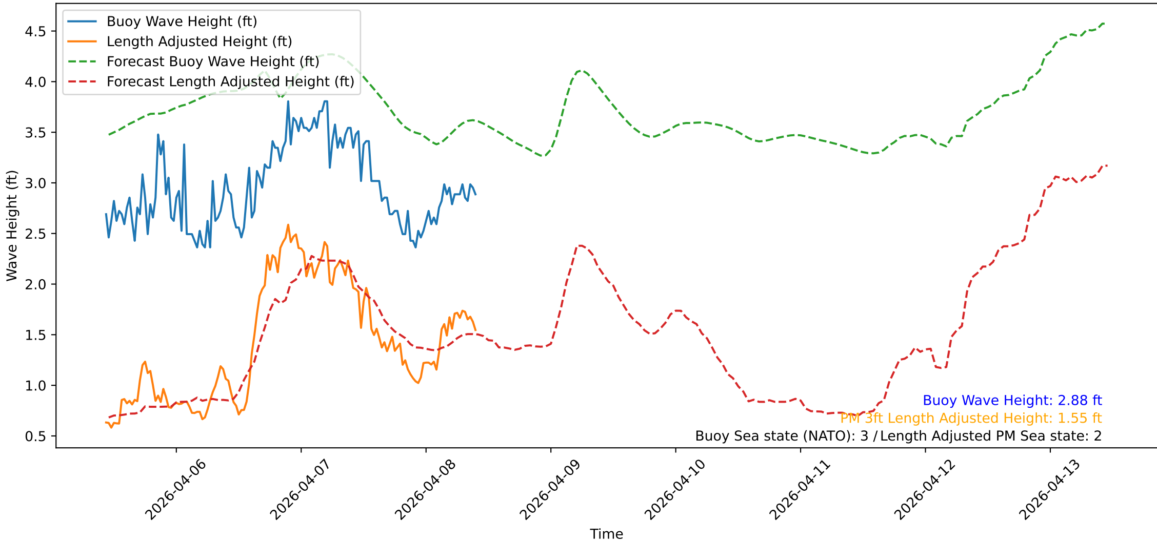
Wave Heights over Time for Green Beach at 2026-04-08 10:31:09
