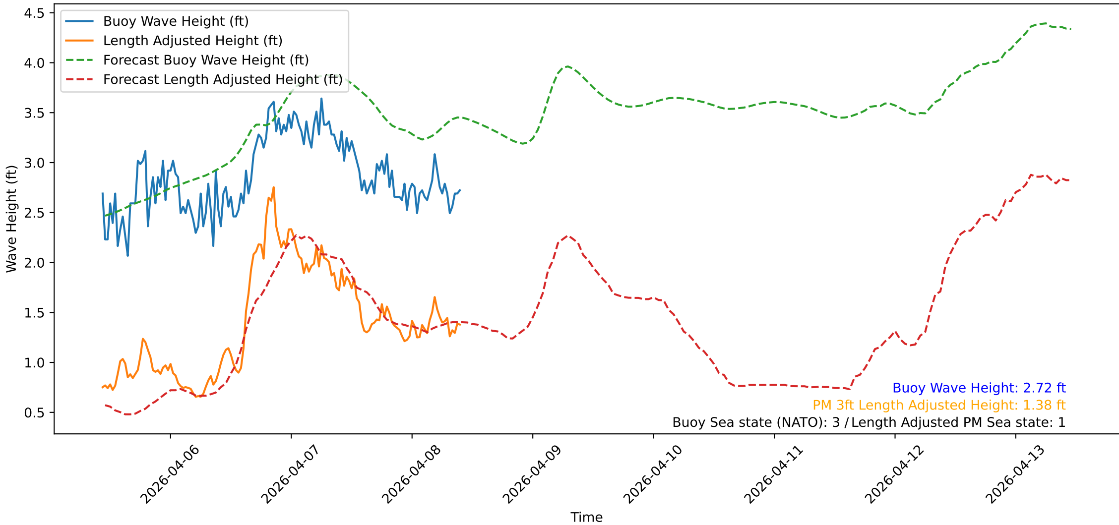
Wave Heights over Time for Oceanside Harbor at 2026-04-08 10:30:31
