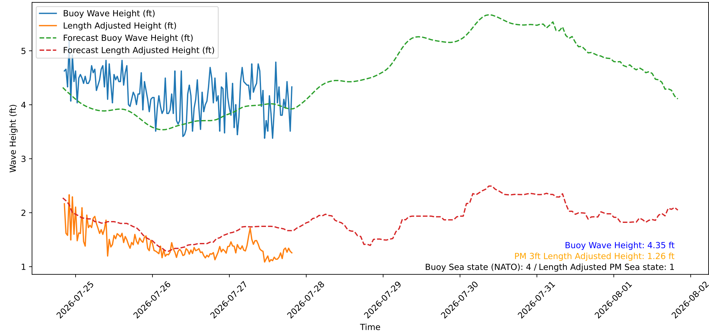
Wave Heights over Time for Green Beach at 2026-07-27 20:21:10
