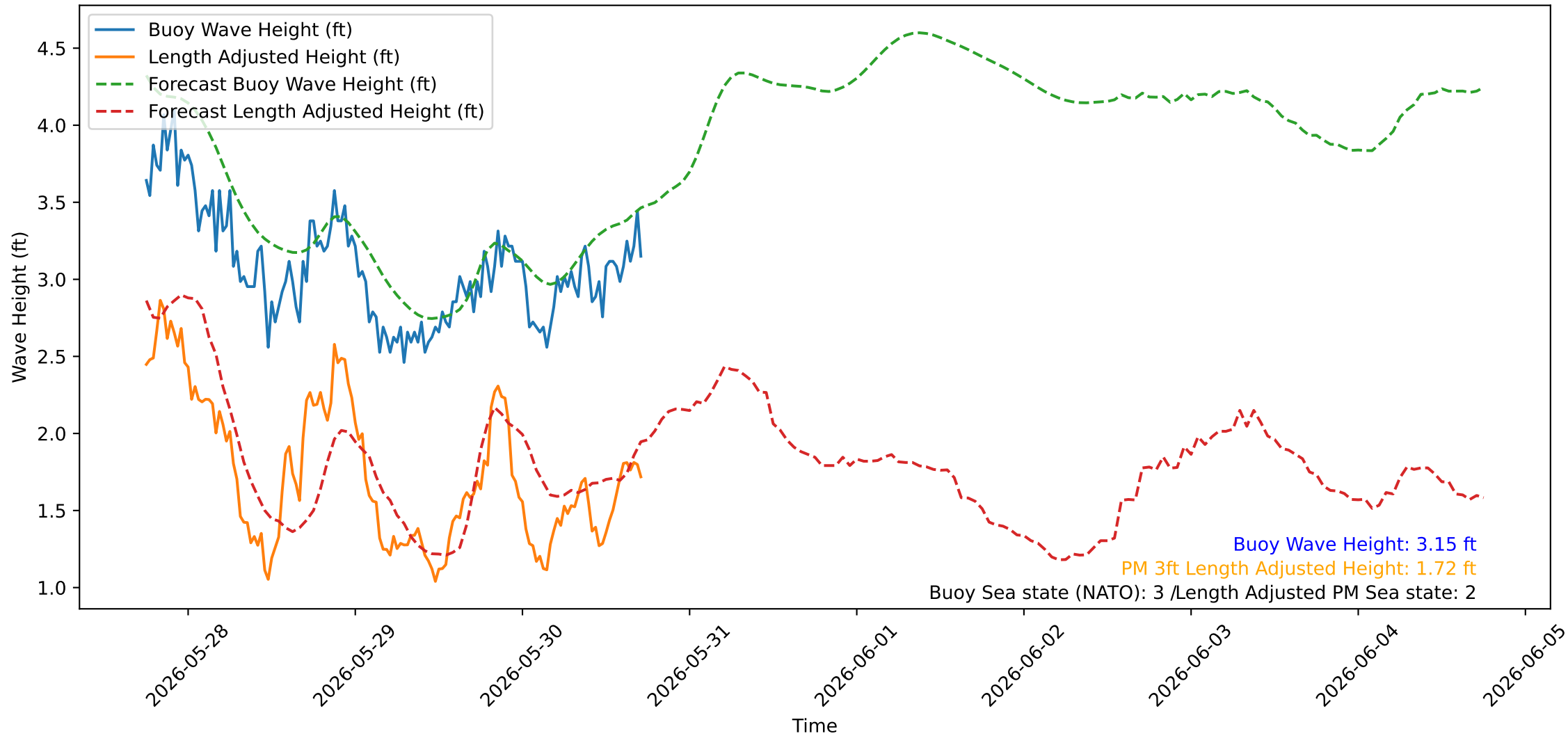
Wave Heights over Time for Green Beach at 2026-05-30 17:51:07
