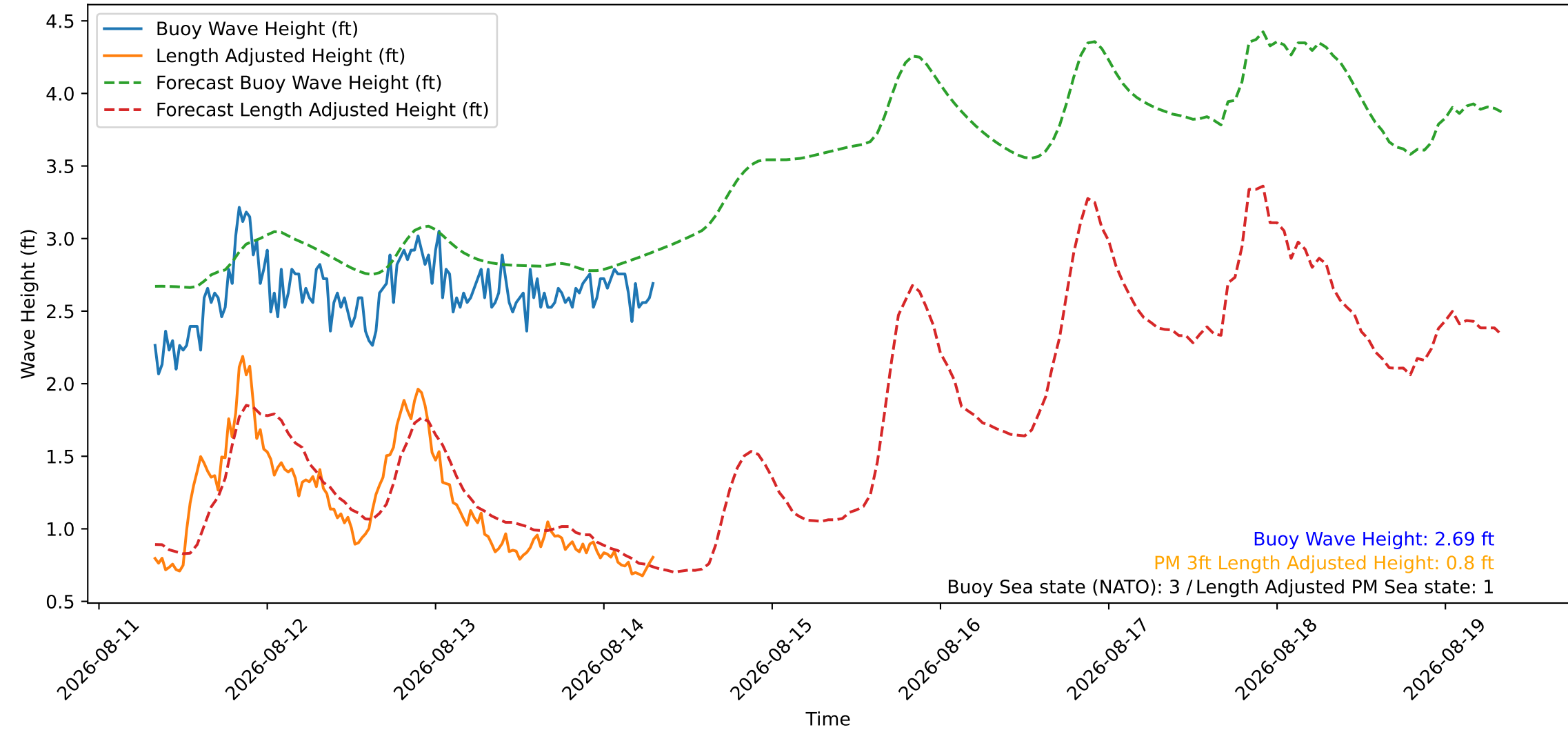
Wave Heights over Time for Green Beach at 2026-08-14 07:51:10
