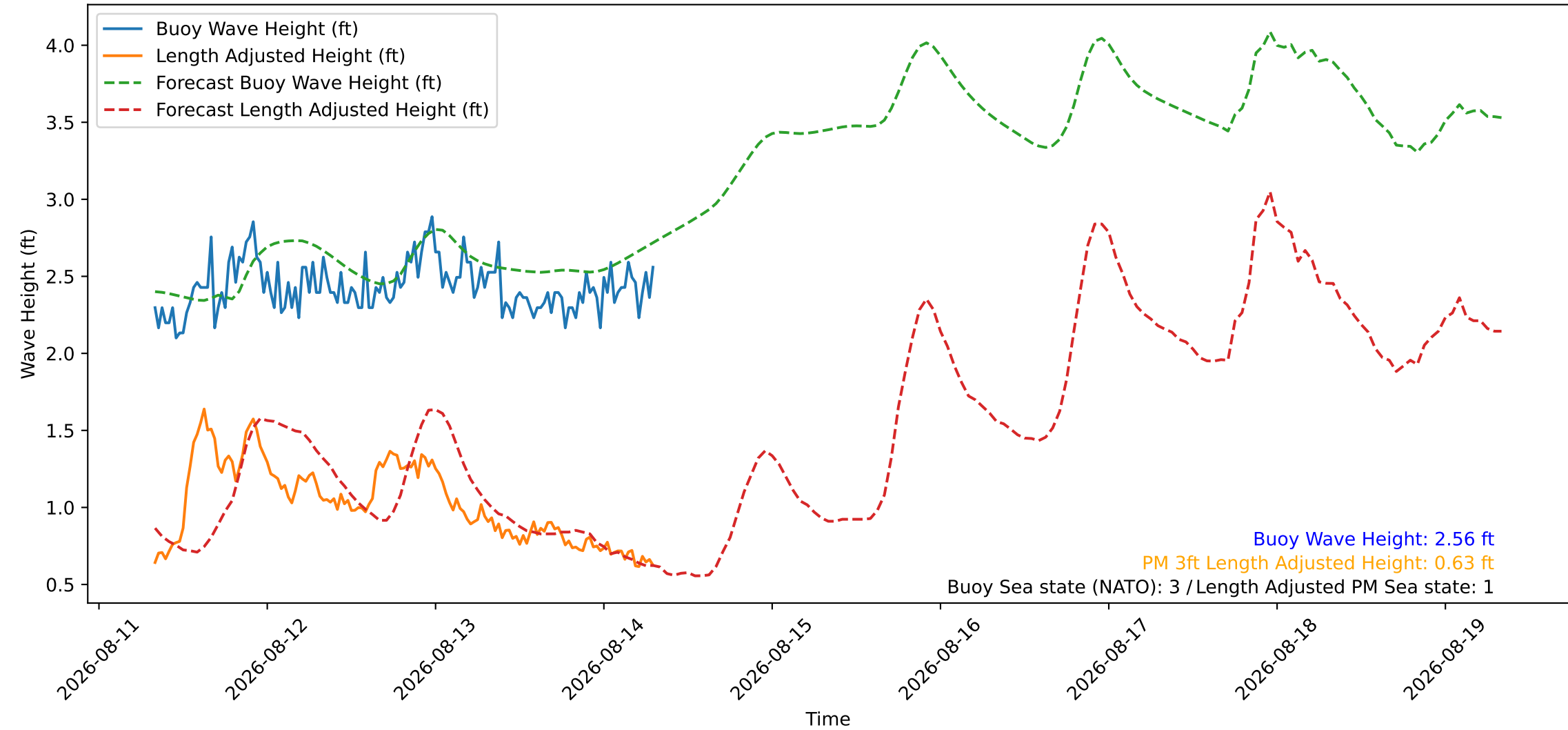
Wave Heights over Time for Red Beach at 2026-08-14 07:50:47
