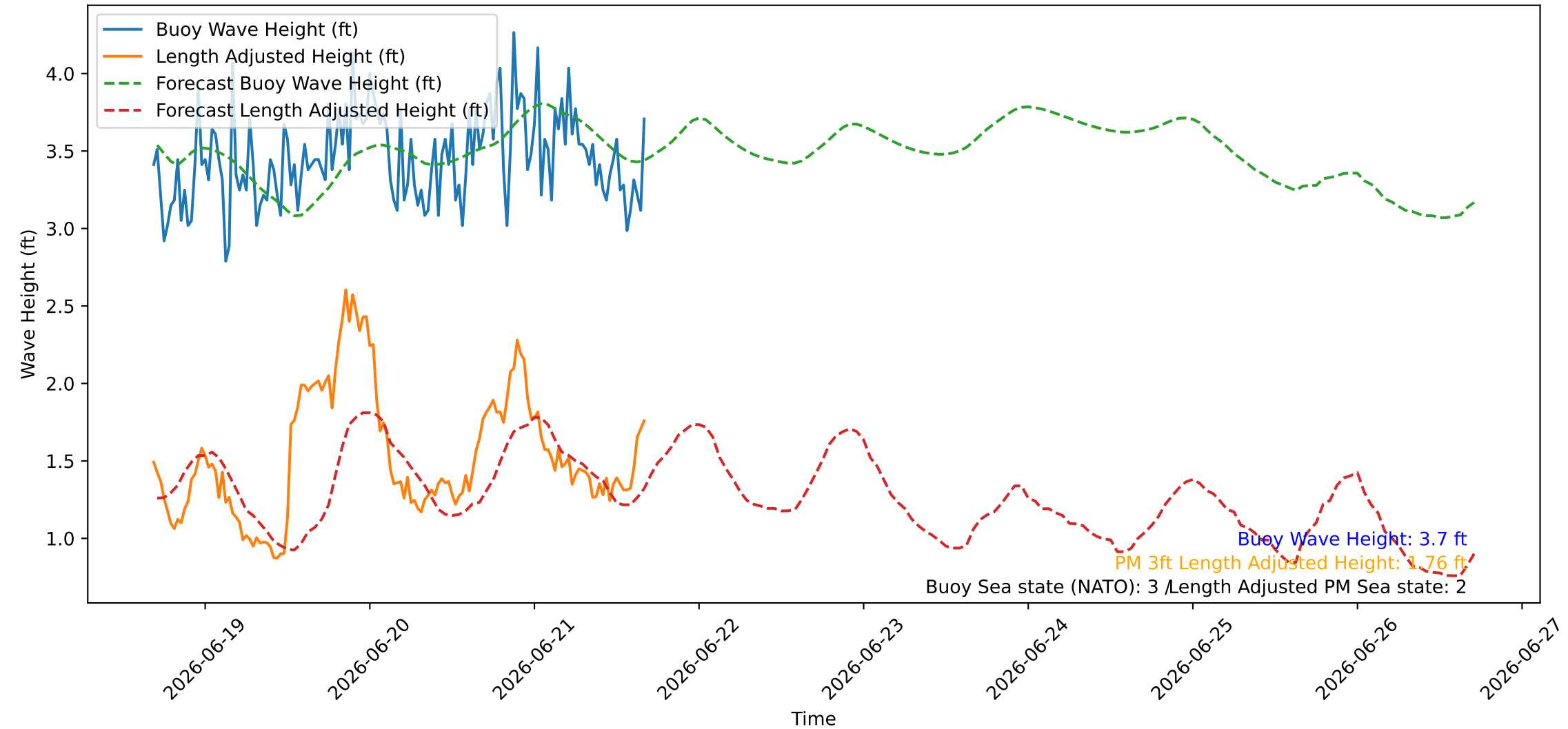
Wave Heights over Time for Oceanside Harbor at 2026-06-21 16:40:25
