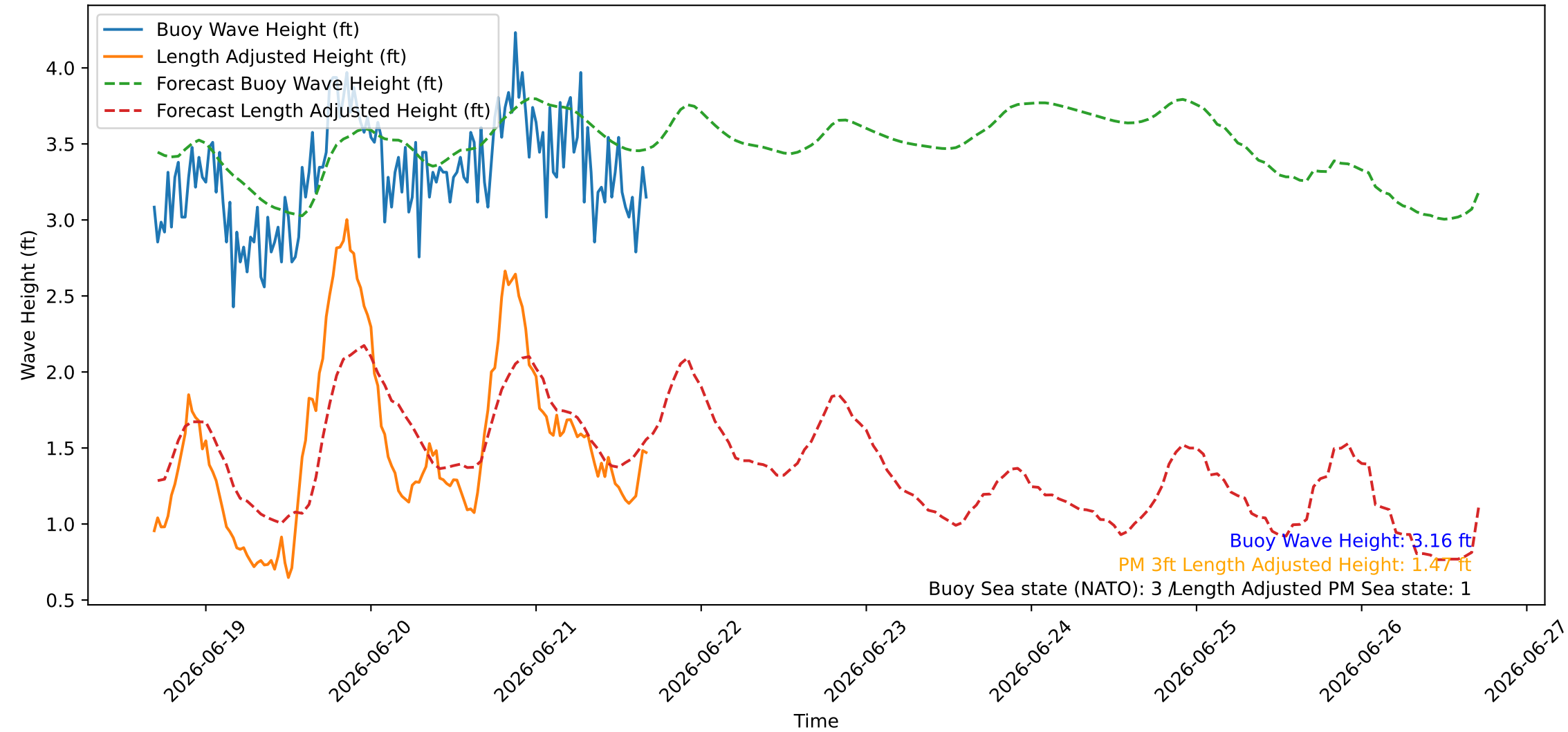
Wave Heights over Time for Green Beach at 2026-06-21 16:41:08
