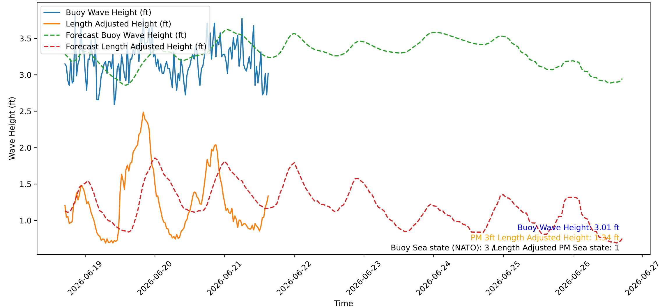
Wave Heights over Time for Red Beach at 2026-06-21 16:40:45
