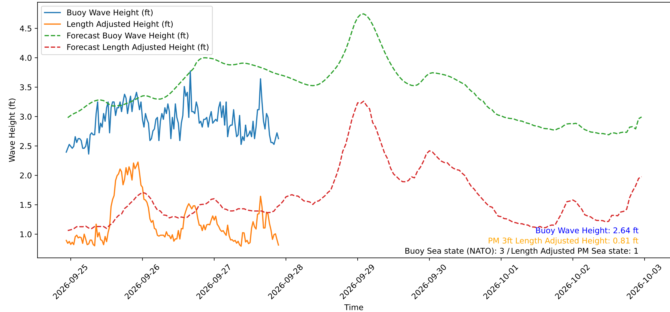
Wave Heights over Time for Oceanside Harbor at 2026-09-27 22:30:30
