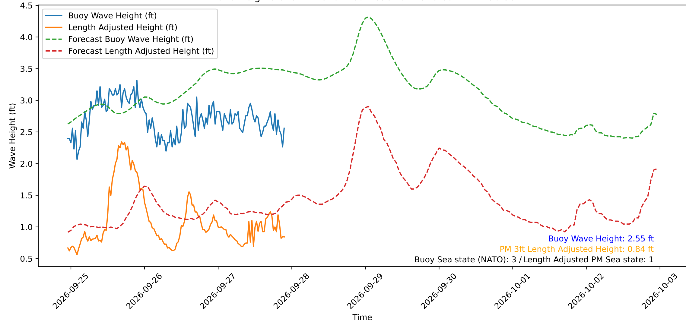
Wave Heights over Time for Red Beach at 2026-09-27 22:30:50
