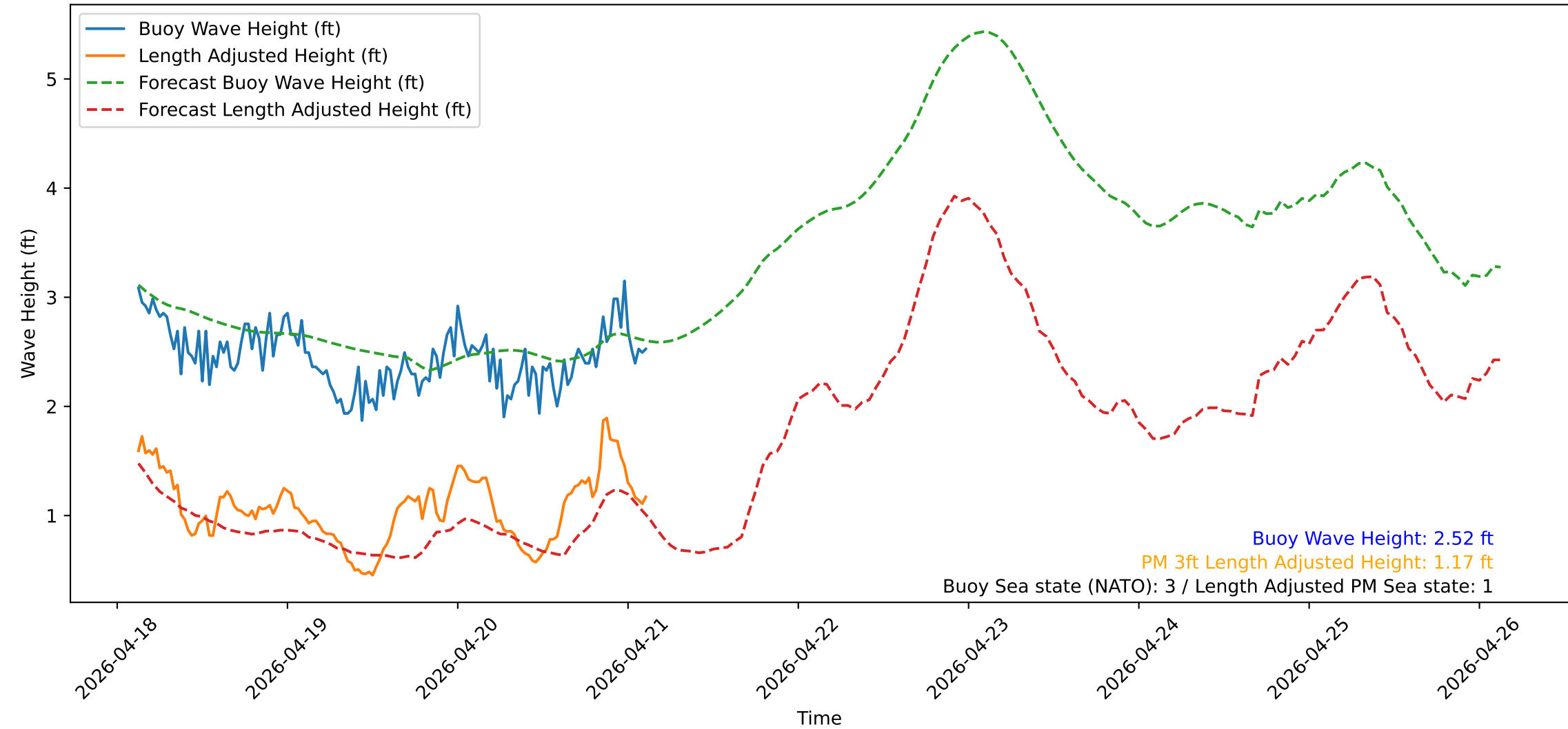
Wave Heights over Time for Green Beach at 2026-04-21 03:11:12
