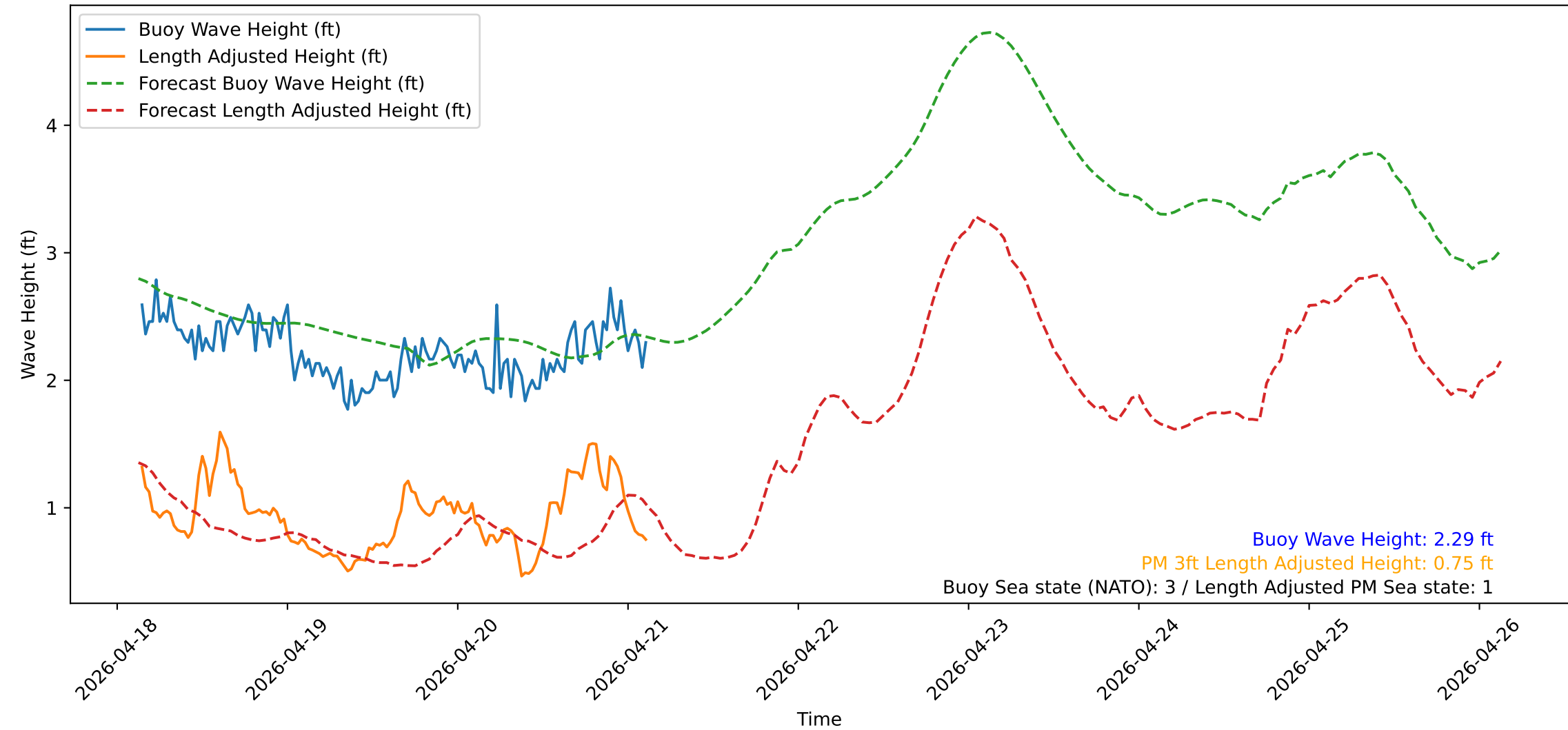
Wave Heights over Time for Red Beach at 2026-04-21 03:10:50
