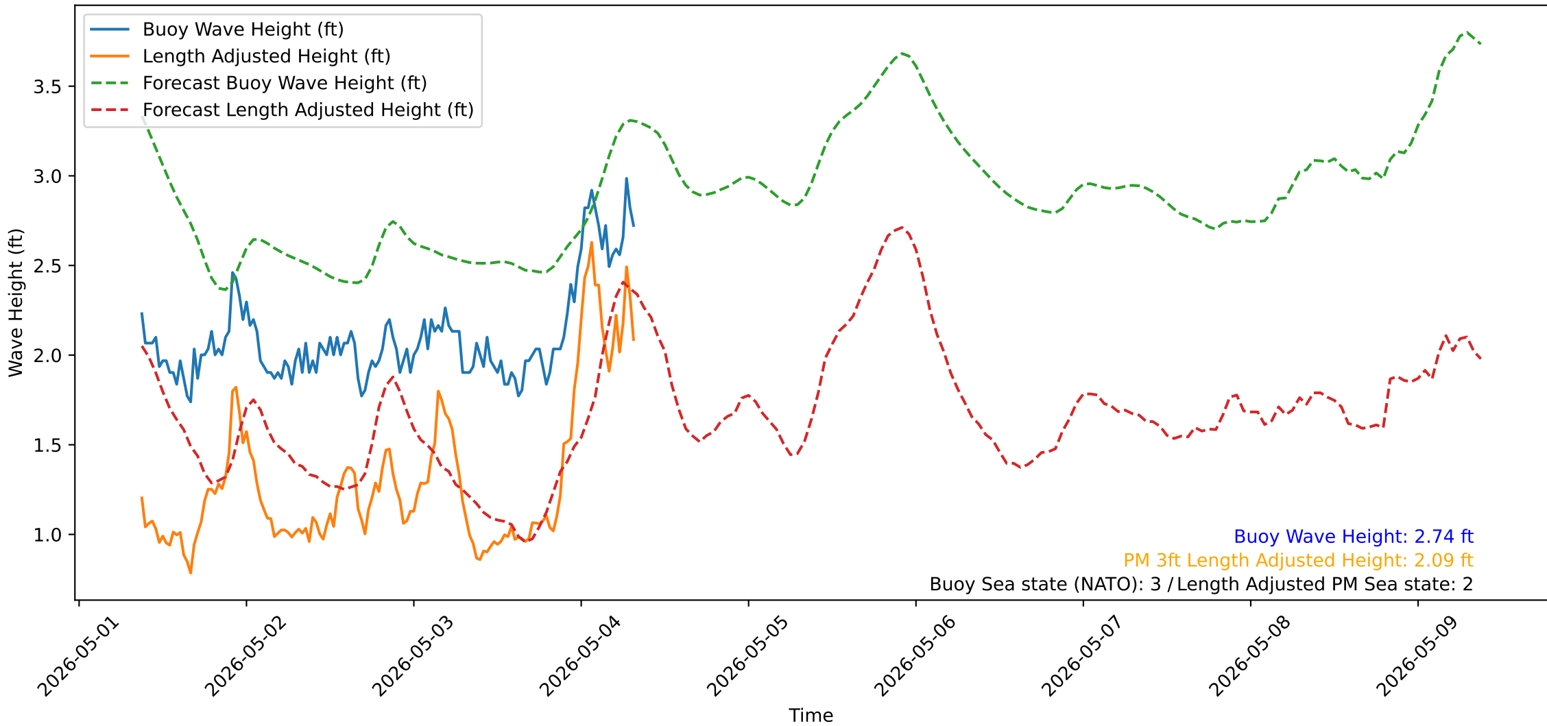
Wave Heights over Time for Green Beach at 2026-05-04 09:01:13
