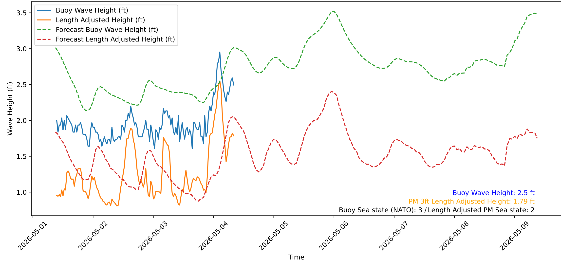
Wave Heights over Time for Red Beach at 2026-05-04 09:00:51
