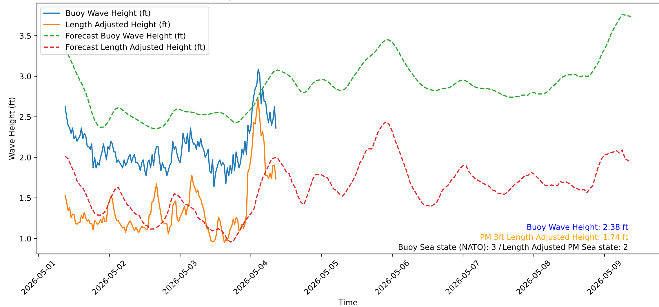
Wave Heights over Time for Oceanside Harbor at 2026-05-04 09:00:32
