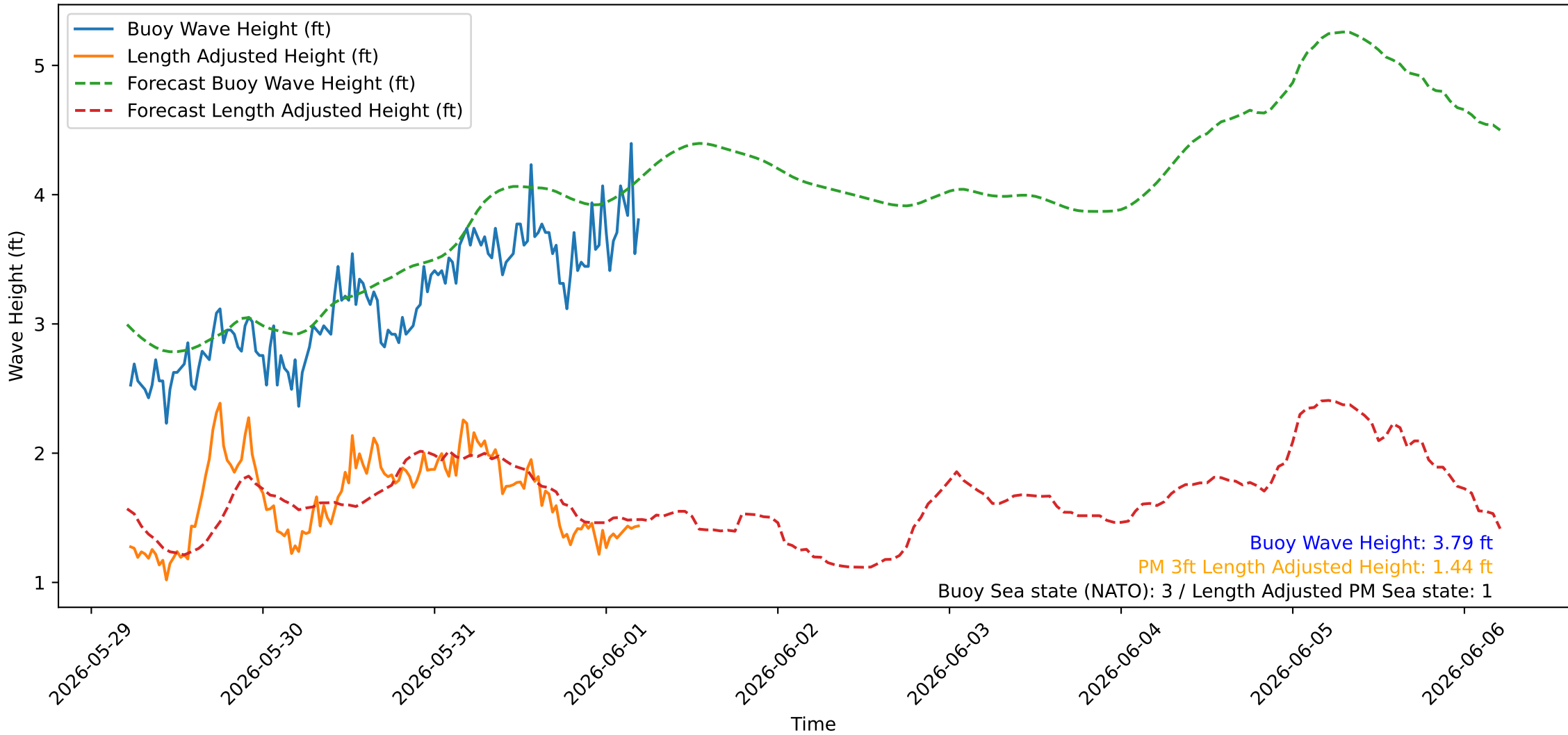
Wave Heights over Time for Oceanside Harbor at 2026-06-01 05:20:26
