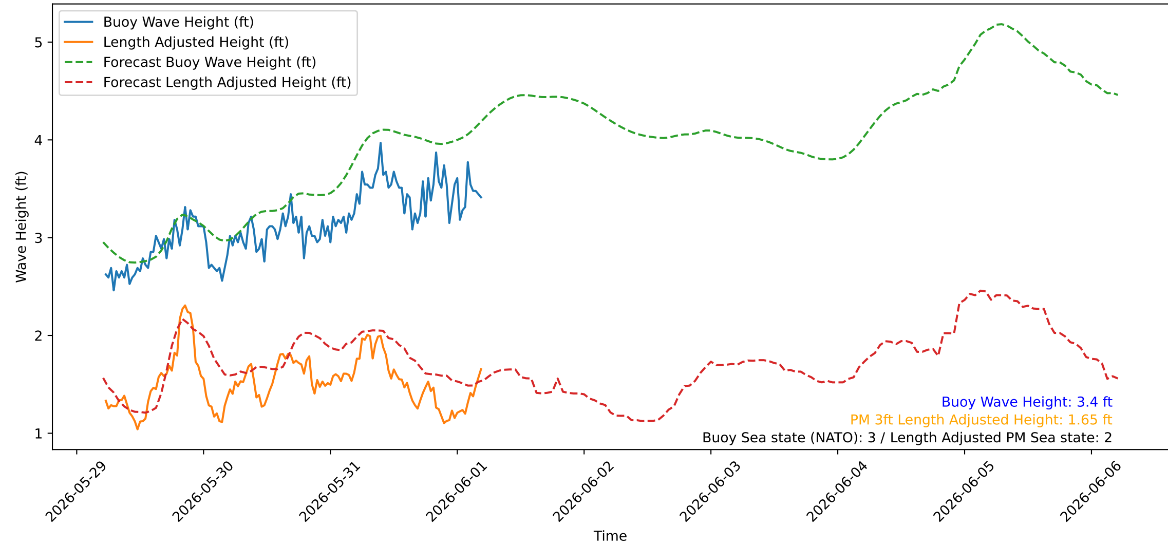
Wave Heights over Time for Green Beach at 2026-06-01 05:21:09
