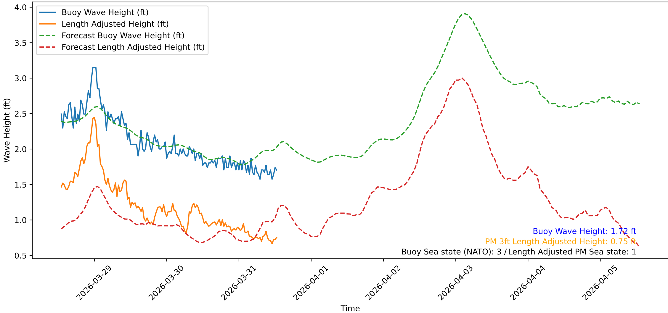
Wave Heights over Time for Oceanside Harbor at 2026-03-31 13:00:31
