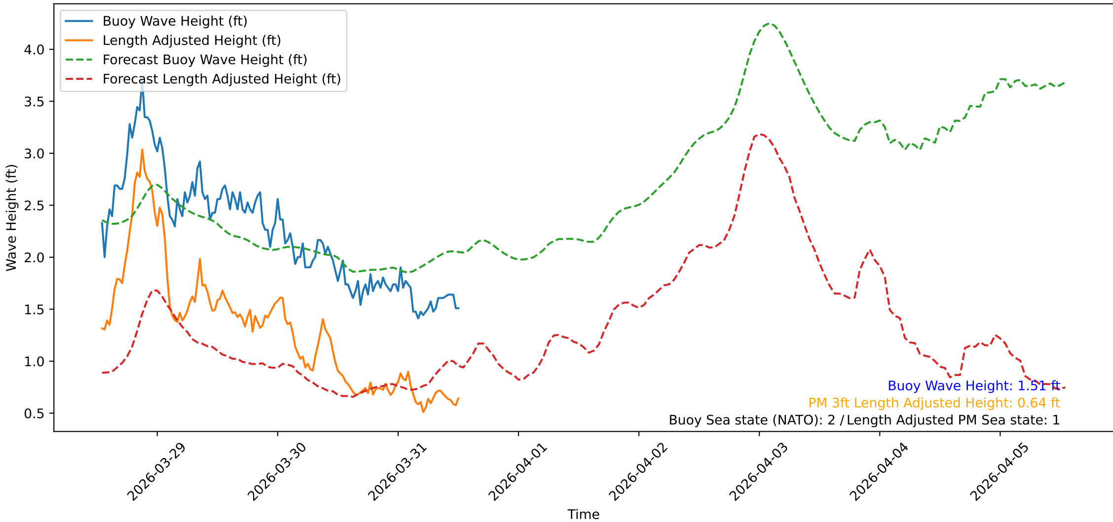
Wave Heights over Time for Green Beach at 2026-03-31 13:01:10
