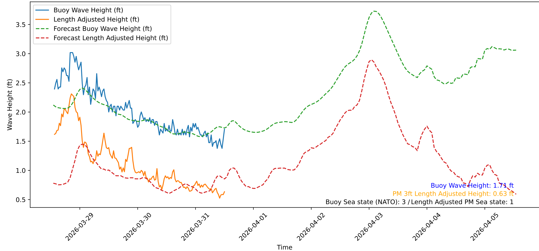
Wave Heights over Time for Red Beach at 2026-03-31 13:00:48
