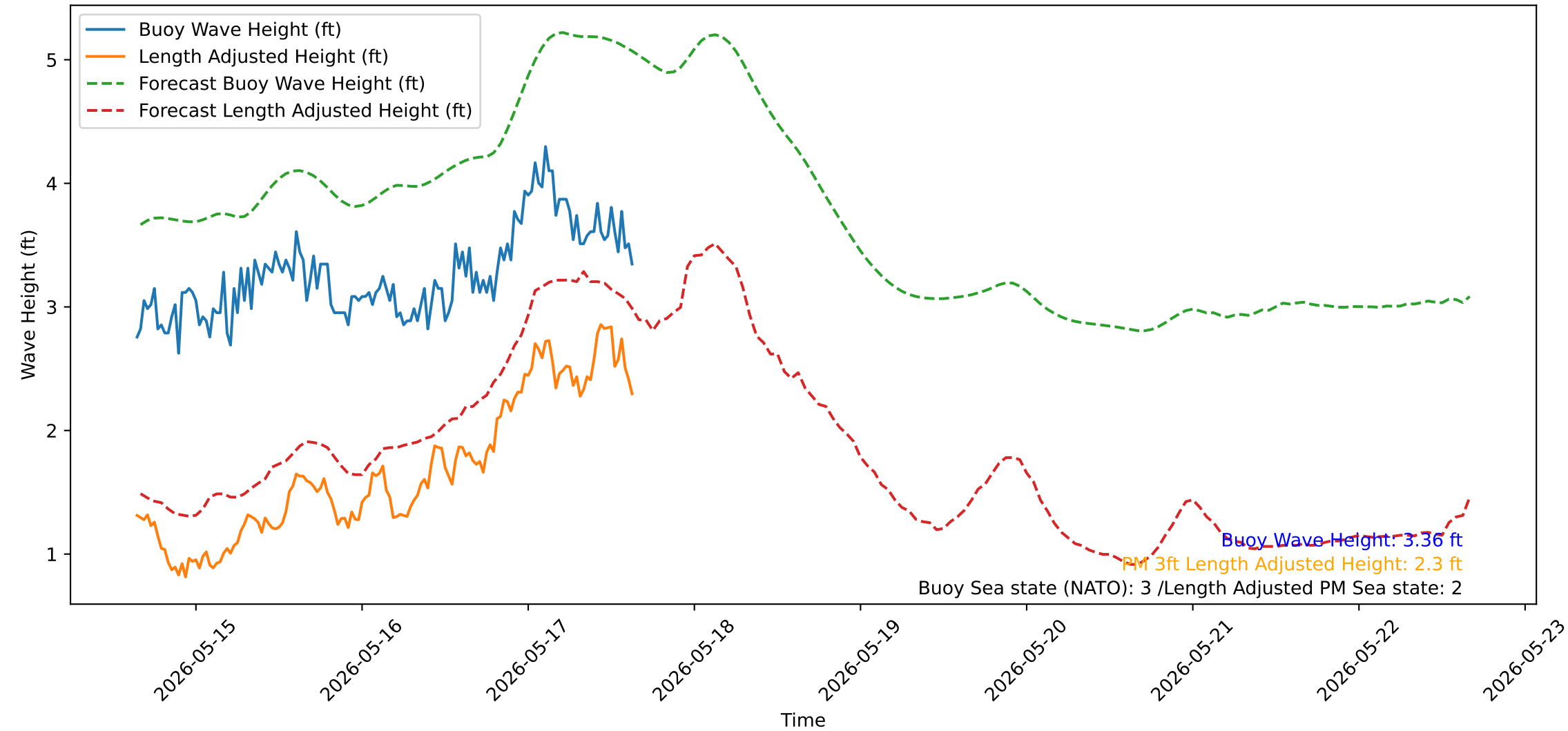
Wave Heights over Time for Oceanside Harbor at 2026-05-17 15:30:31
