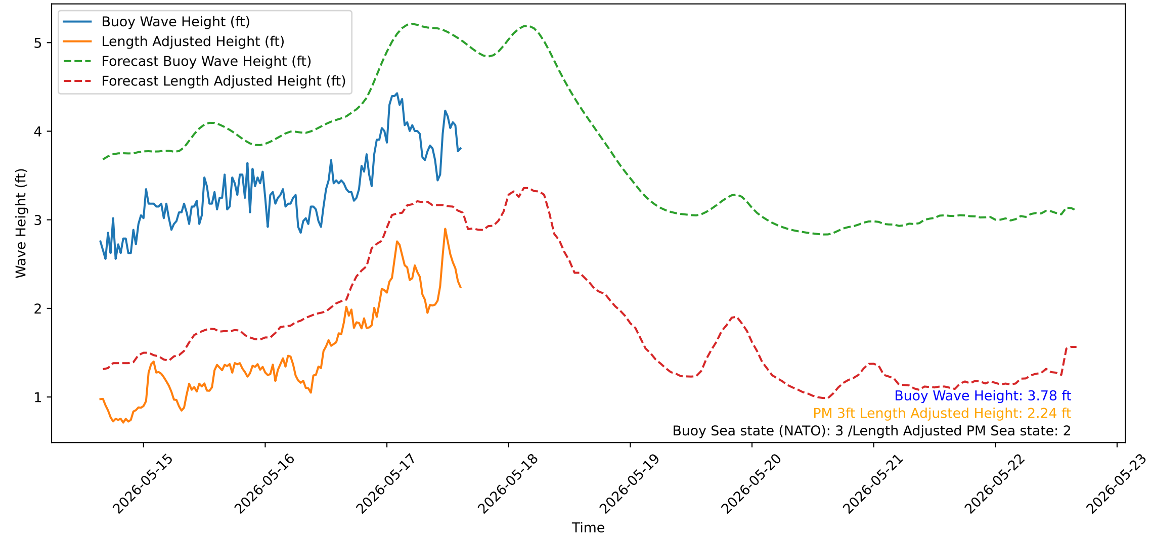
Wave Heights over Time for Green Beach at 2026-05-17 15:31:12
