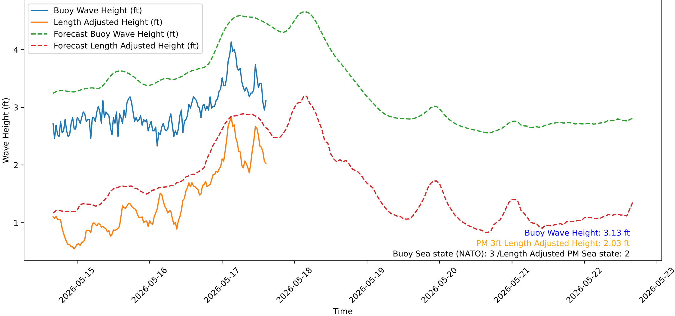
Wave Heights over Time for Red Beach at 2026-05-17 15:30:50
