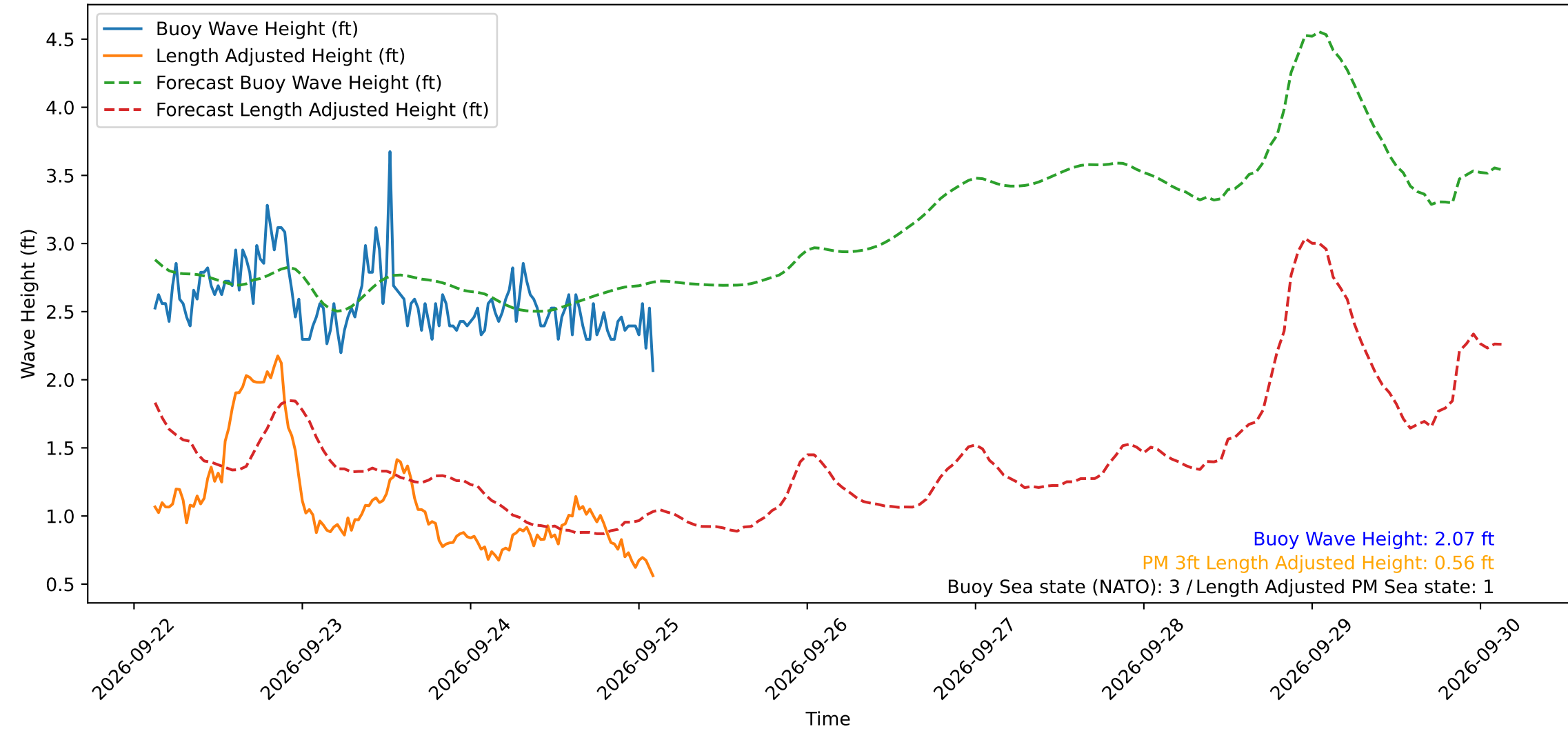
Wave Heights over Time for Red Beach at 2026-09-25 02:40:49
