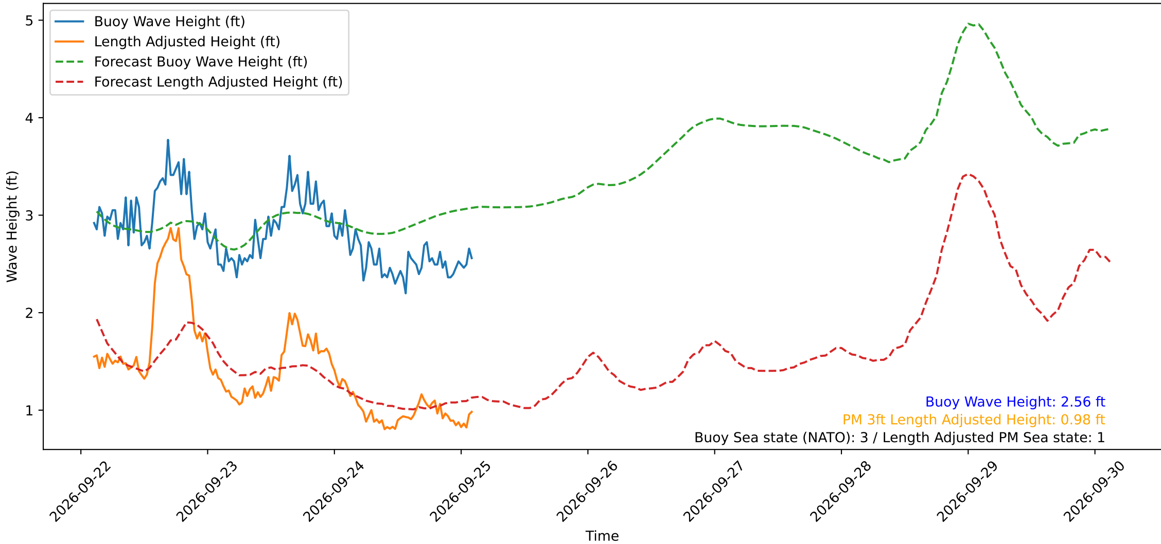
Wave Heights over Time for Oceanside Harbor at 2026-09-25 02:40:29
