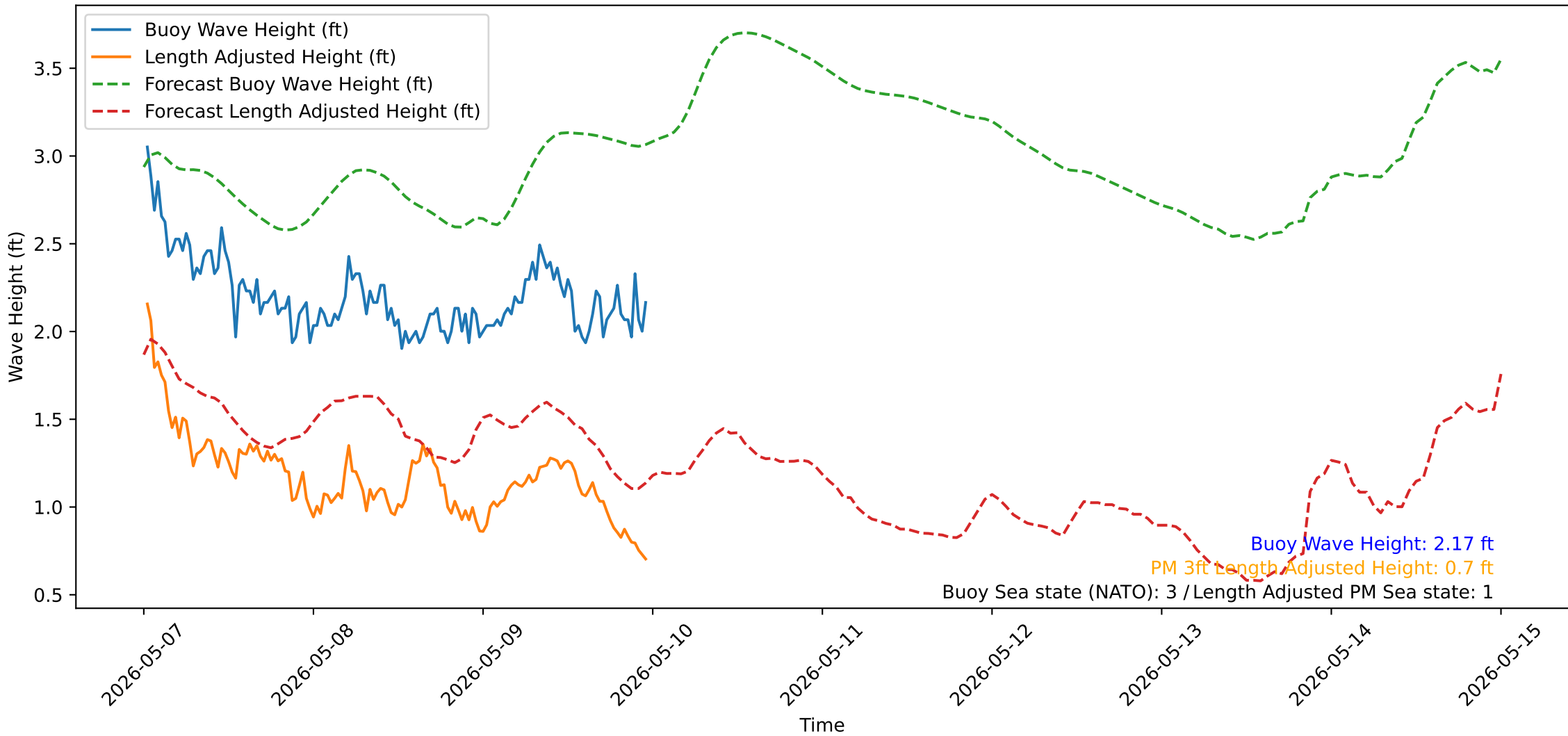
Wave Heights over Time for Red Beach at 2026-05-10 00:00:51
