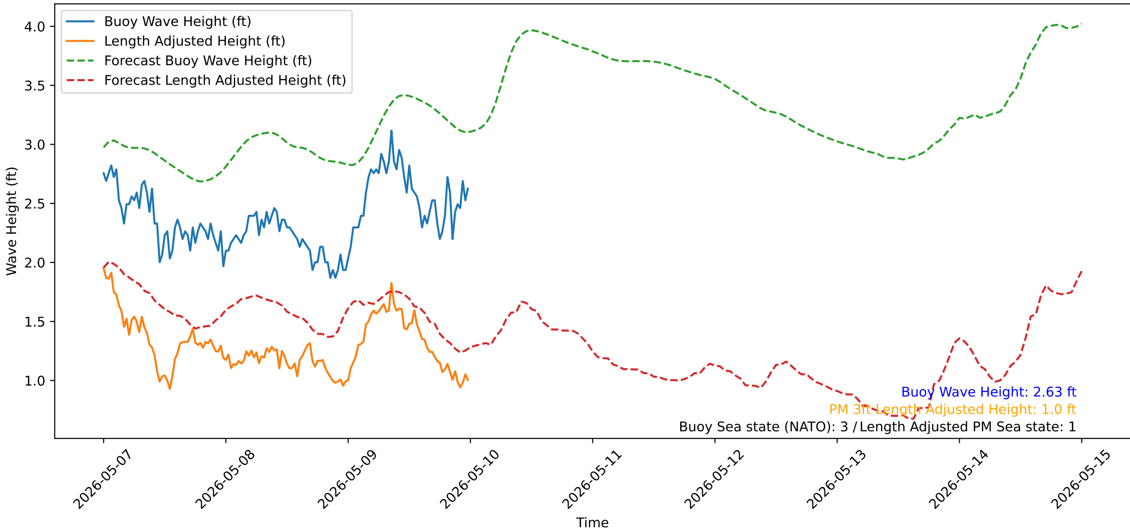
Wave Heights over Time for Oceanside Harbor at 2026-05-10 00:00:32
