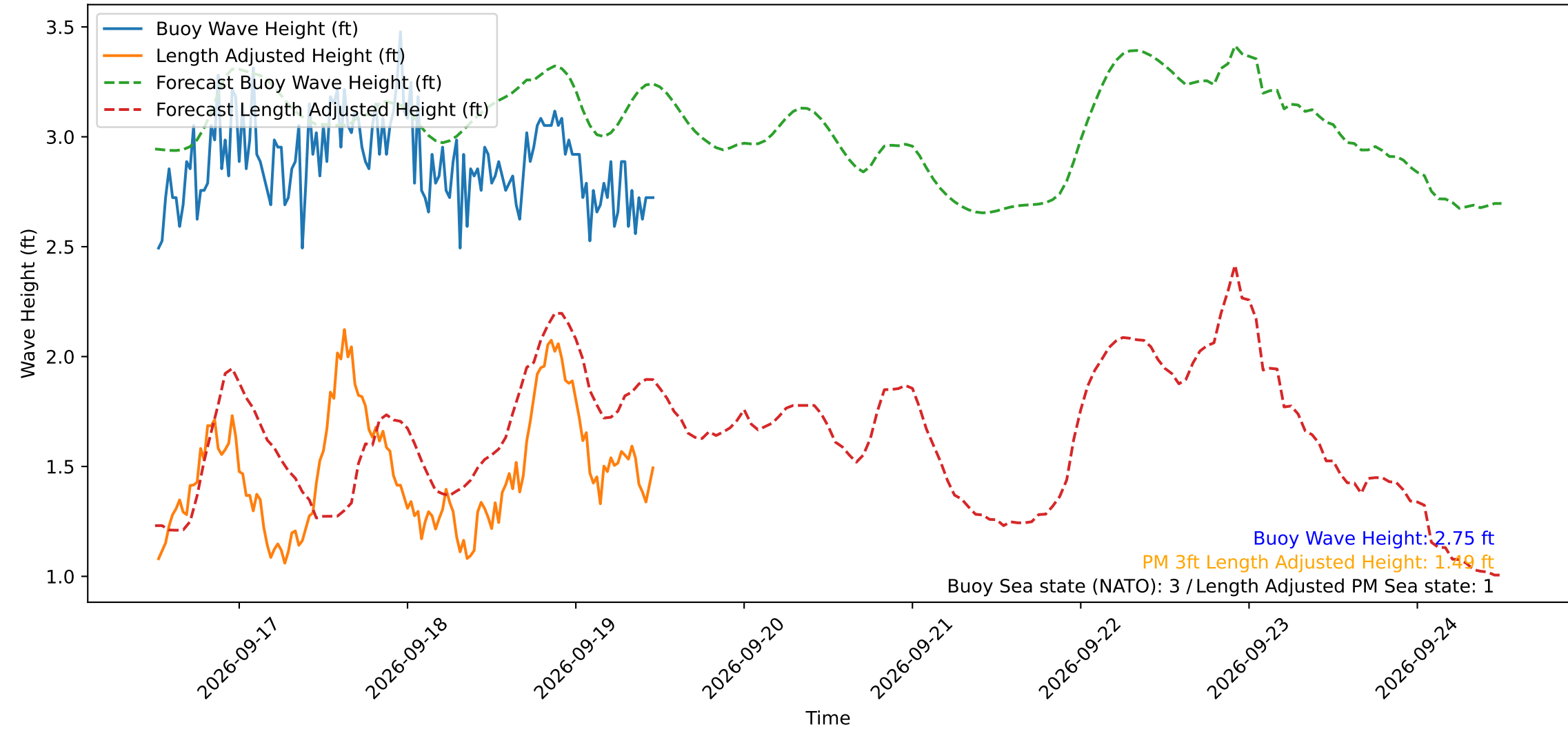
Wave Heights over Time for Green Beach at 2026-09-19 12:01:12
