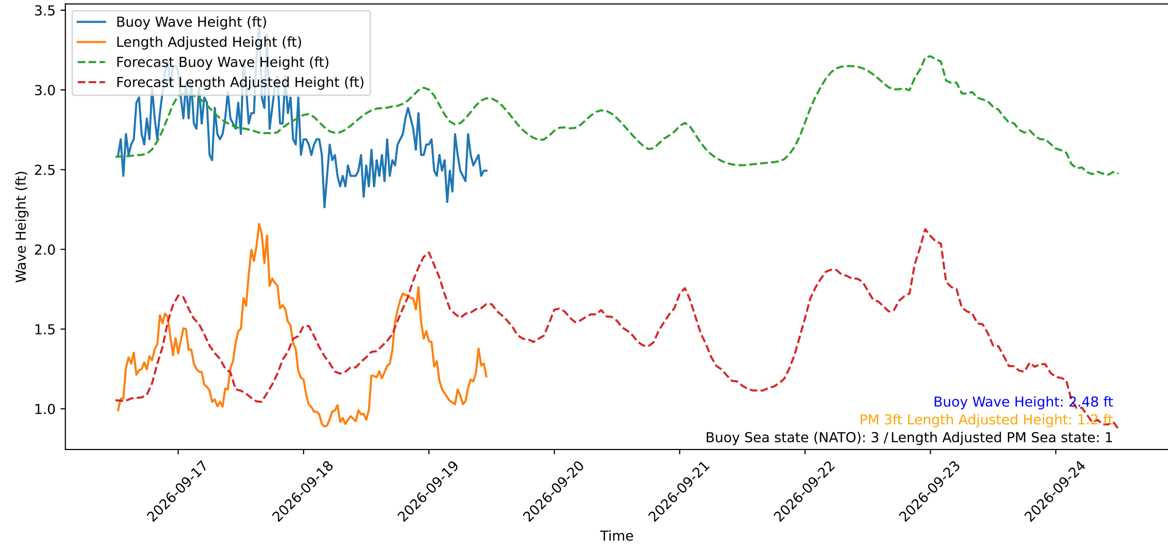
Wave Heights over Time for Red Beach at 2026-09-19 12:00:50
