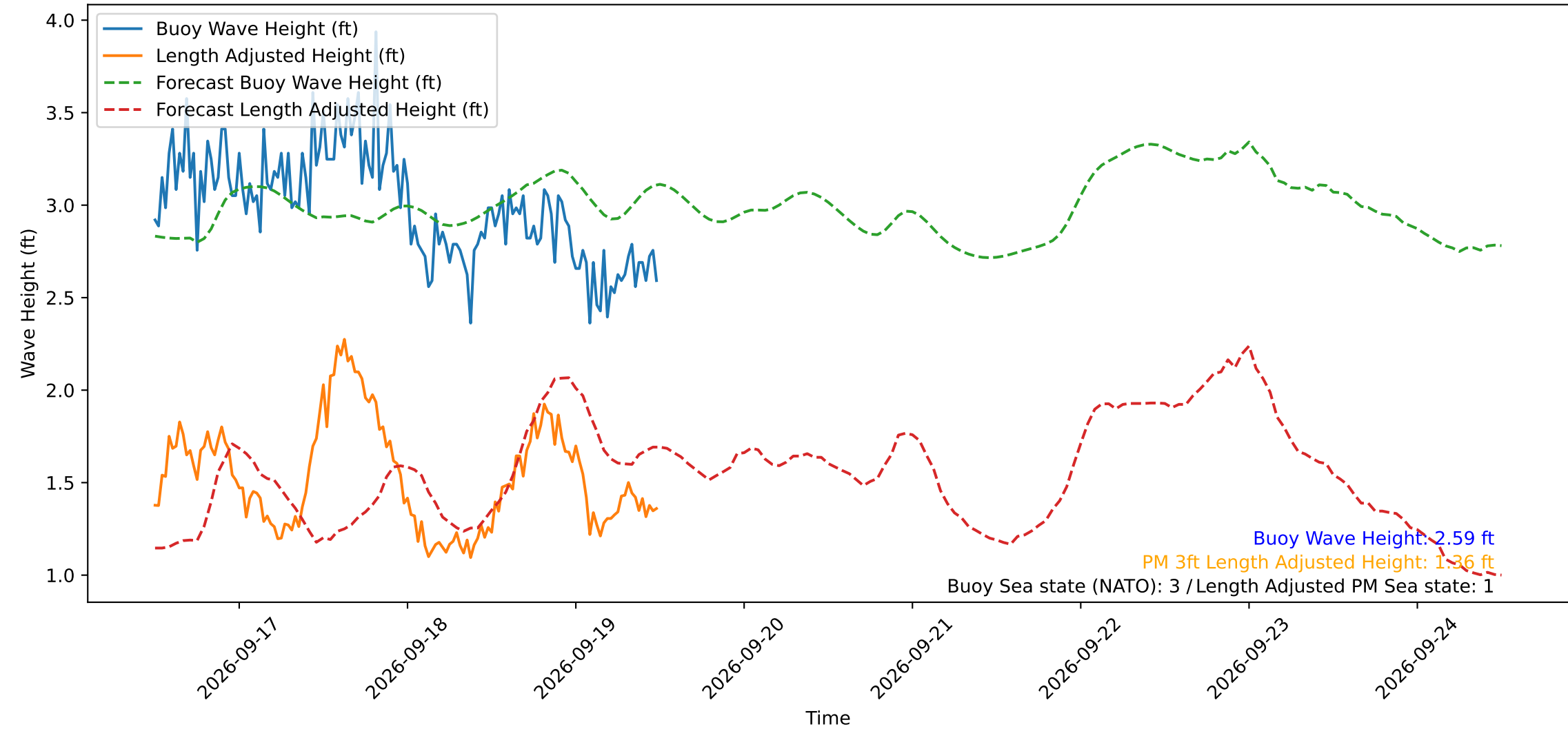
Wave Heights over Time for Oceanside Harbor at 2026-09-19 12:00:30
