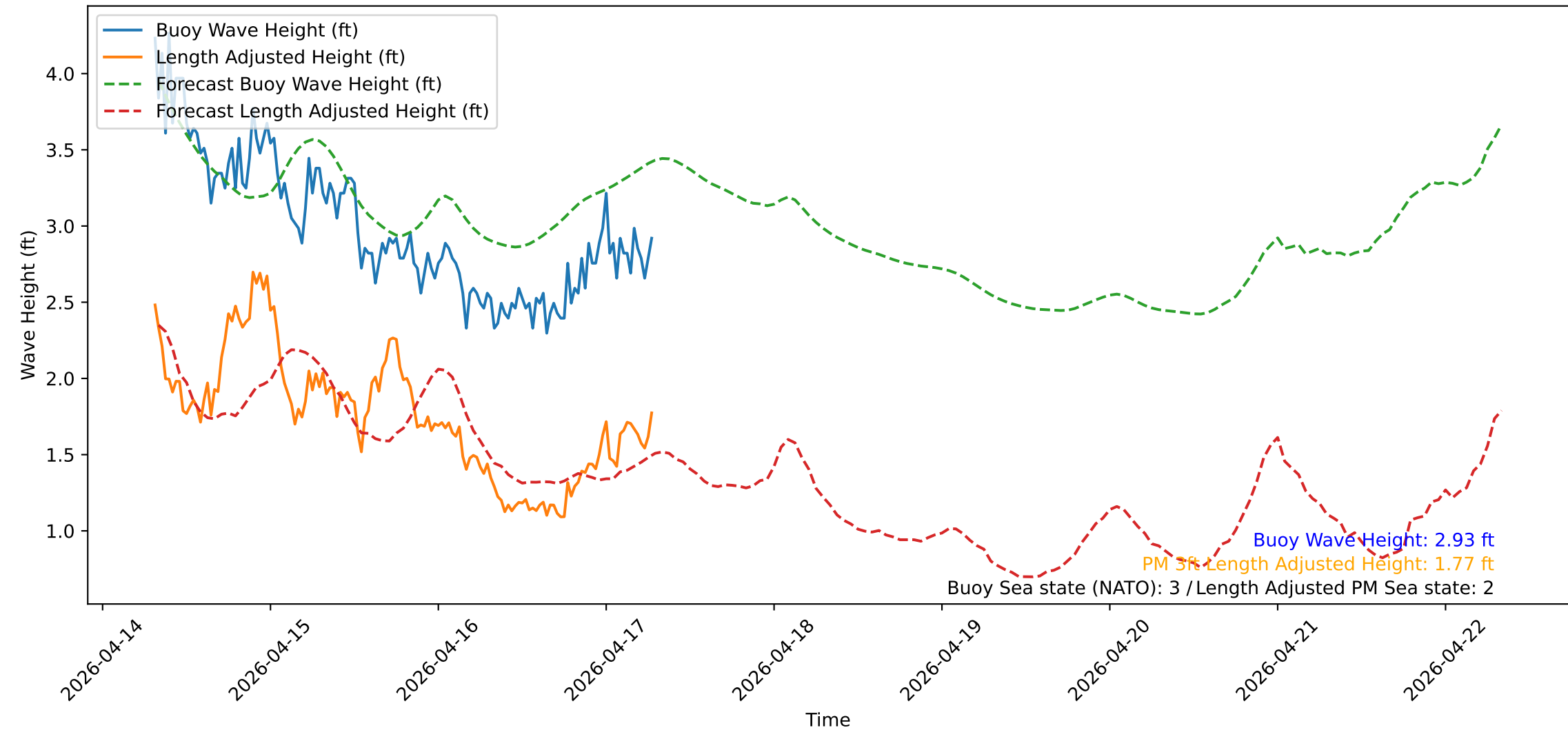
Wave Heights over Time for Oceanside Harbor at 2026-04-17 07:30:32
