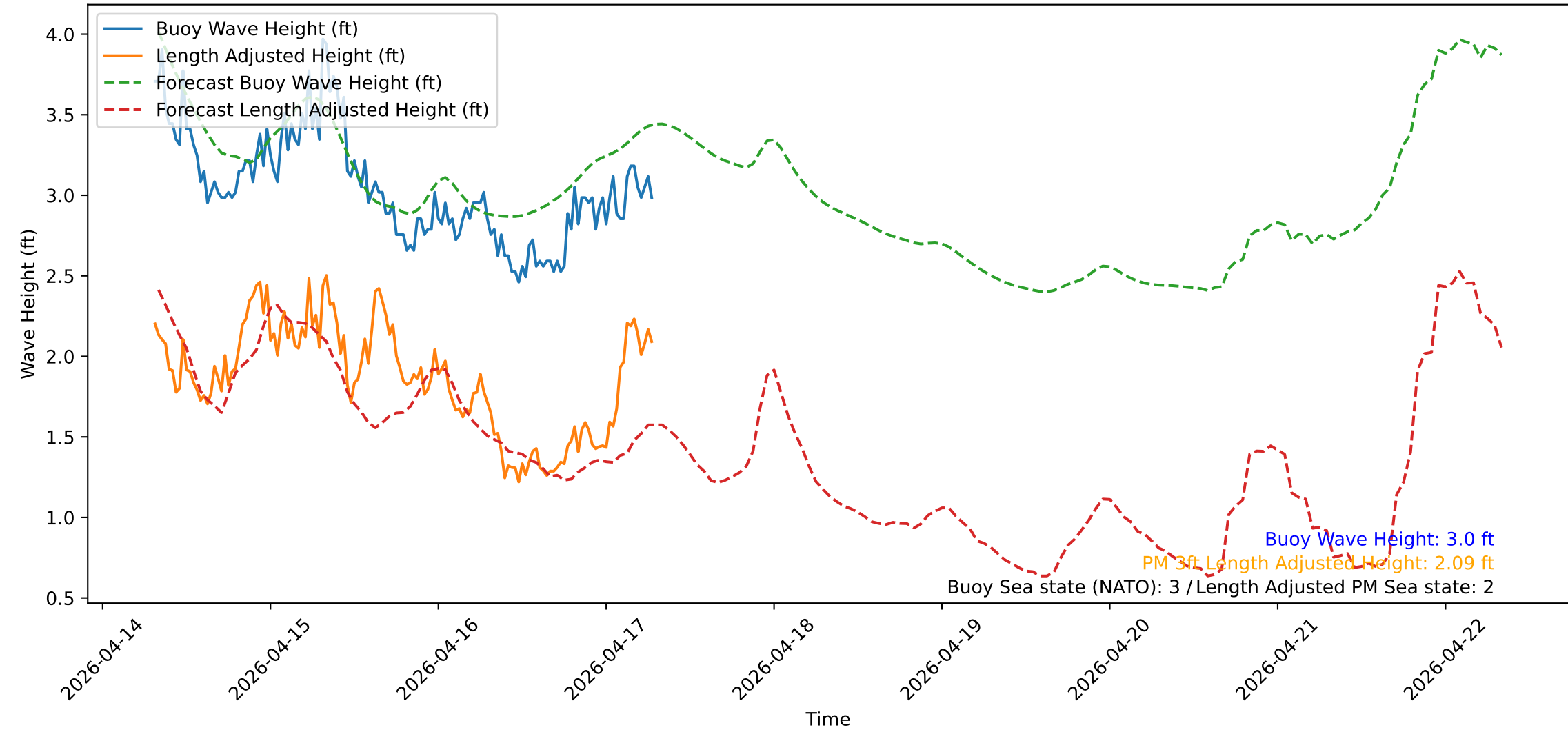
Wave Heights over Time for Green Beach at 2026-04-17 07:31:14
