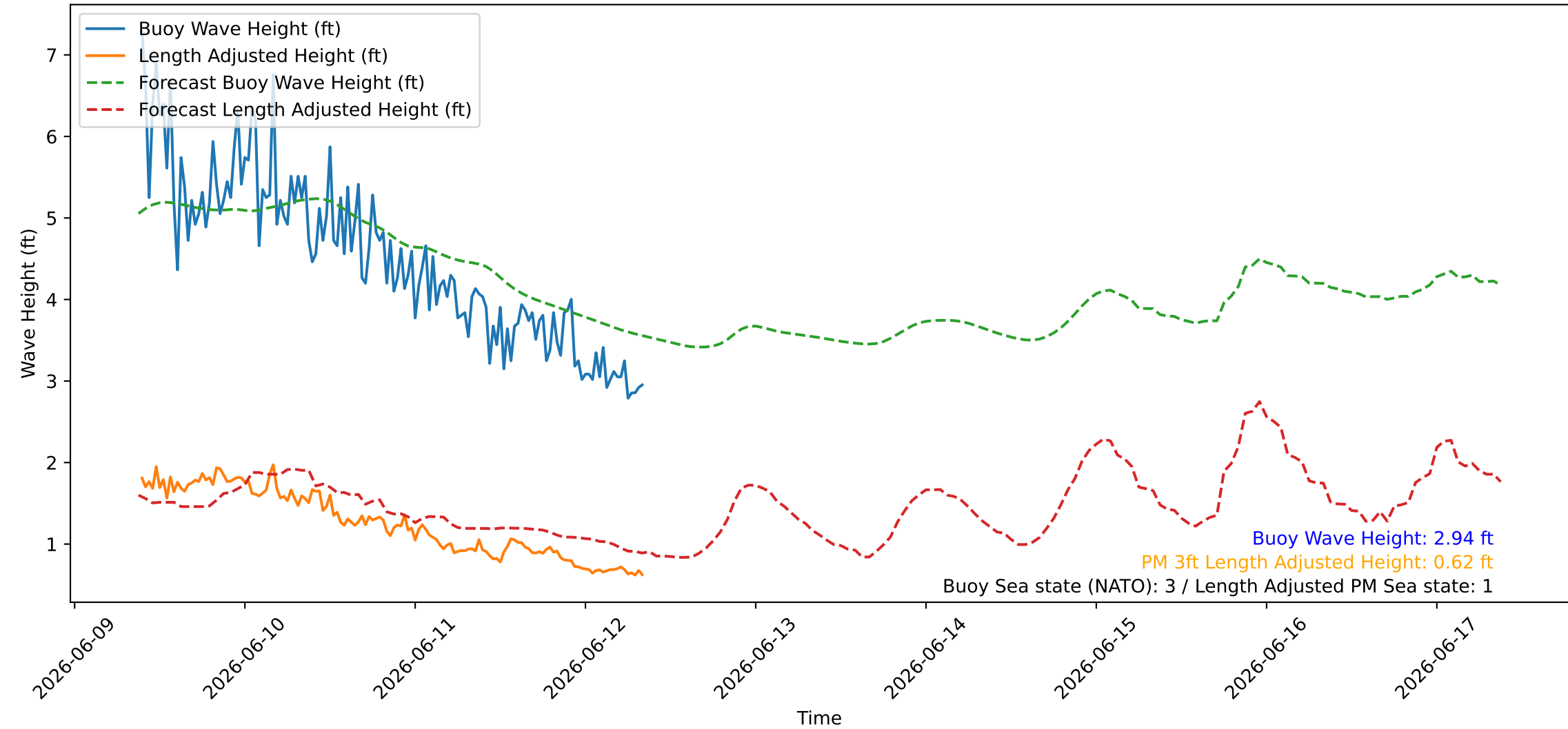
Wave Heights over Time for Red Beach at 2026-06-12 09:00:47
