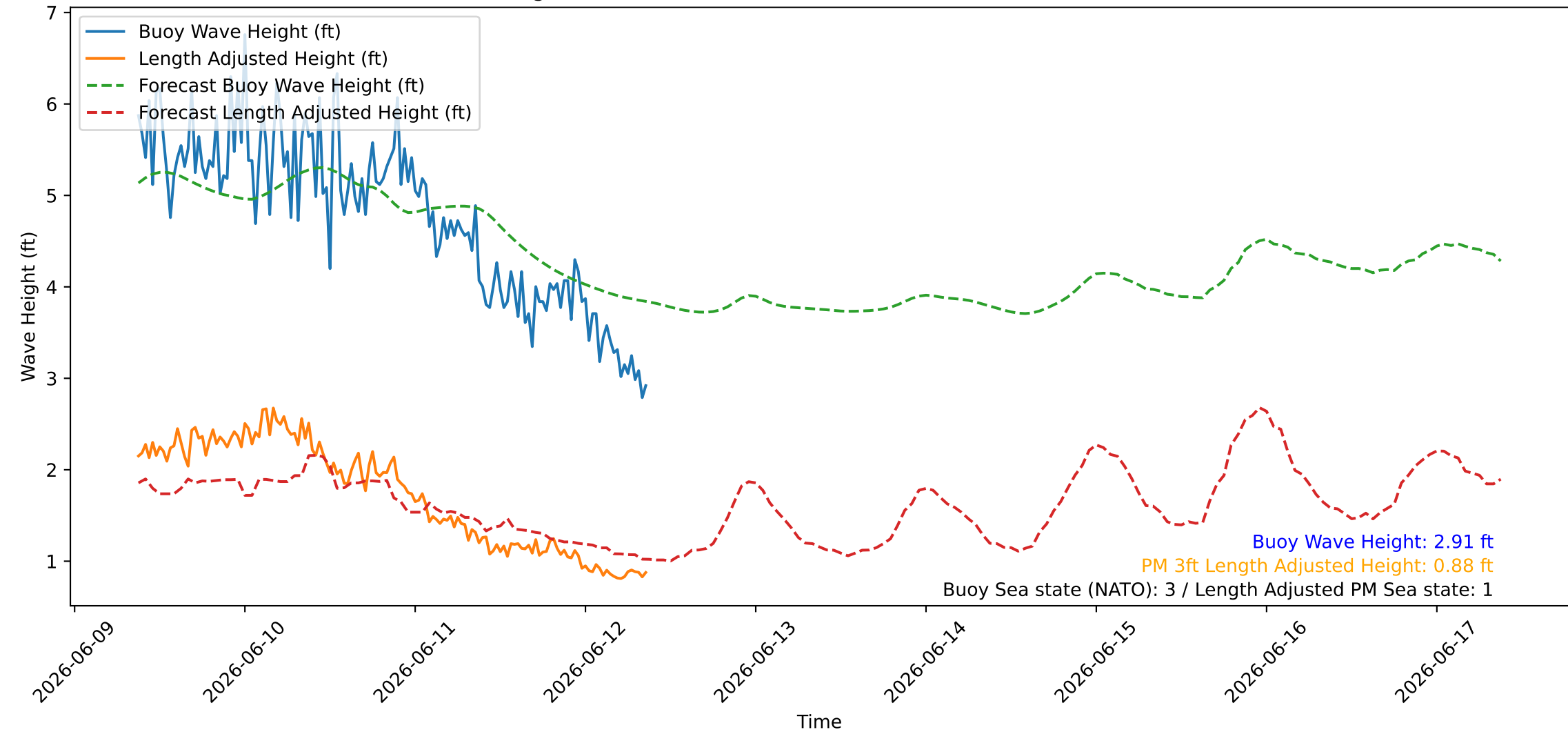
Wave Heights over Time for Oceanside Harbor at 2026-06-12 09:00:26
