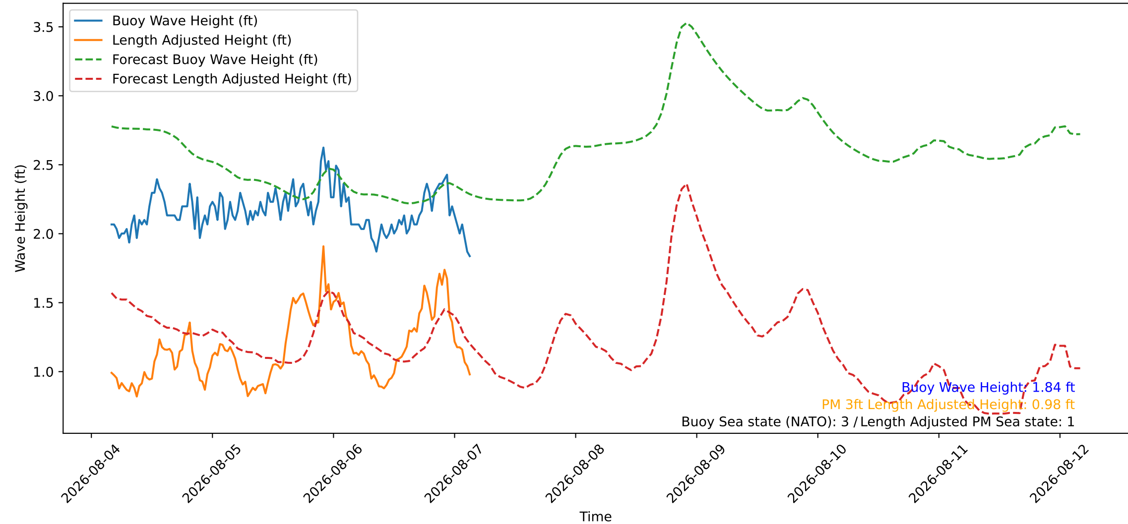
Wave Heights over Time for Green Beach at 2026-08-07 04:01:07
