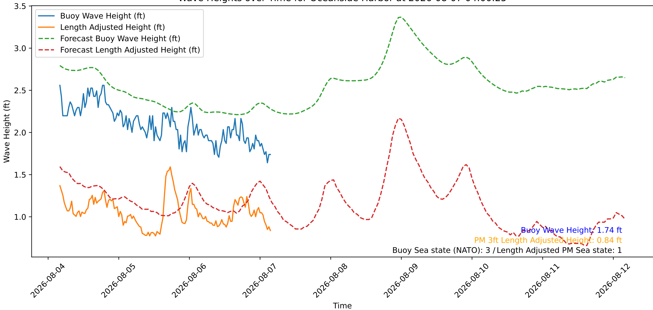
Wave Heights over Time for Oceanside Harbor at 2026-08-07 04:00:25
