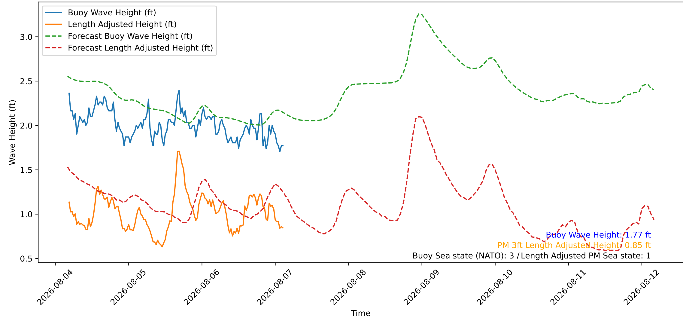
Wave Heights over Time for Red Beach at 2026-08-07 04:00:44
