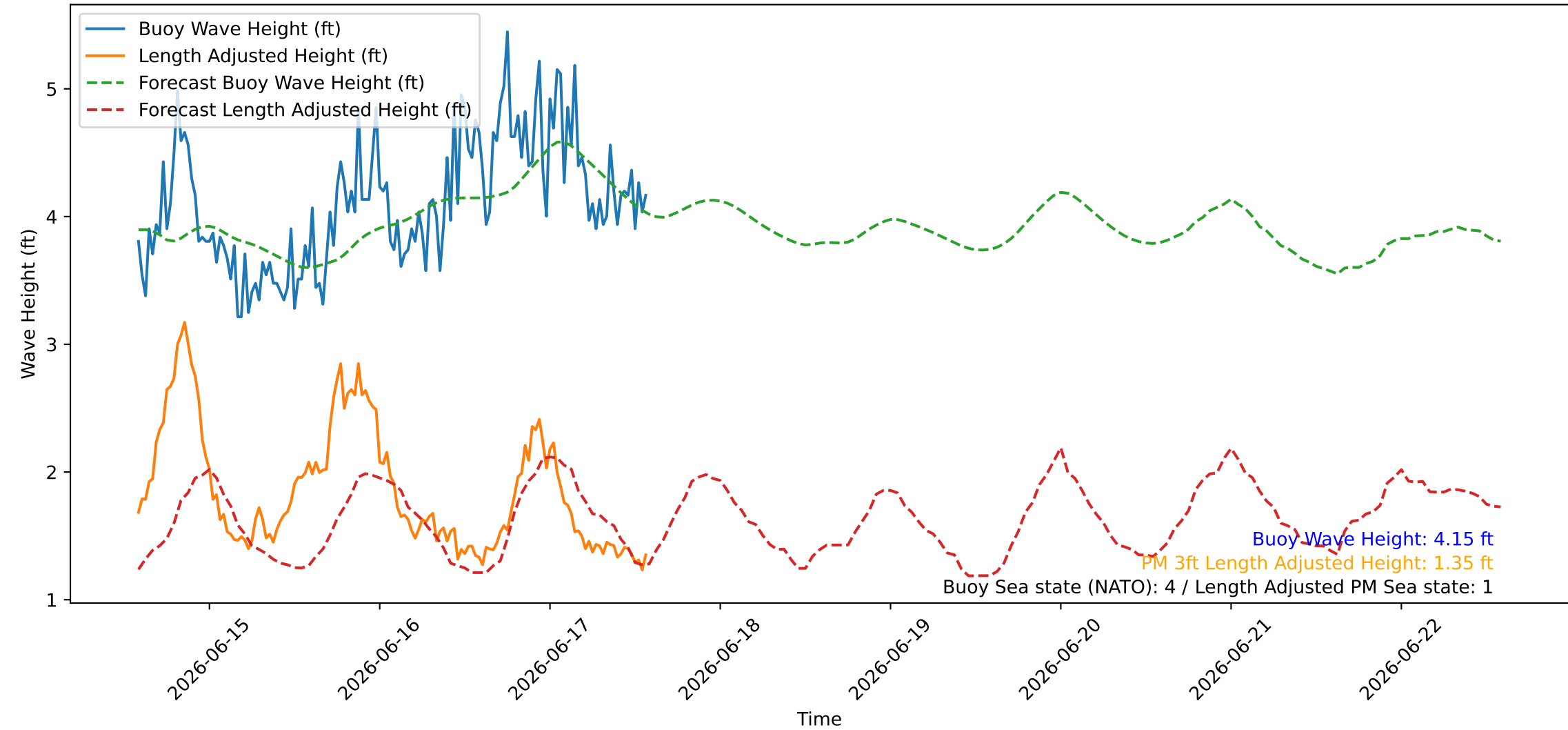
Wave Heights over Time for Oceanside Harbor at 2026-06-17 14:00:26
