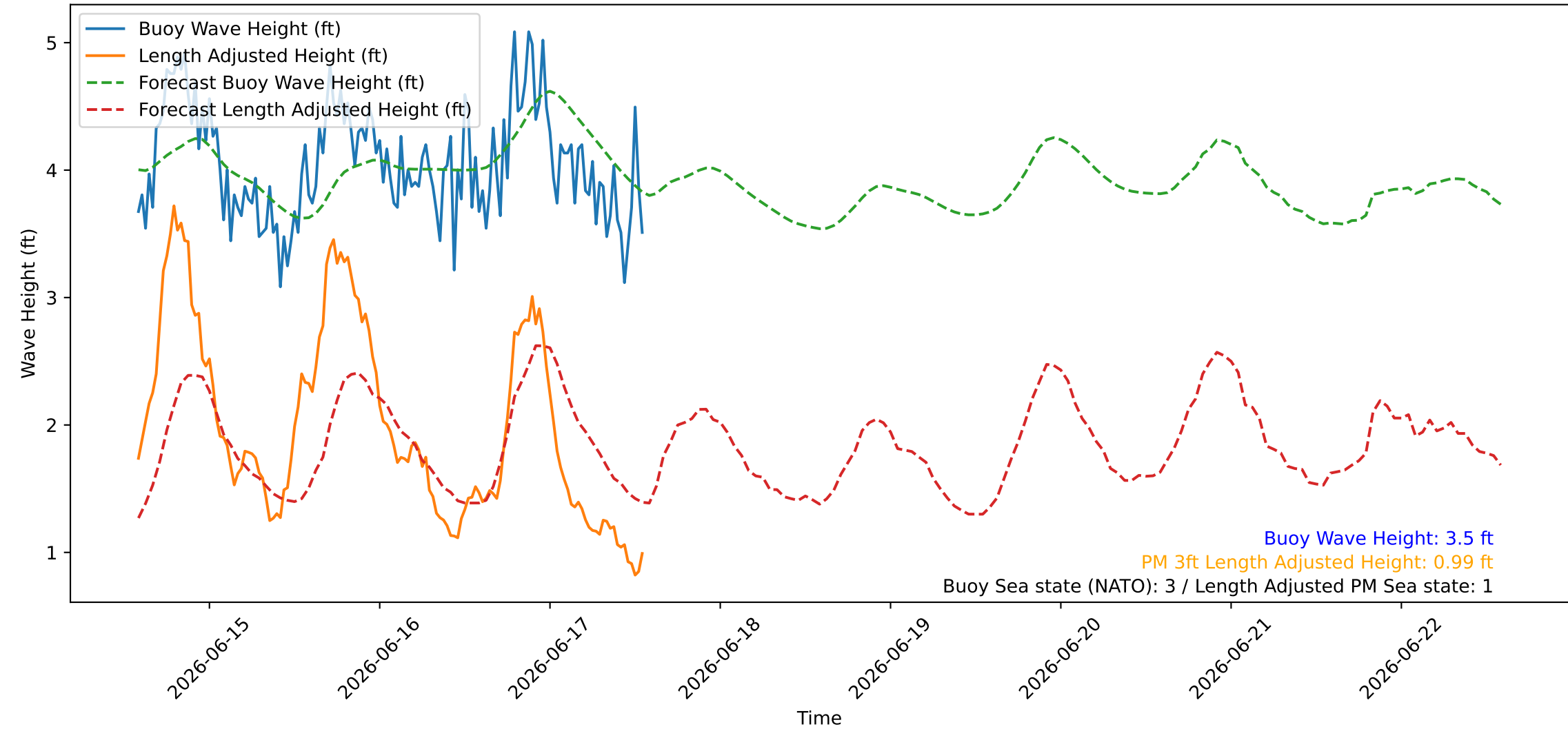
Wave Heights over Time for Green Beach at 2026-06-17 14:01:07
