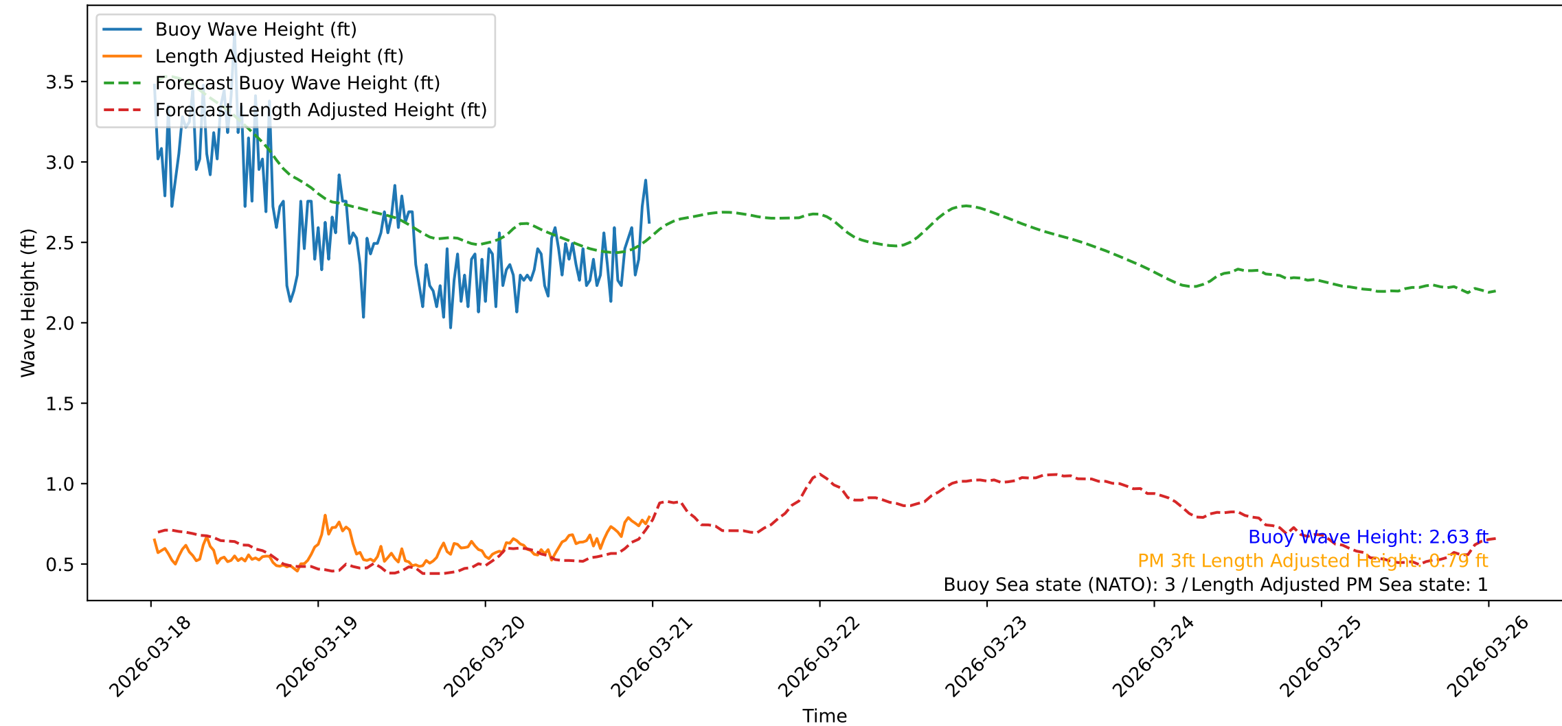
Wave Heights over Time for Oceanside Harbor at 2026-03-21 00:30:31
