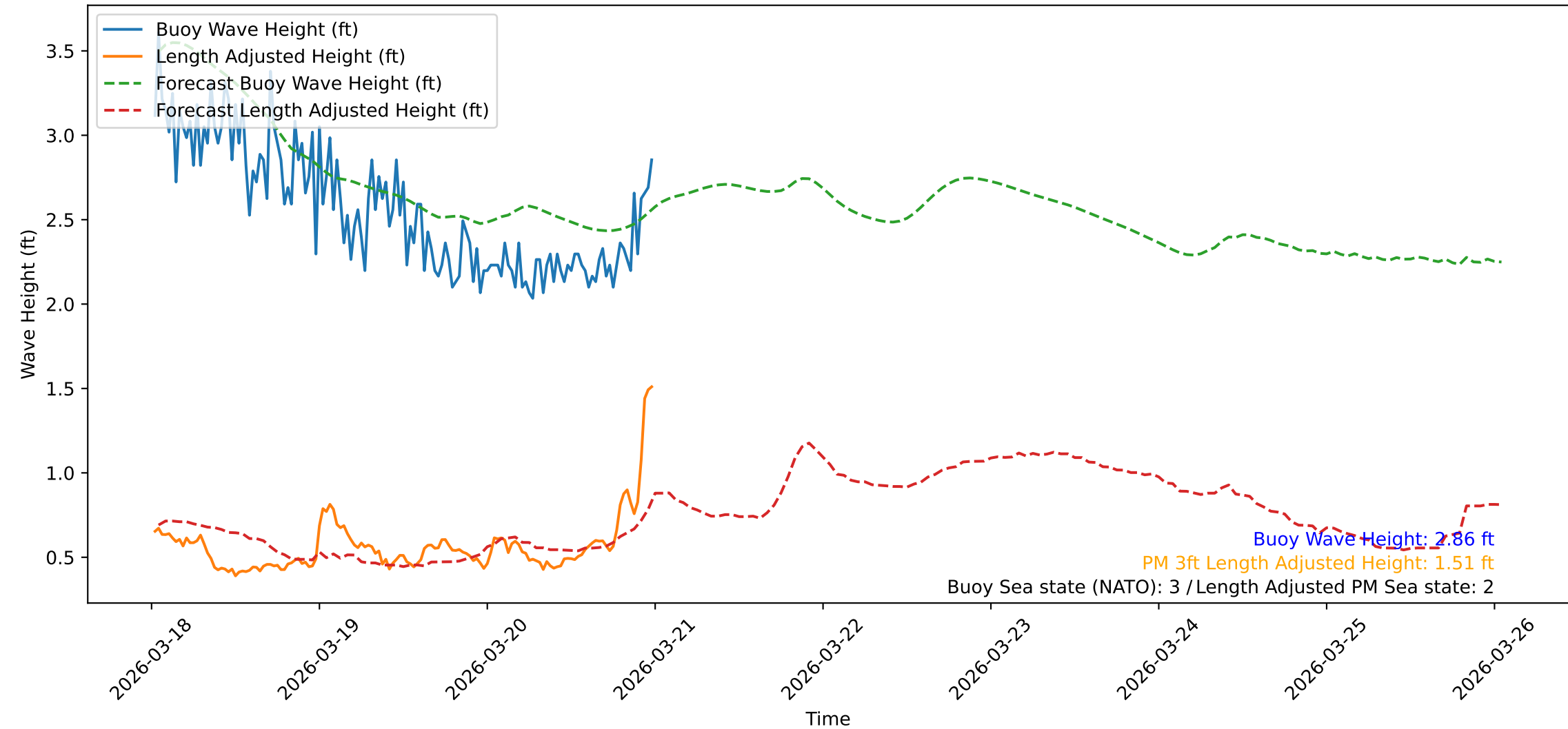
Wave Heights over Time for Green Beach at 2026-03-21 00:31:10
