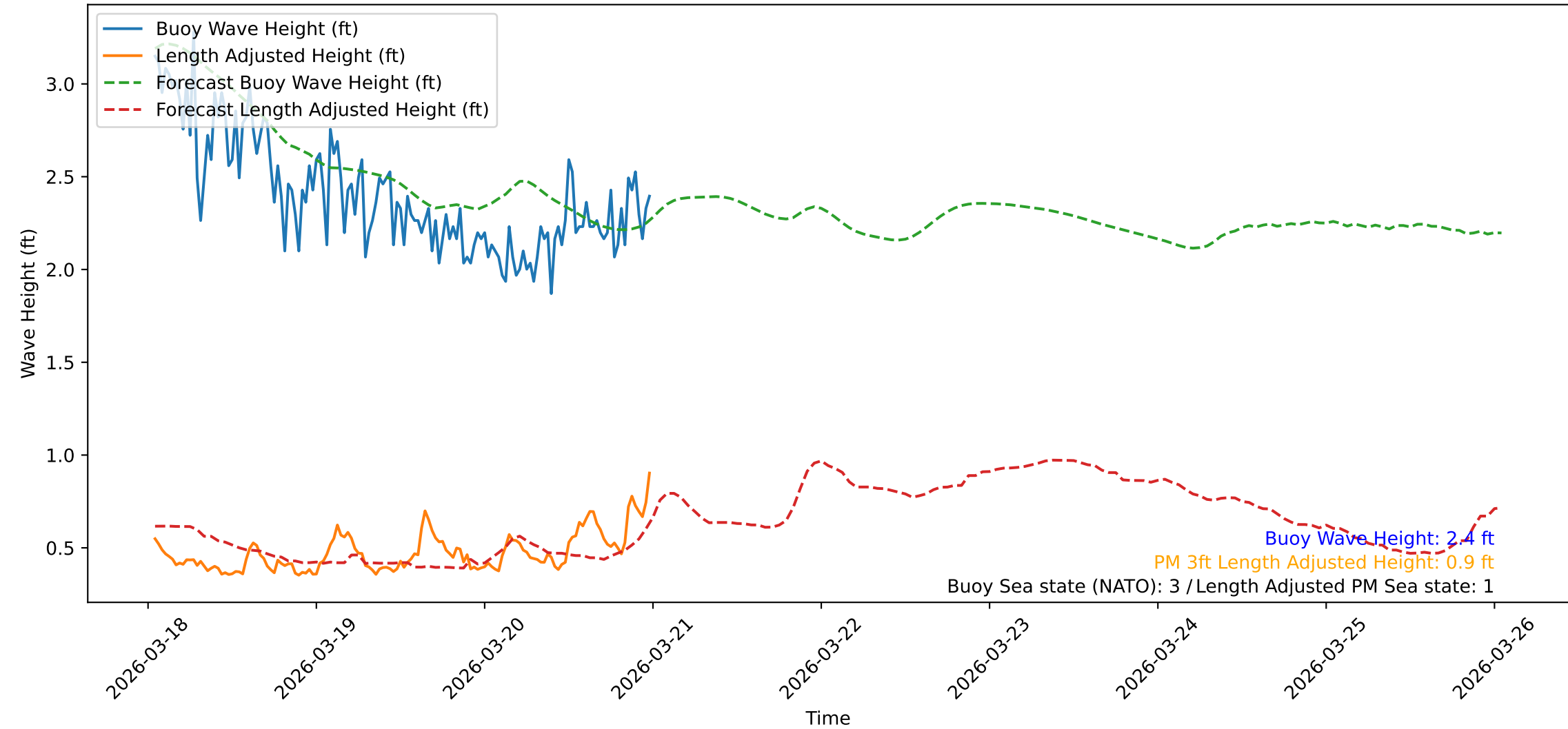
Wave Heights over Time for Red Beach at 2026-03-21 00:30:47
