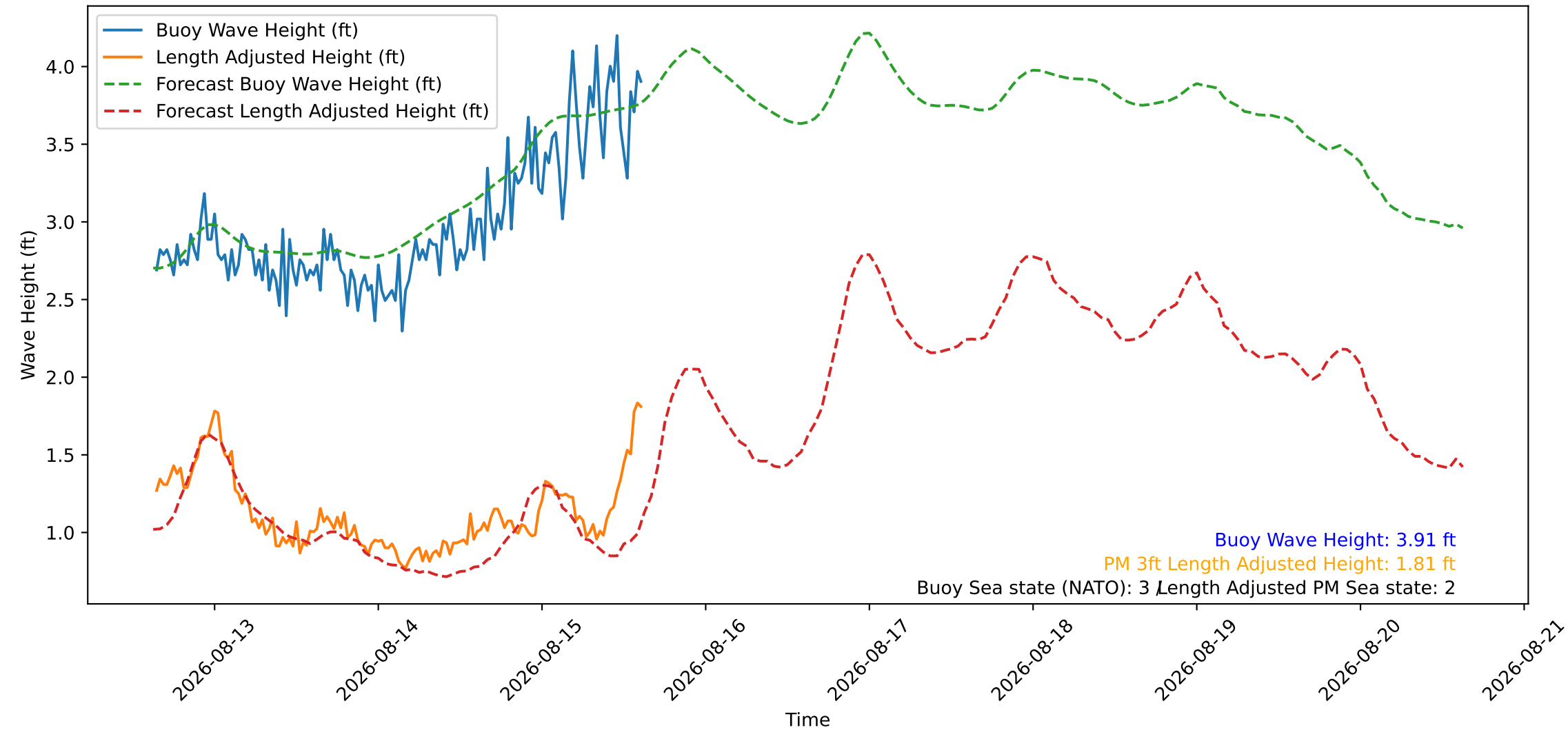
Wave Heights over Time for Oceanside Harbor at 2026-08-15 15:20:26
