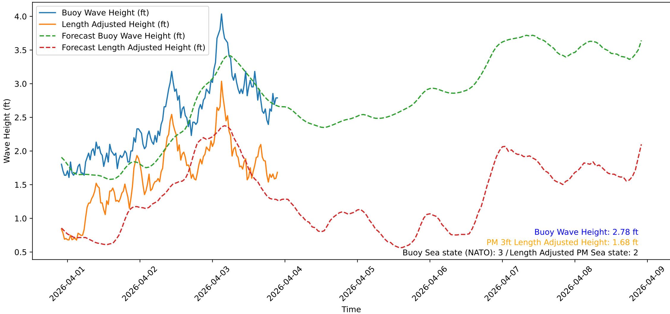
Wave Heights over Time for Oceanside Harbor at 2026-04-03 22:10:39
