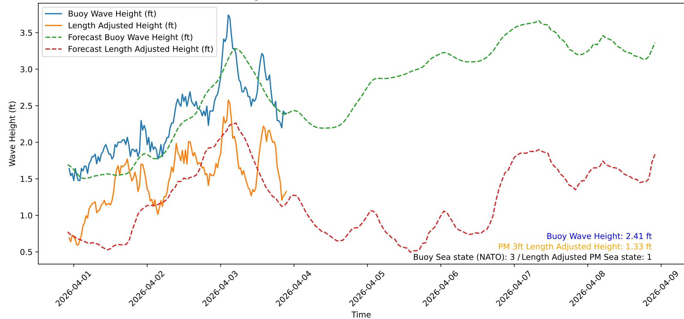
Wave Heights over Time for Red Beach at 2026-04-03 22:11:00
