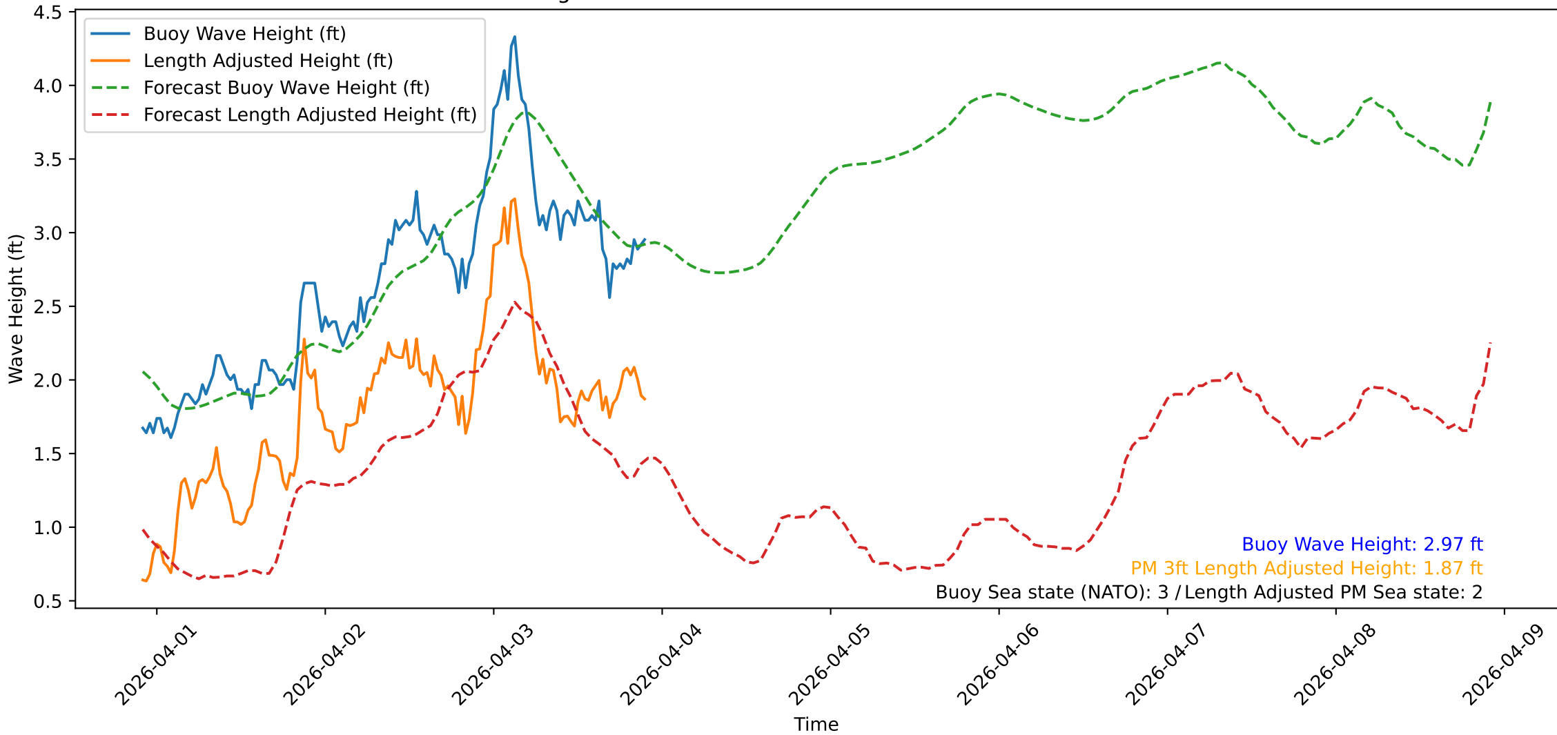
Wave Heights over Time for Green Beach at 2026-04-03 22:11:29
