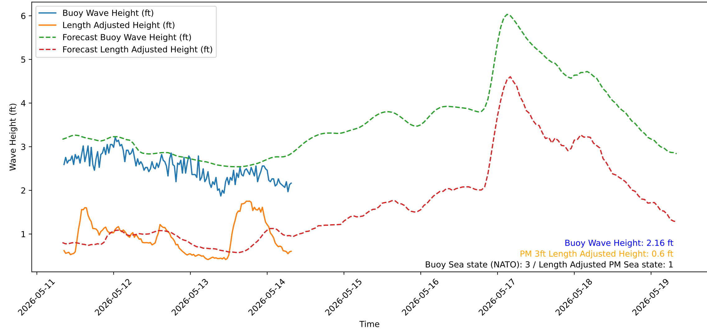
Wave Heights over Time for Red Beach at 2026-05-14 08:20:53
