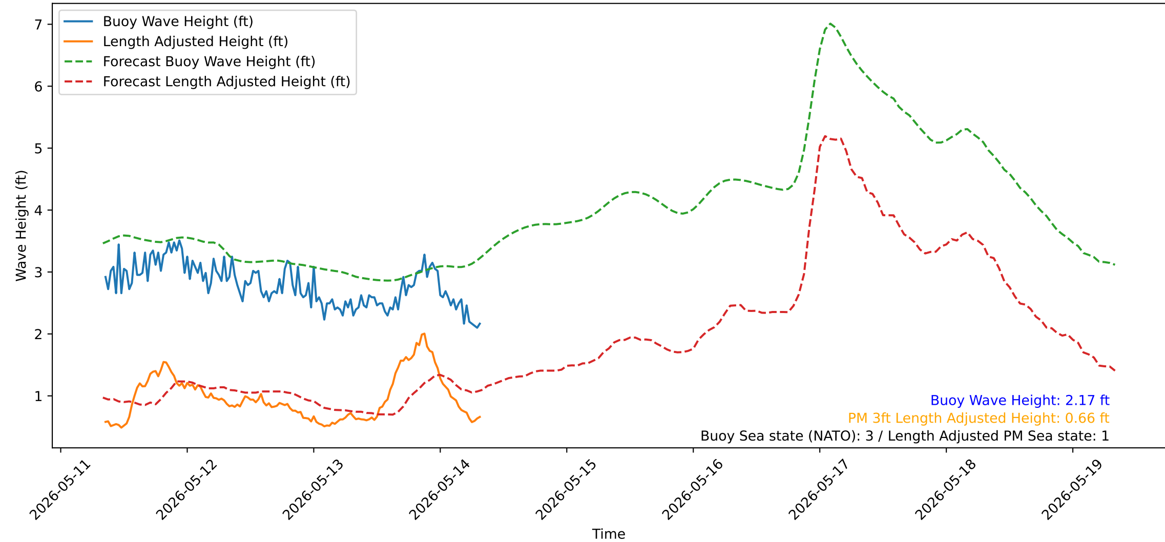
Wave Heights over Time for Green Beach at 2026-05-14 08:21:16
