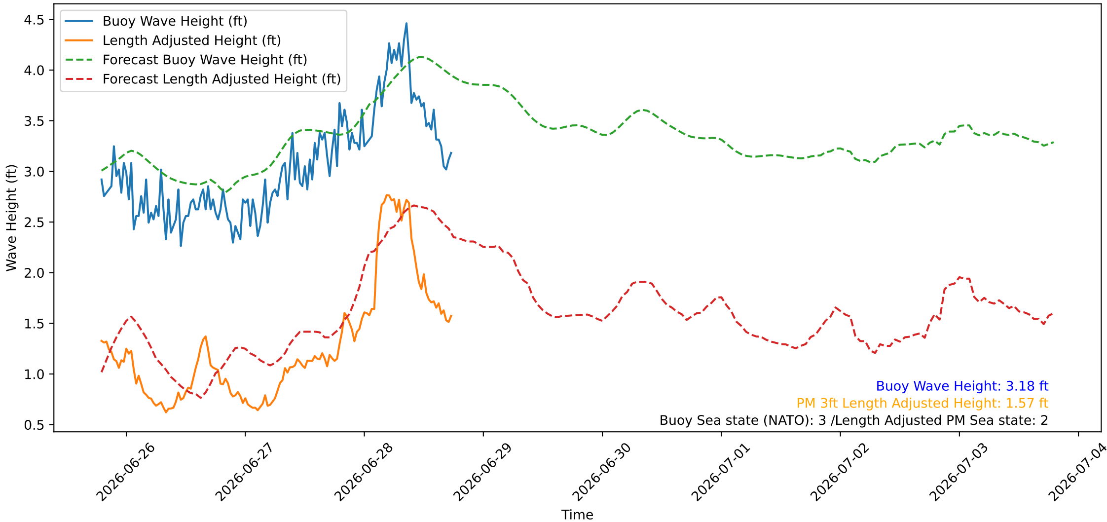
Wave Heights over Time for Red Beach at 2026-06-28 18:30:45
