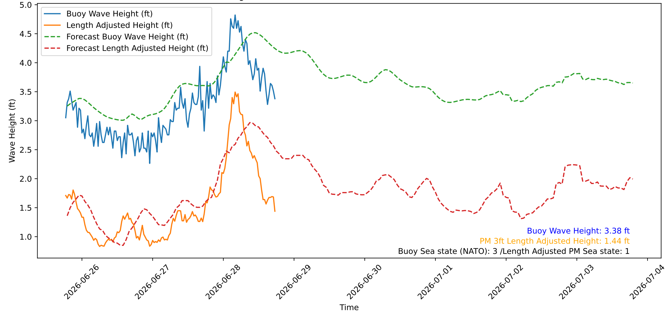
Wave Heights over Time for Green Beach at 2026-06-28 18:31:07
