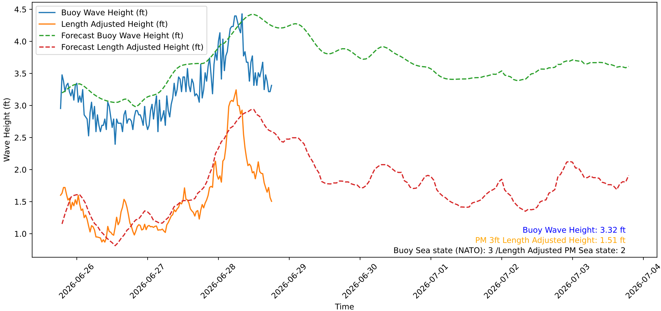
Wave Heights over Time for Oceanside Harbor at 2026-06-28 18:30:26
