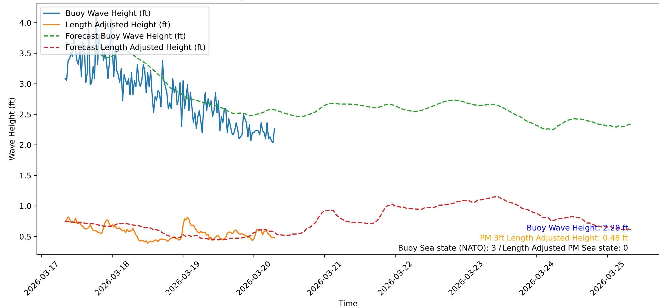
Wave Heights over Time for Green Beach at 2026-03-20 08:01:09
