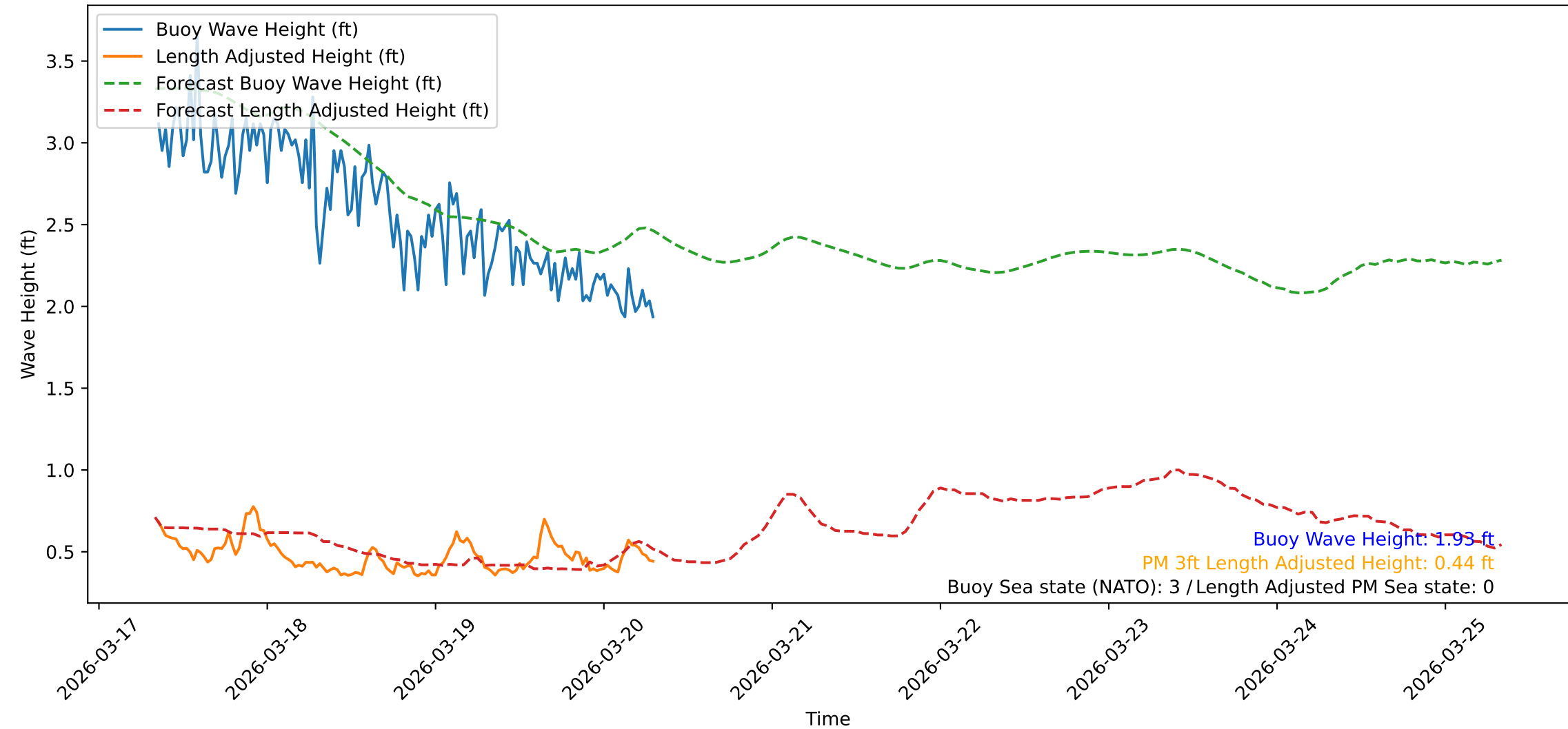
Wave Heights over Time for Red Beach at 2026-03-20 08:00:47
