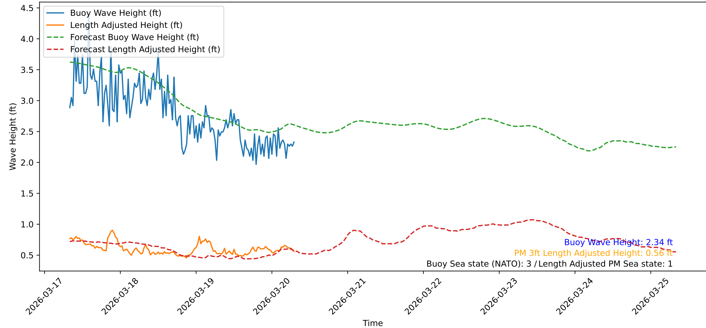
Wave Heights over Time for Oceanside Harbor at 2026-03-20 08:00:31
