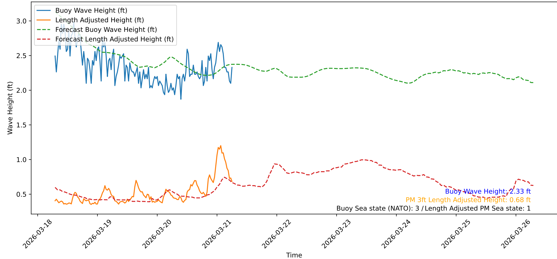
Wave Heights over Time for Red Beach at 2026-03-21 06:50:49
