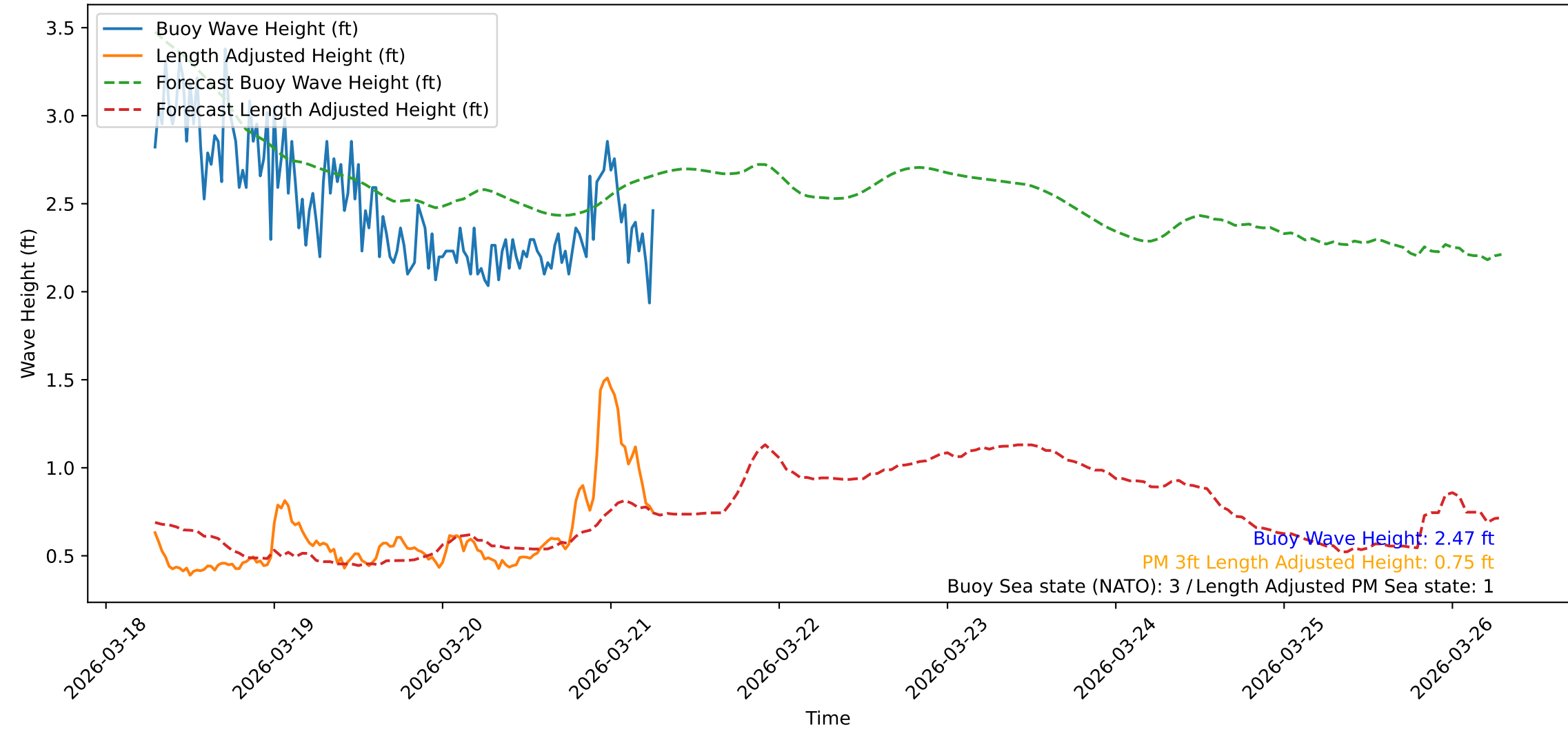
Wave Heights over Time for Green Beach at 2026-03-21 06:51:12
