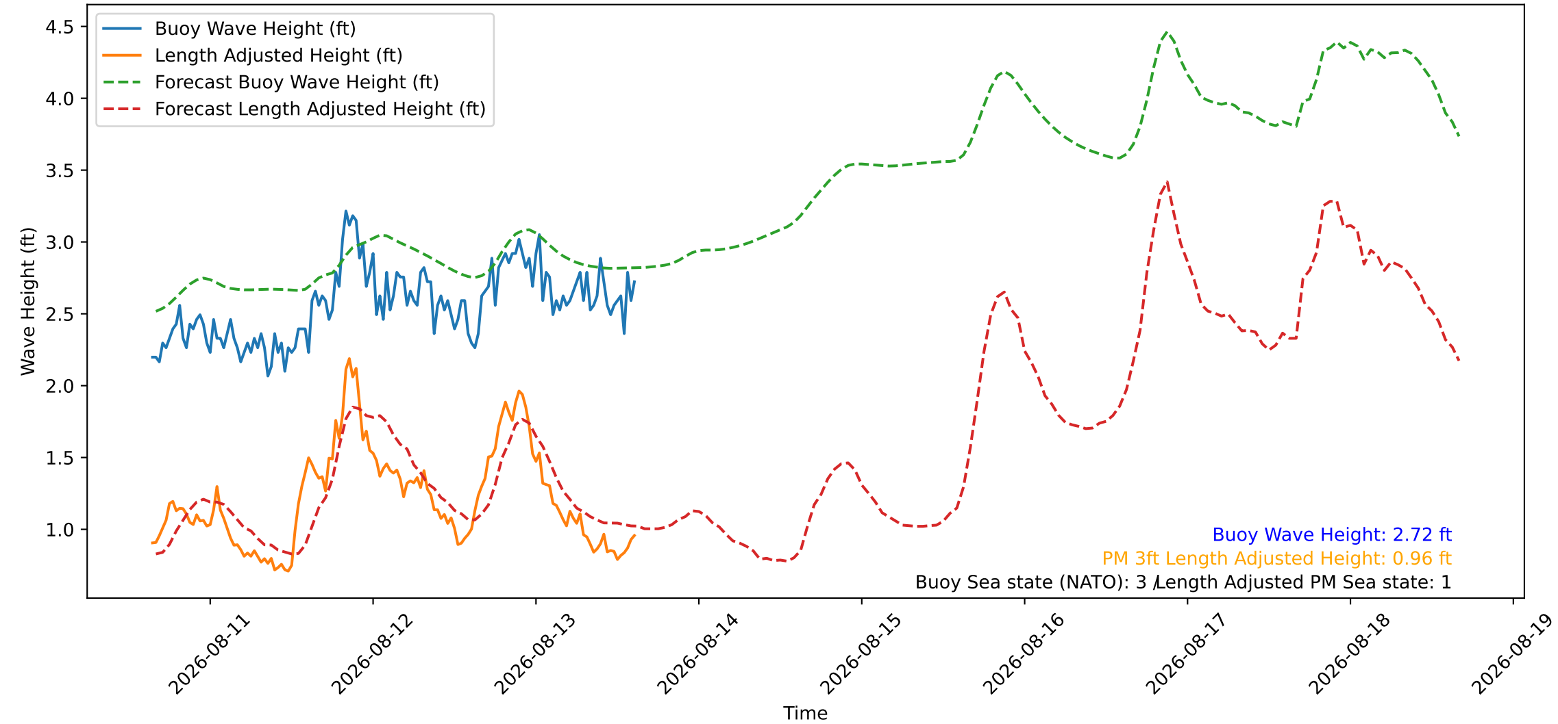
Wave Heights over Time for Green Beach at 2026-08-13 15:31:09
