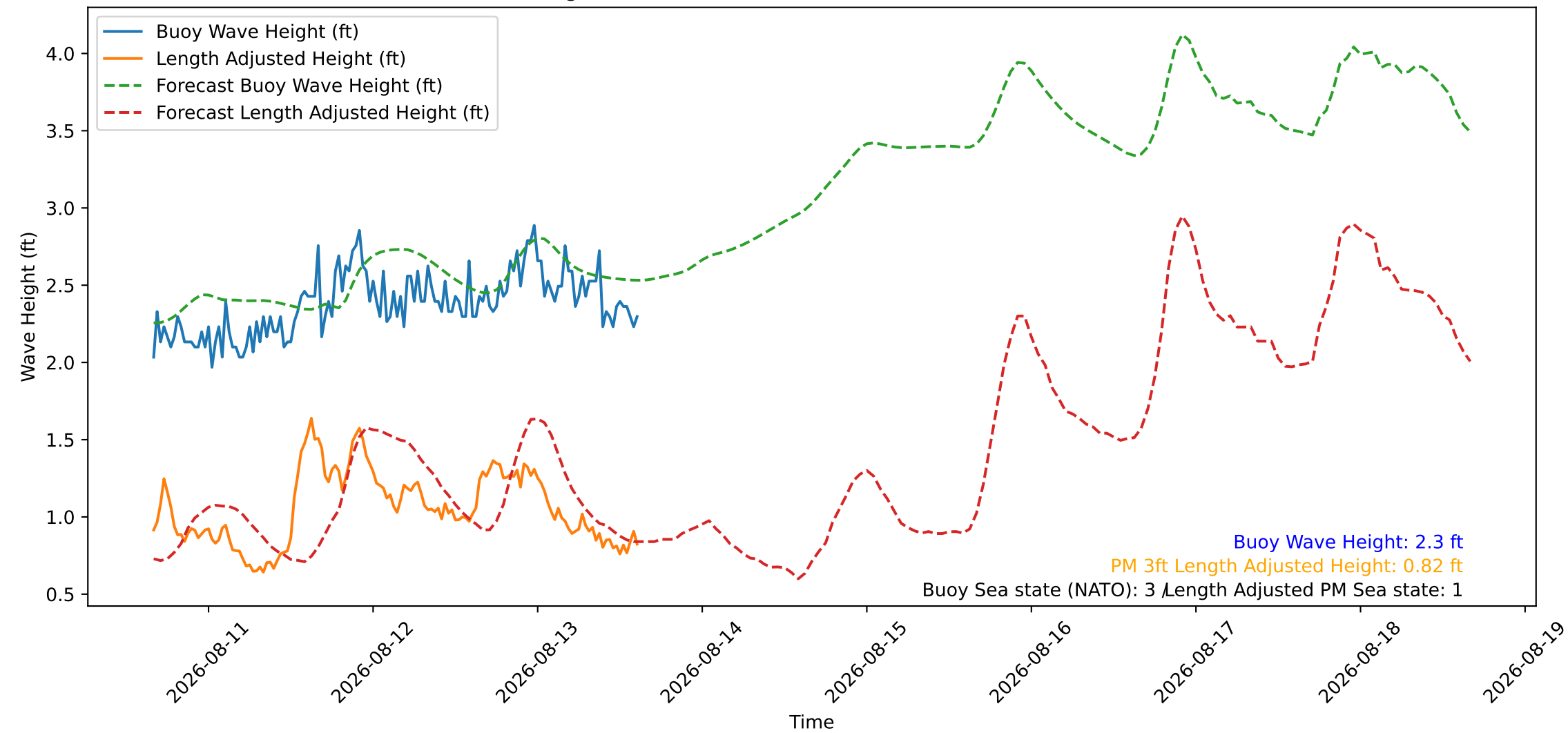
Wave Heights over Time for Red Beach at 2026-08-13 15:30:46
