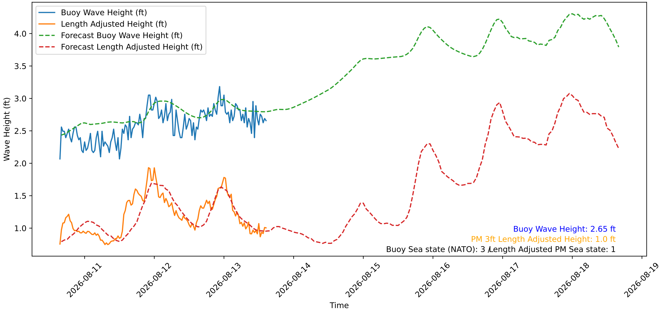
Wave Heights over Time for Oceanside Harbor at 2026-08-13 15:30:26
