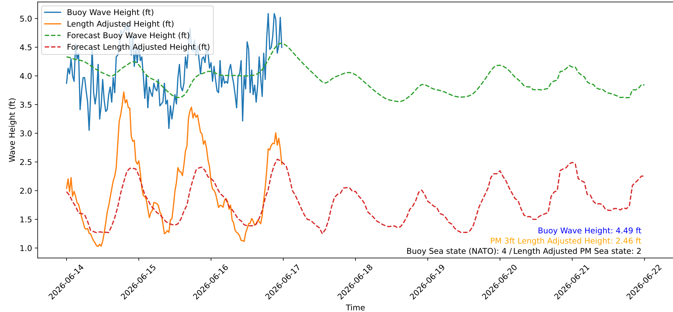
Wave Heights over Time for Green Beach at 2026-06-17 00:11:08
