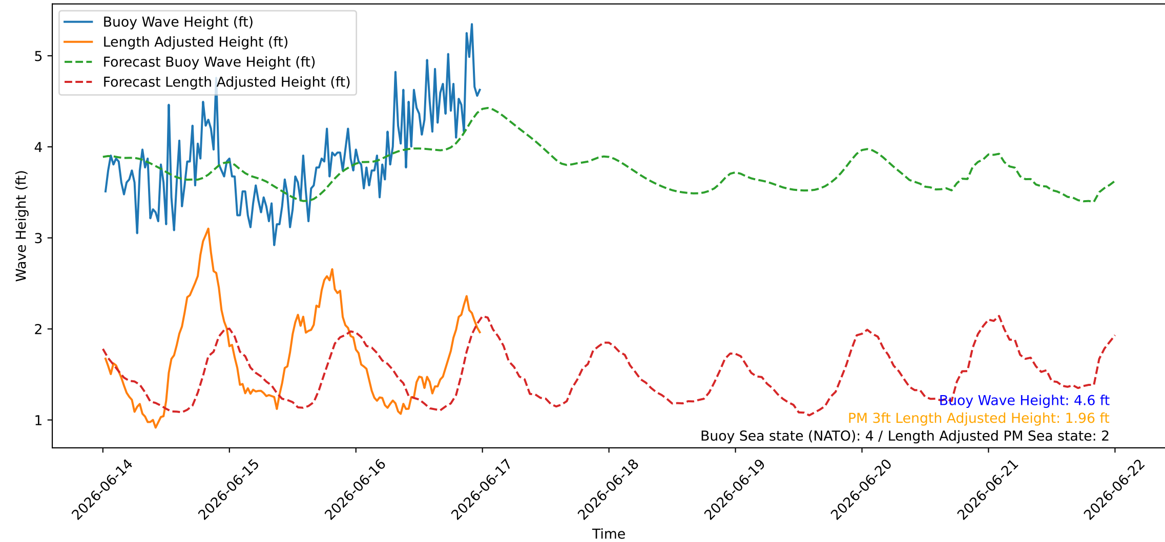
Wave Heights over Time for Red Beach at 2026-06-17 00:10:46
