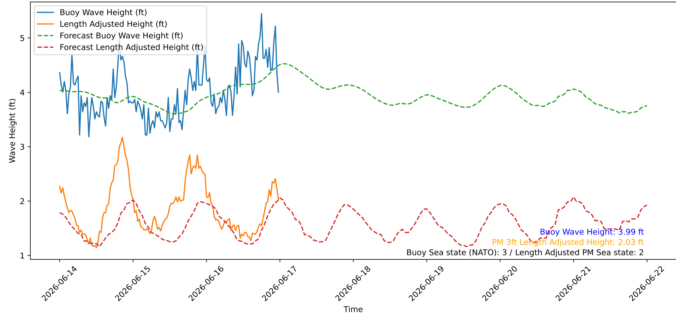
Wave Heights over Time for Oceanside Harbor at 2026-06-17 00:10:26
