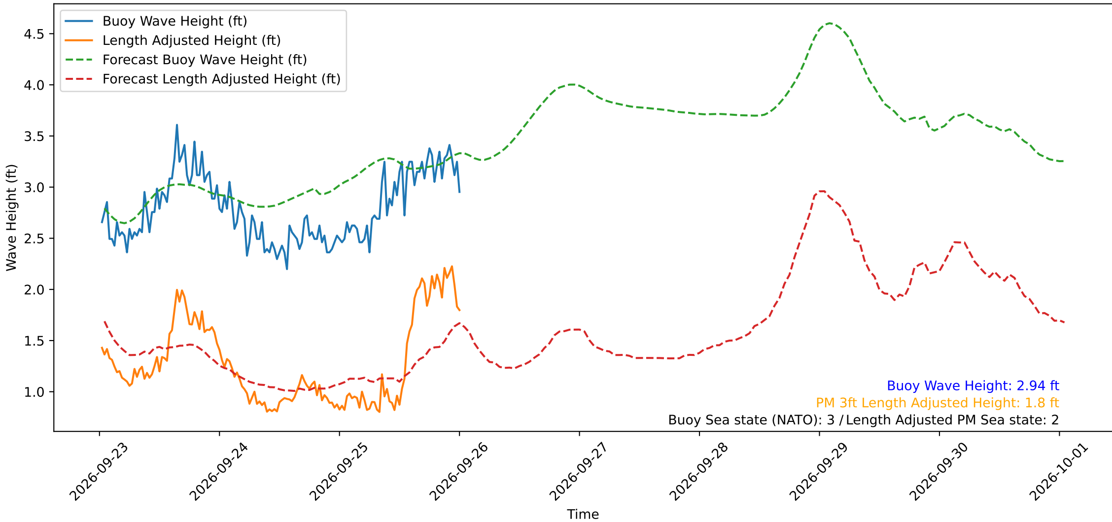
Wave Heights over Time for Oceanside Harbor at 2026-09-26 00:40:30
