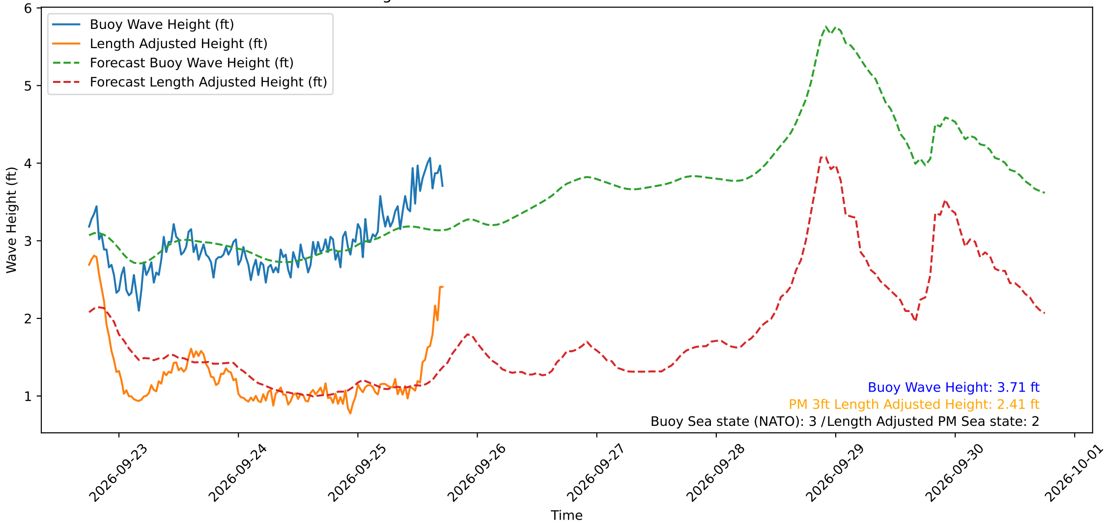
Wave Heights over Time for Green Beach at 2026-09-25 17:51:14
