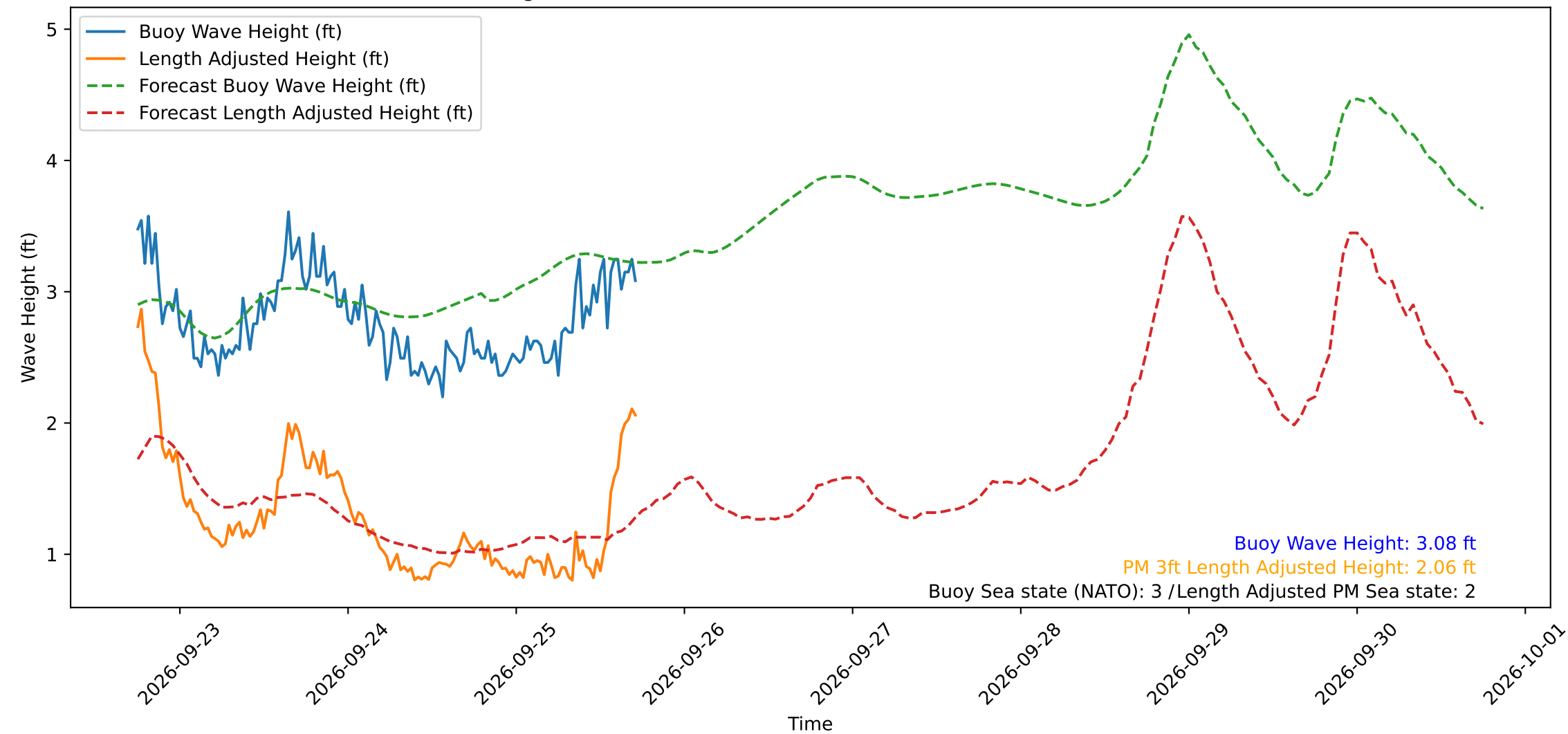
Wave Heights over Time for Oceanside Harbor at 2026-09-25 17:50:29
