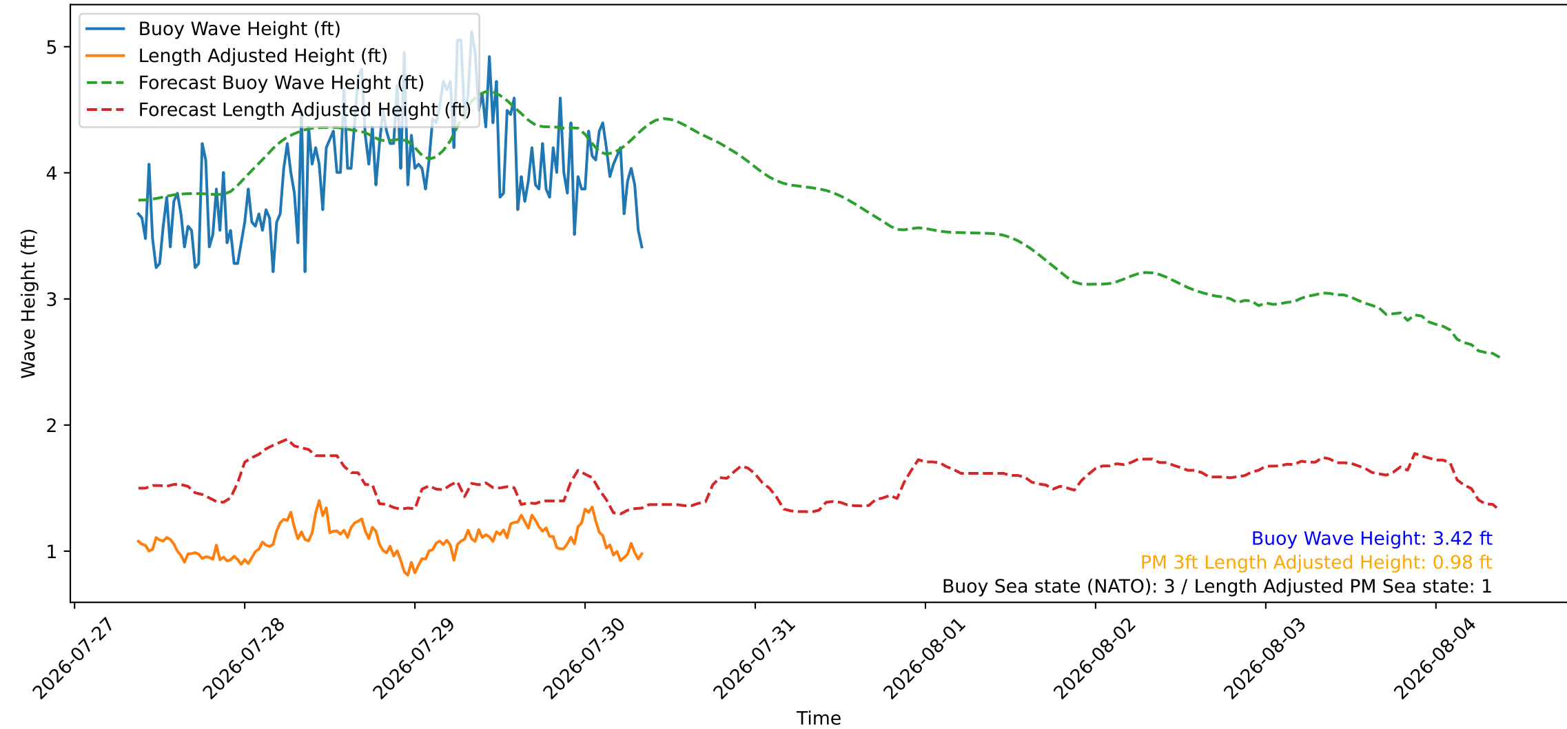
Wave Heights over Time for Red Beach at 2026-07-30 08:40:46
