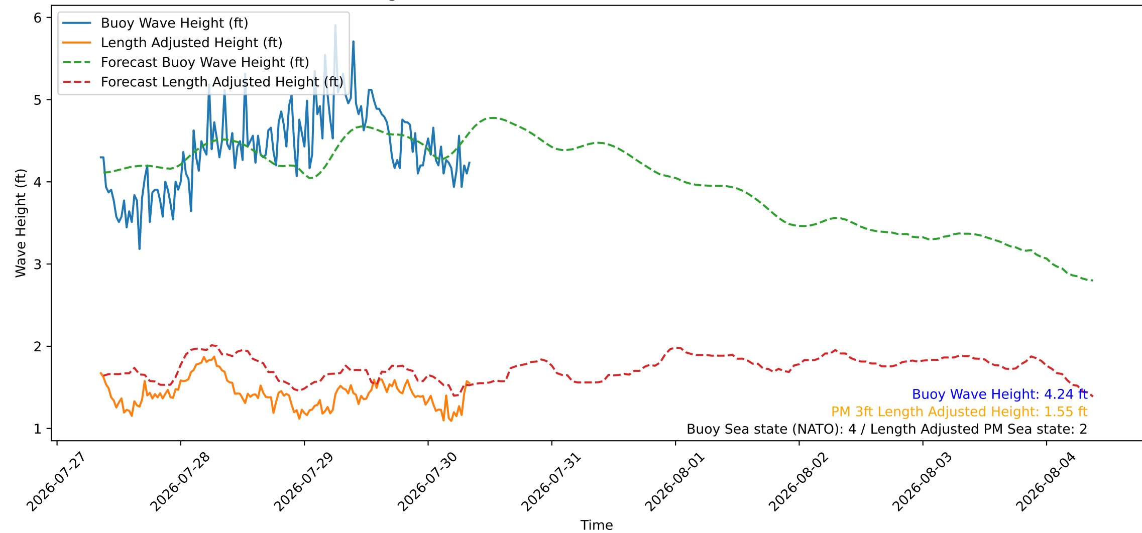
Wave Heights over Time for Oceanside Harbor at 2026-07-30 08:40:26
