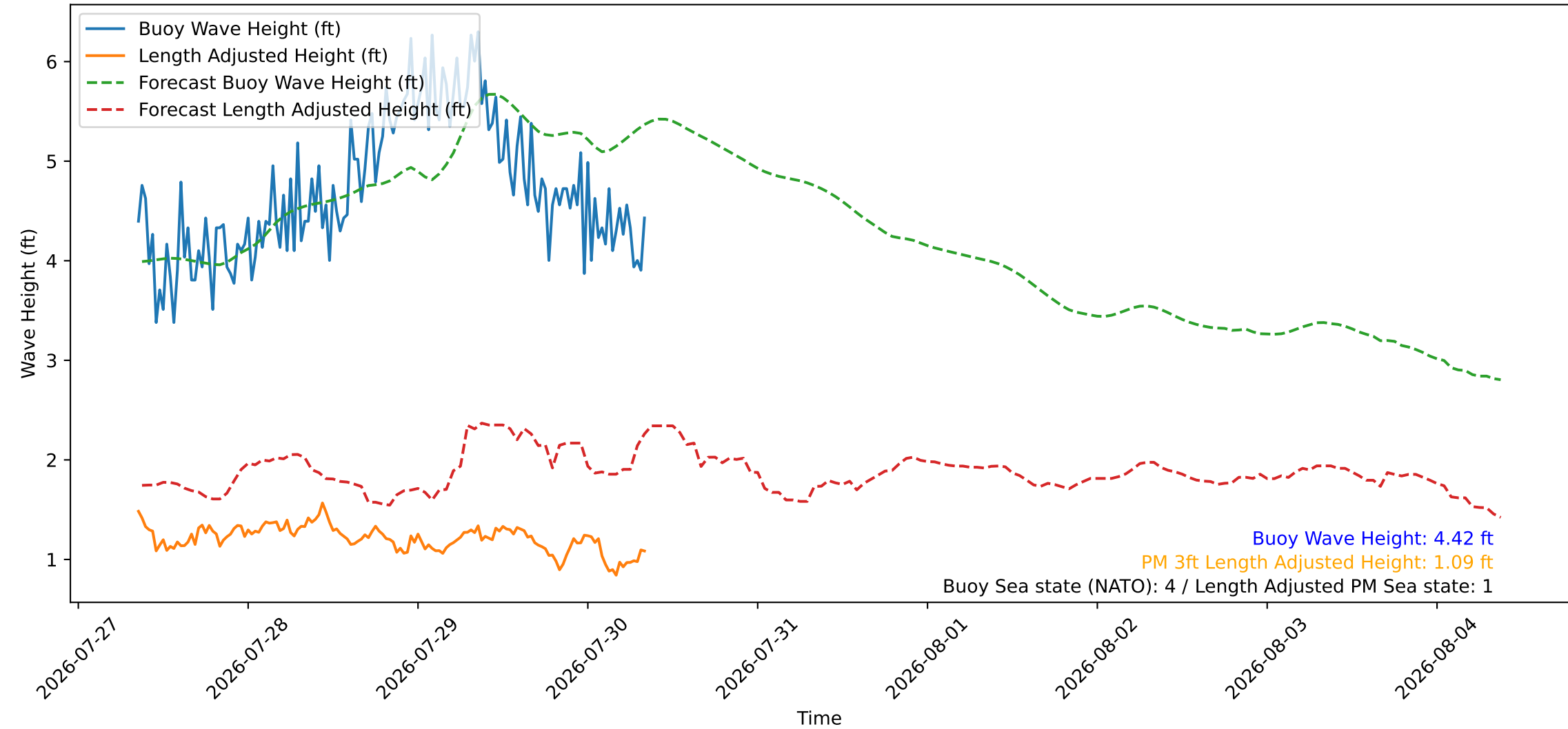
Wave Heights over Time for Green Beach at 2026-07-30 08:41:09
