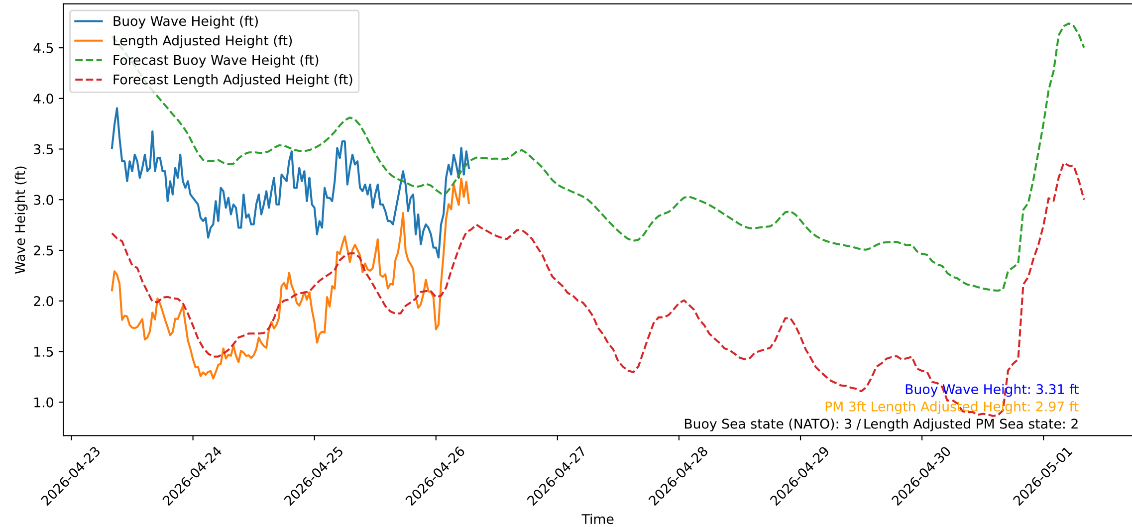
Wave Heights over Time for Green Beach at 2026-04-26 07:51:13
