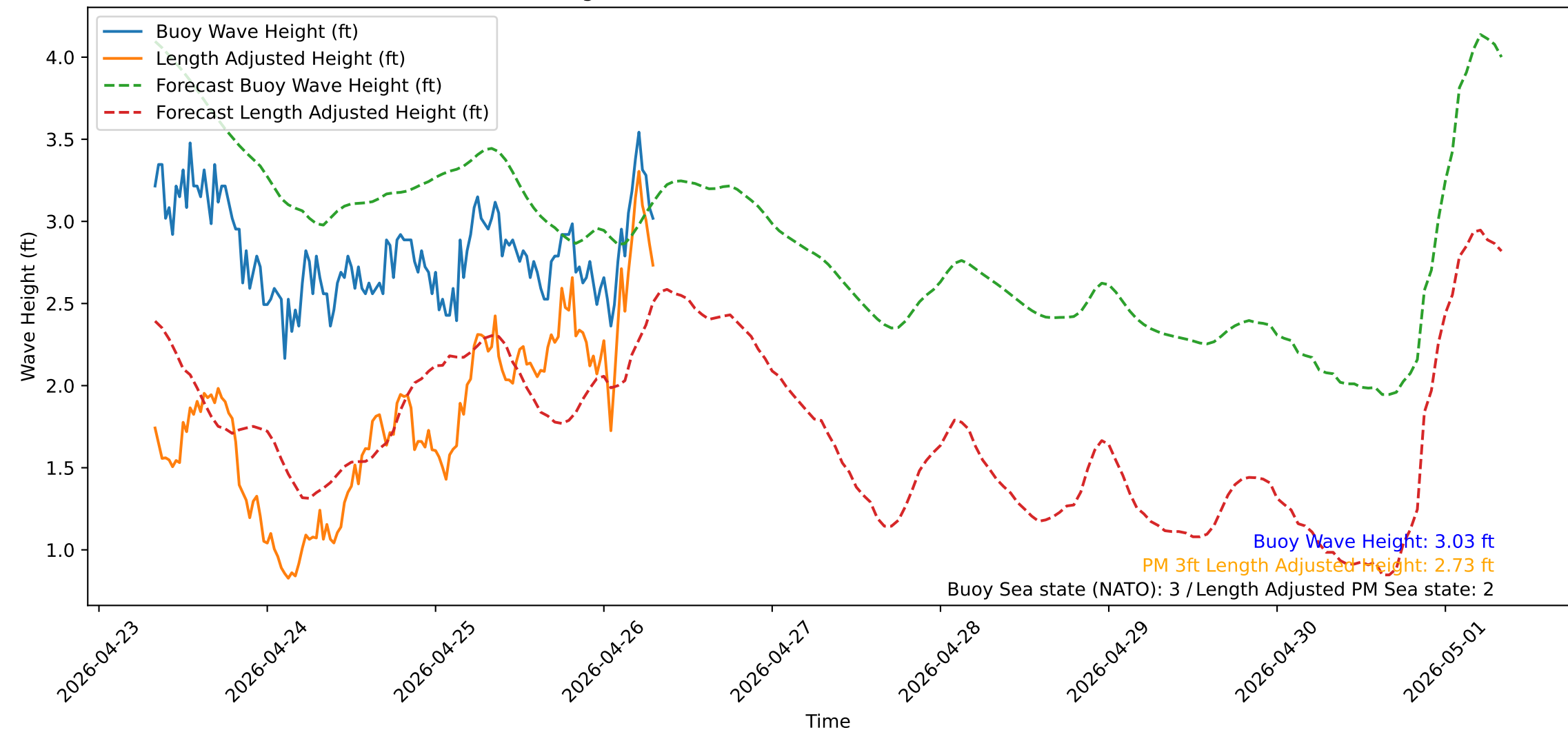
Wave Heights over Time for Red Beach at 2026-04-26 07:50:50
