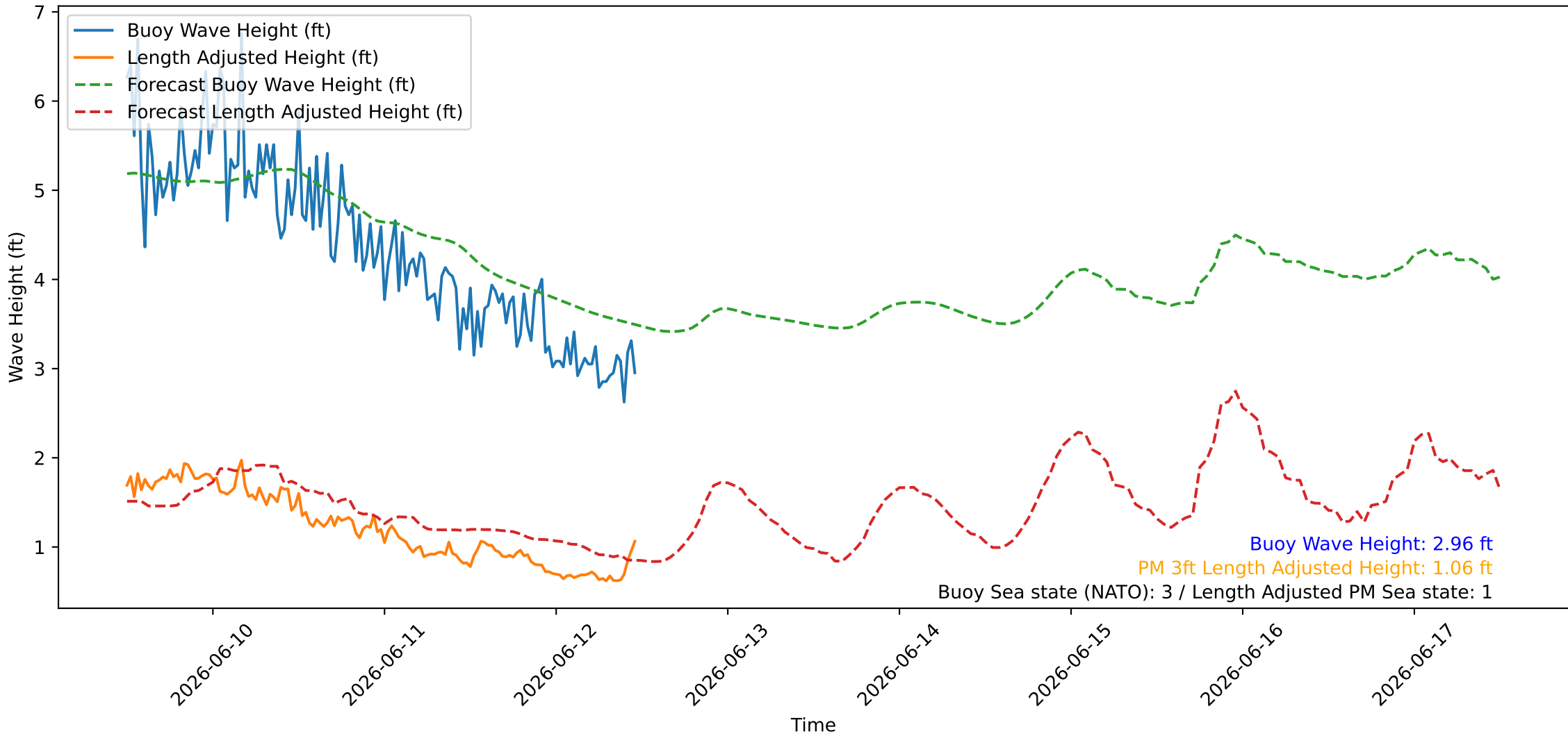
Wave Heights over Time for Red Beach at 2026-06-12 11:50:48
