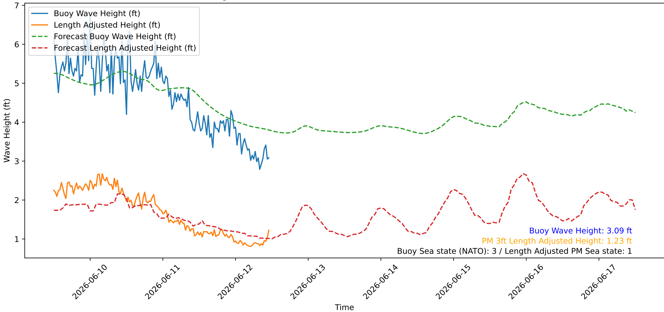
Wave Heights over Time for Oceanside Harbor at 2026-06-12 11:50:26
