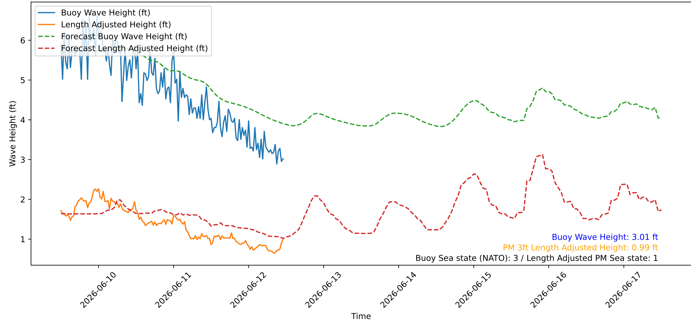
Wave Heights over Time for Green Beach at 2026-06-12 11:51:10
