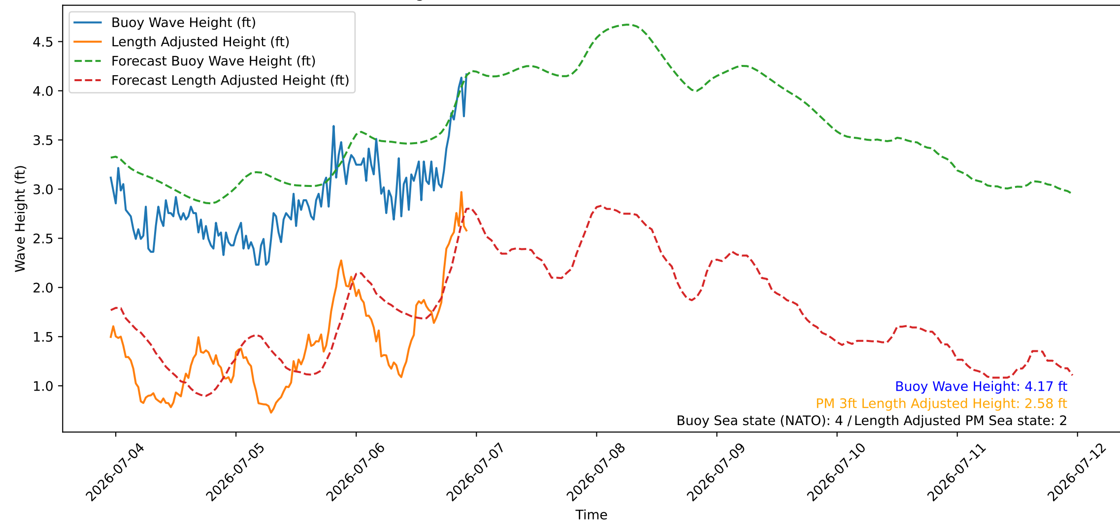
Wave Heights over Time for Red Beach at 2026-07-06 22:40:46
