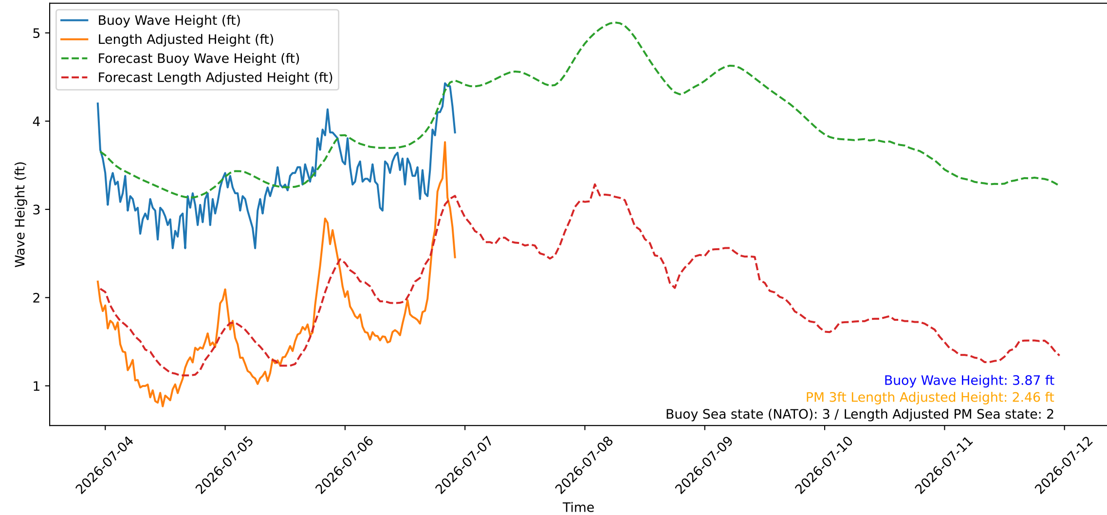
Wave Heights over Time for Green Beach at 2026-07-06 22:41:08
