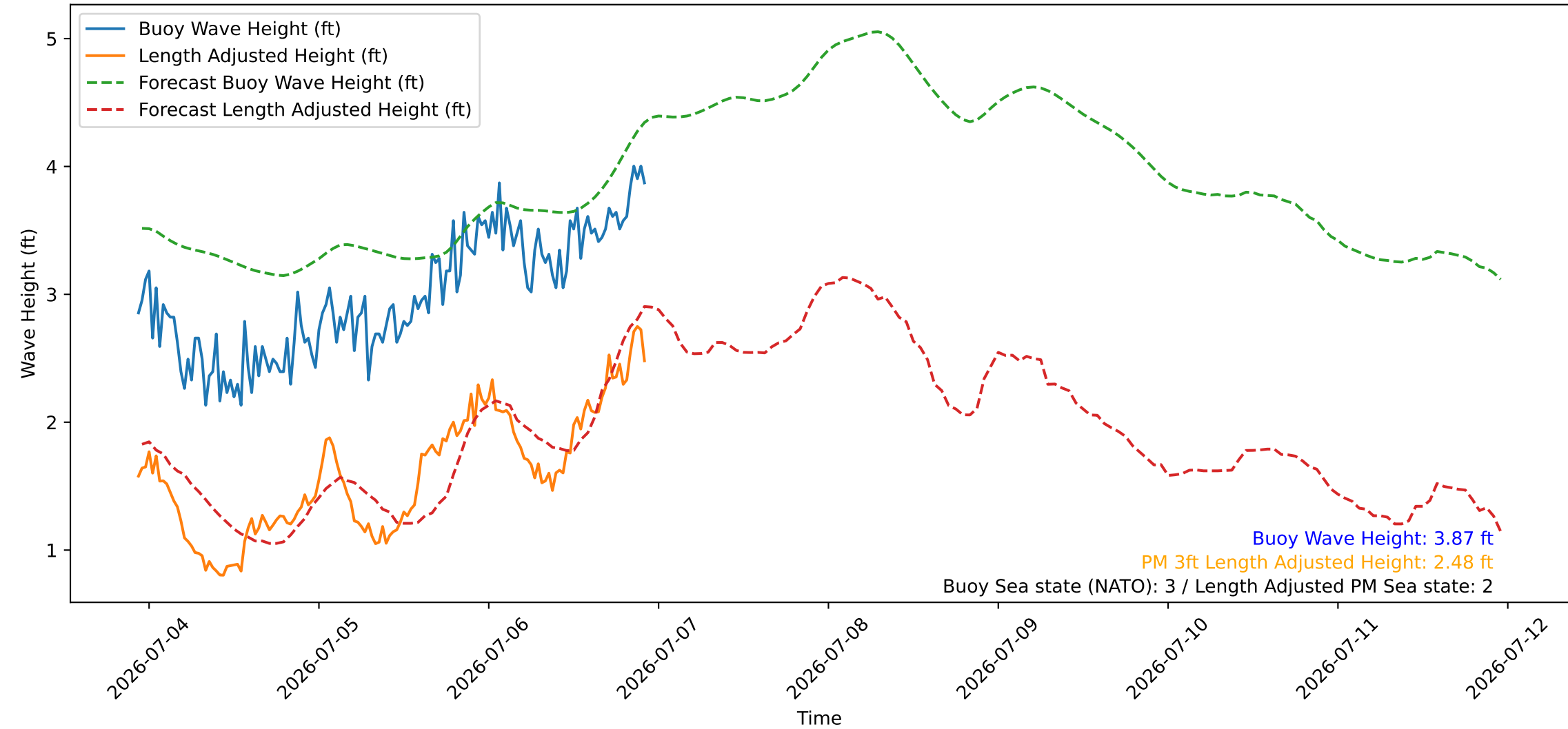
Wave Heights over Time for Oceanside Harbor at 2026-07-06 22:40:26
