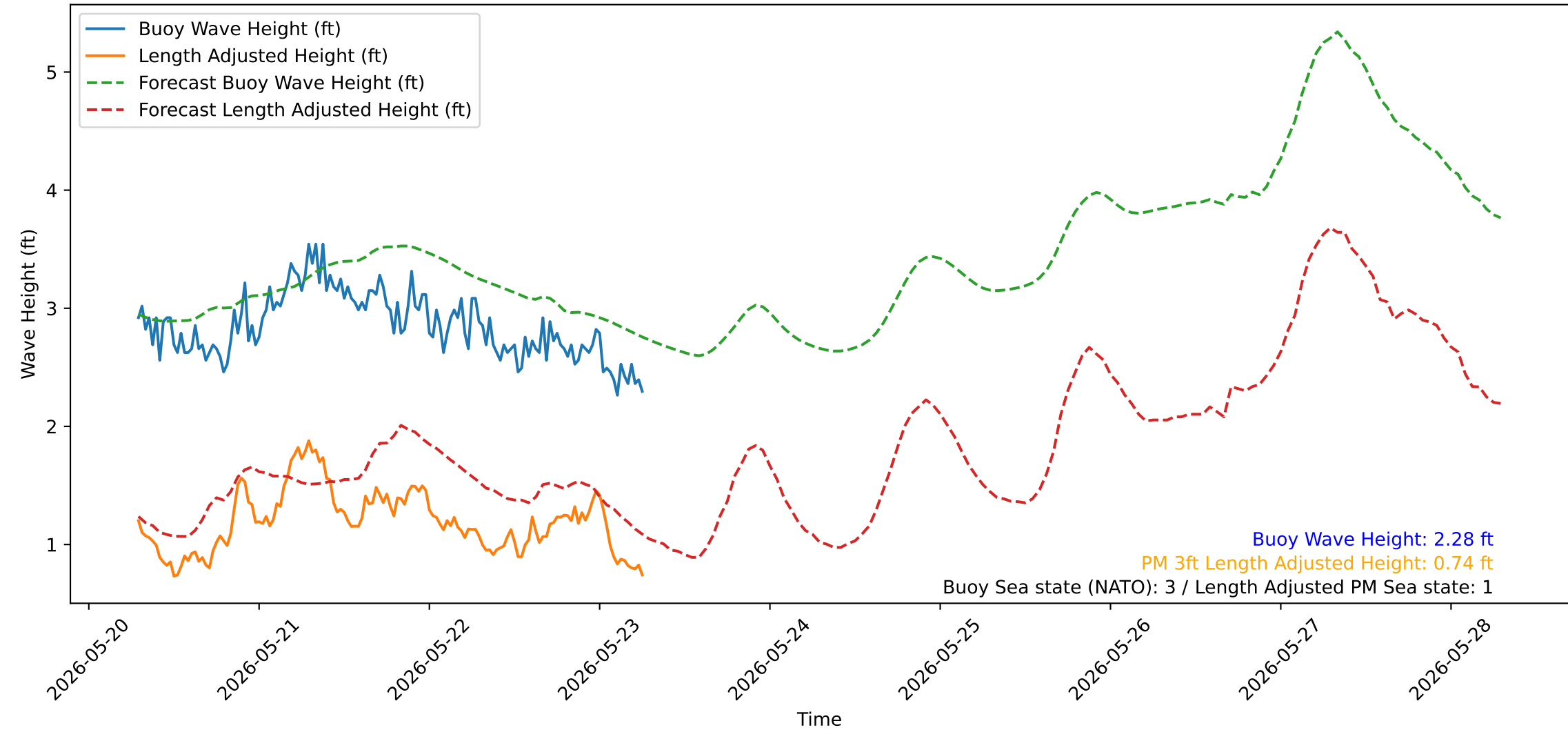
Wave Heights over Time for Green Beach at 2026-05-23 07:01:12
