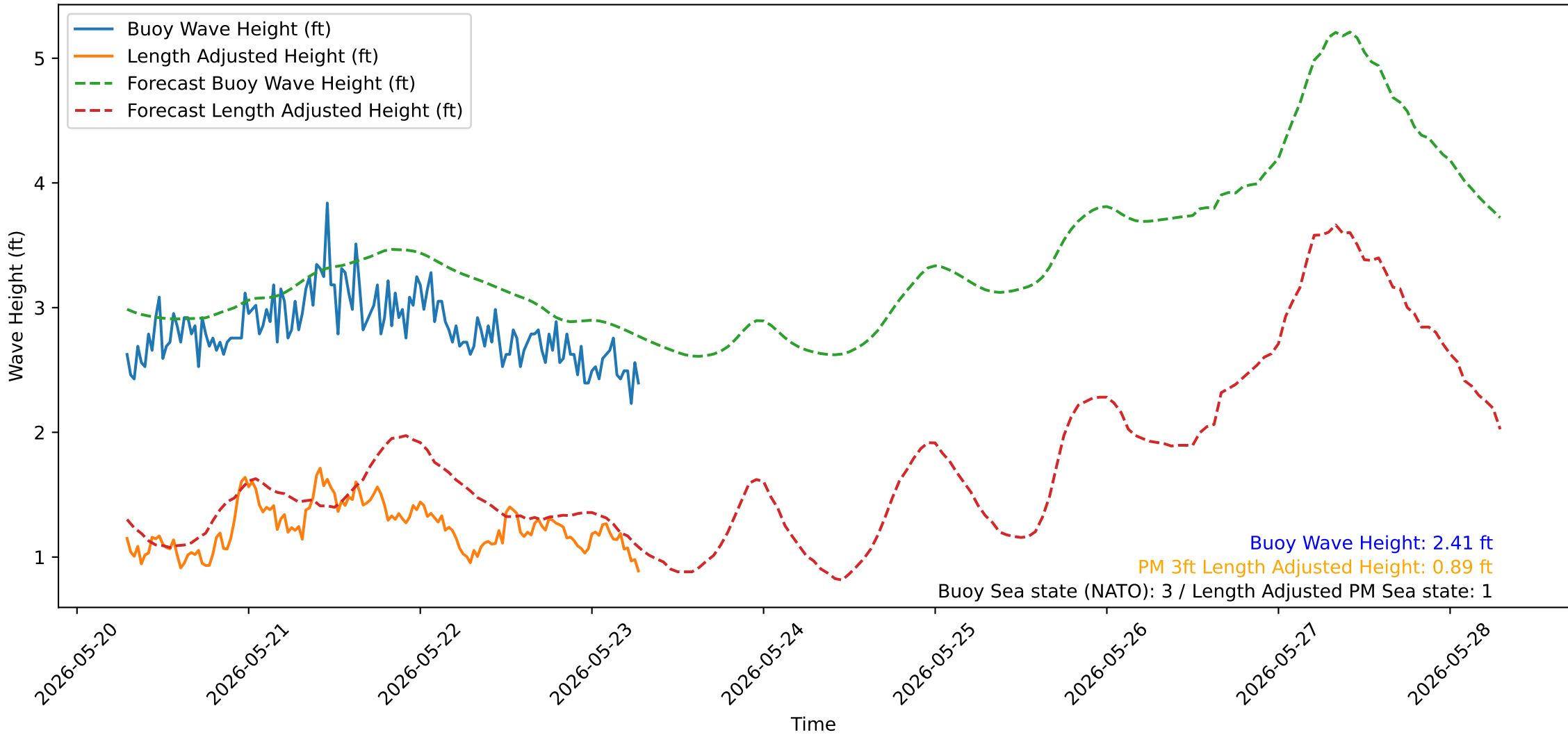
Wave Heights over Time for Oceanside Harbor at 2026-05-23 07:00:31
