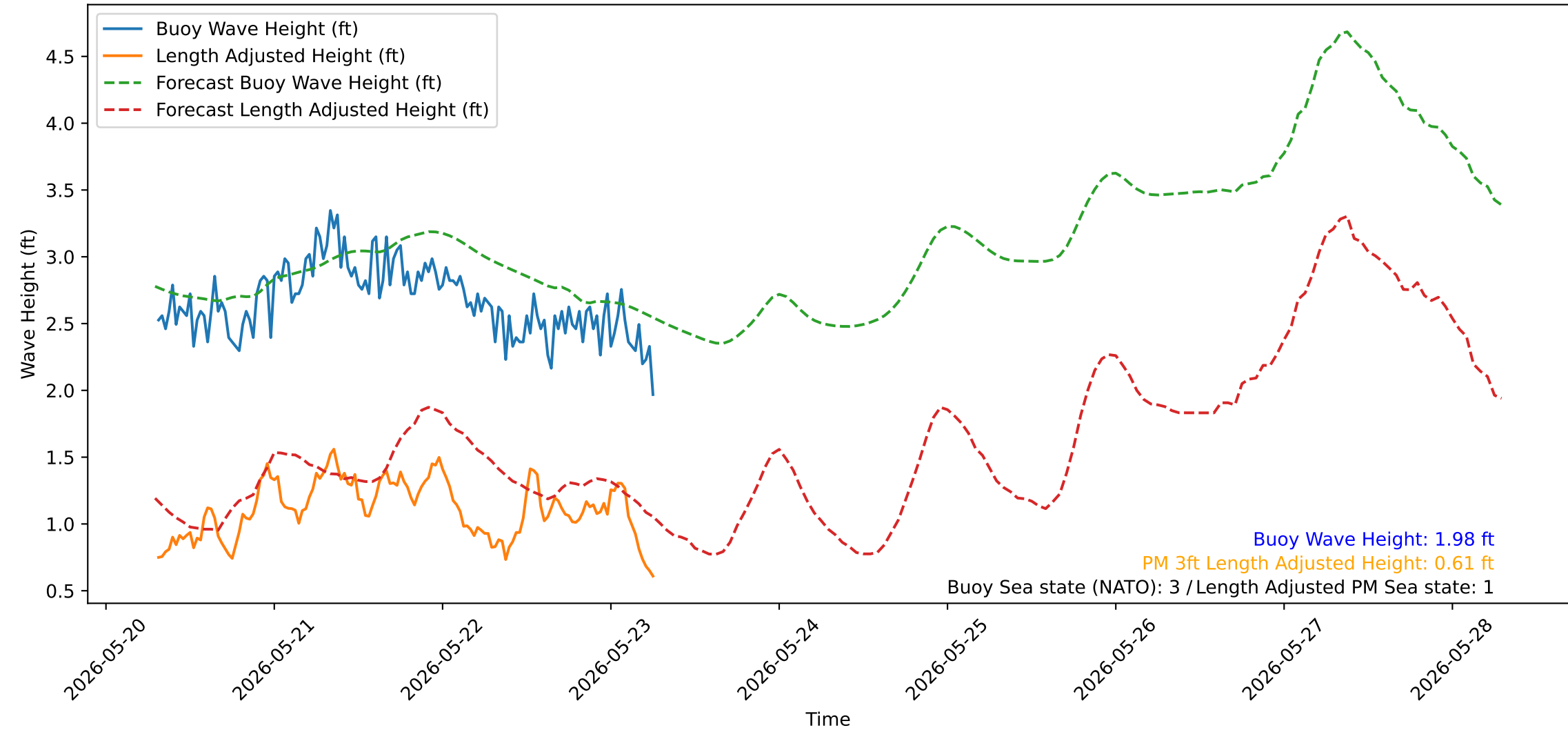
Wave Heights over Time for Red Beach at 2026-05-23 07:00:50
