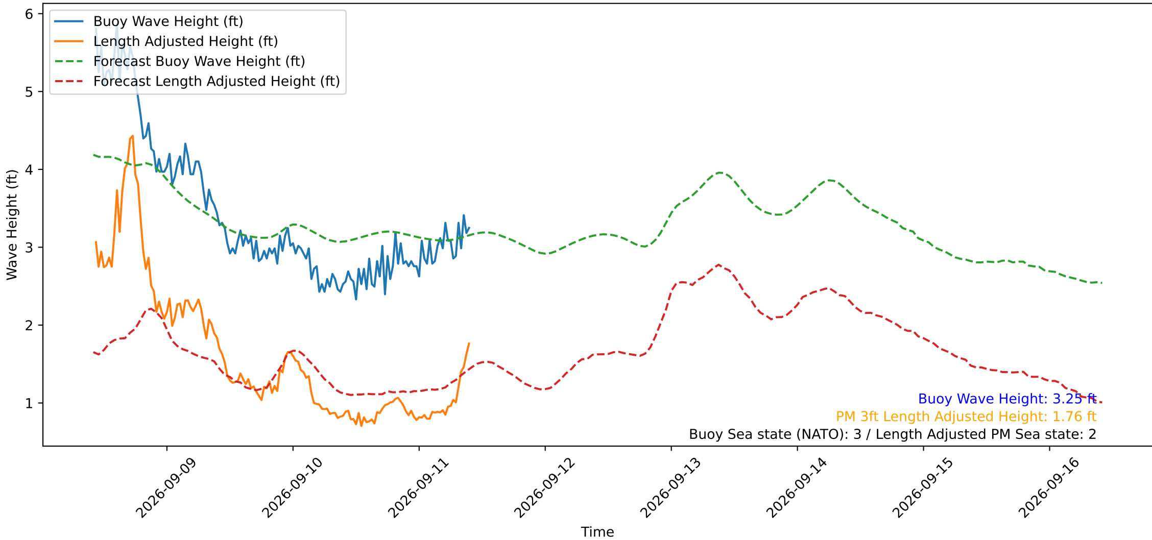
Wave Heights over Time for Red Beach at 2026-09-11 10:10:50
