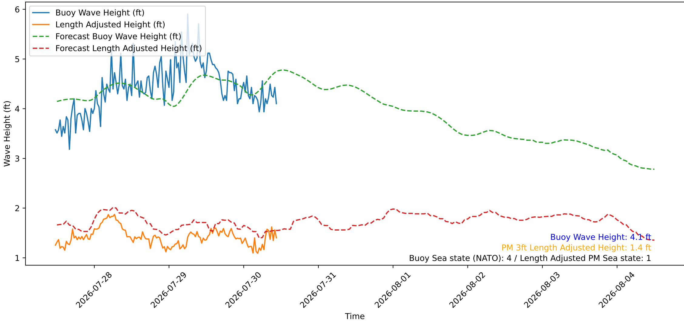
Wave Heights over Time for Oceanside Harbor at 2026-07-30 11:30:26
