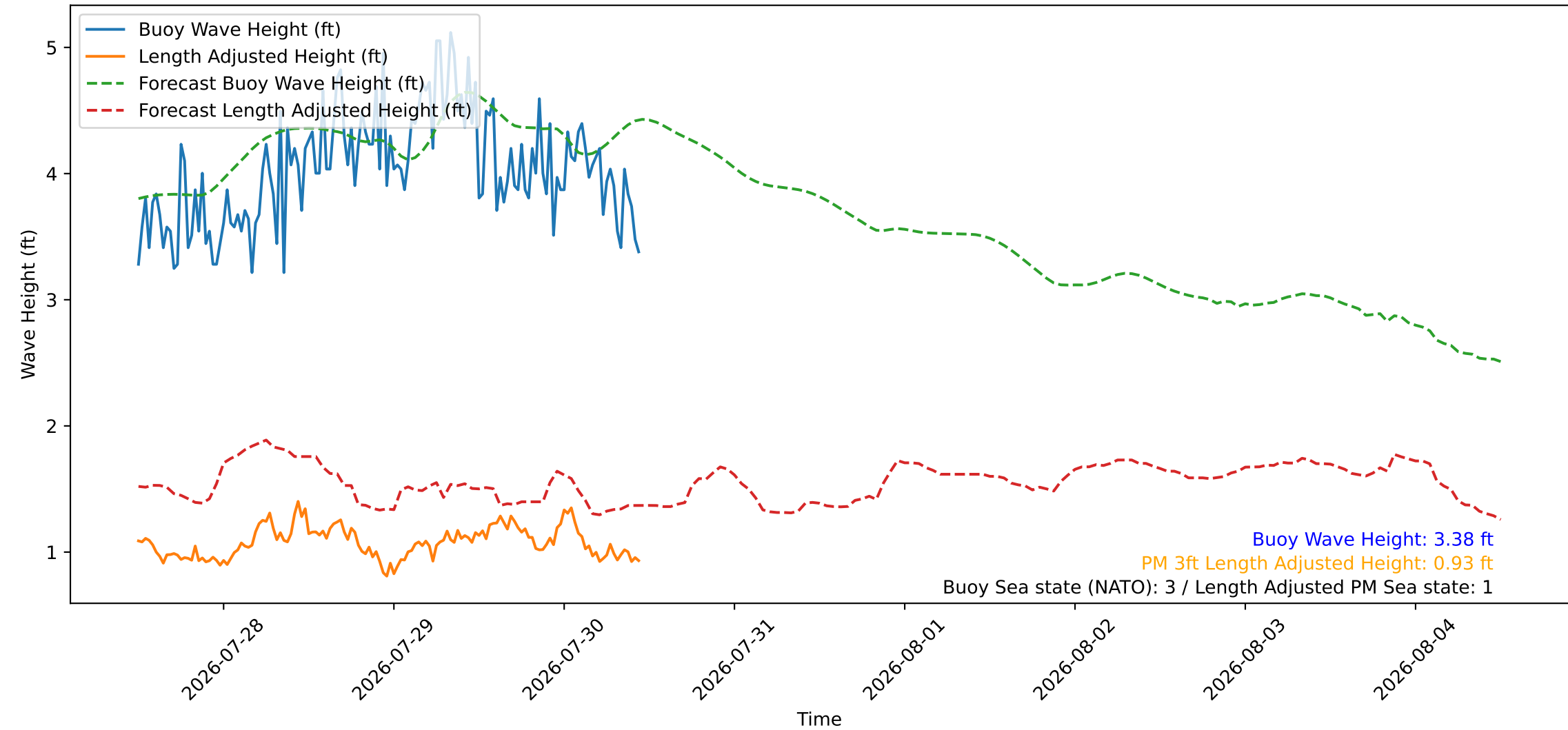
Wave Heights over Time for Red Beach at 2026-07-30 11:30:46
