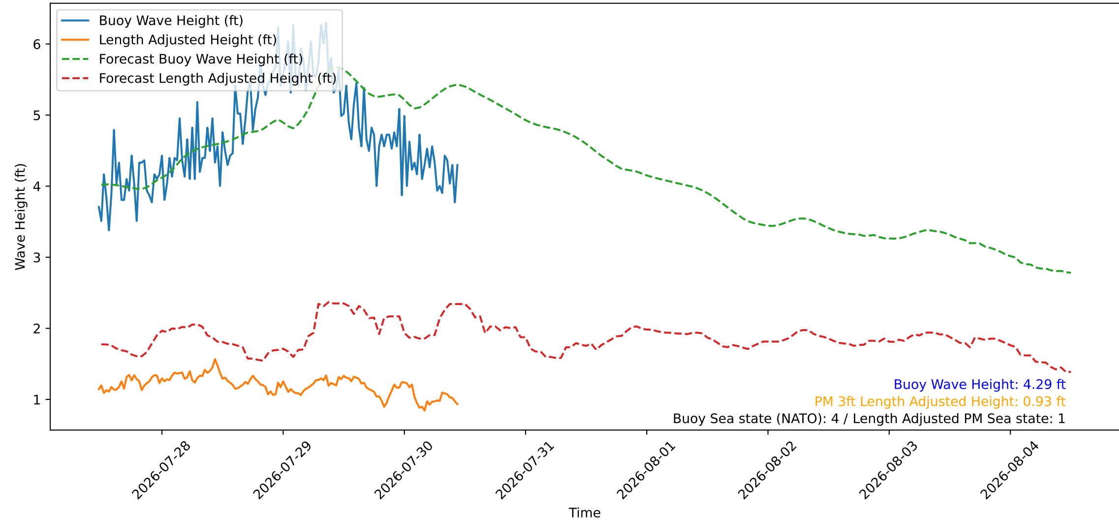
Wave Heights over Time for Green Beach at 2026-07-30 11:31:09
