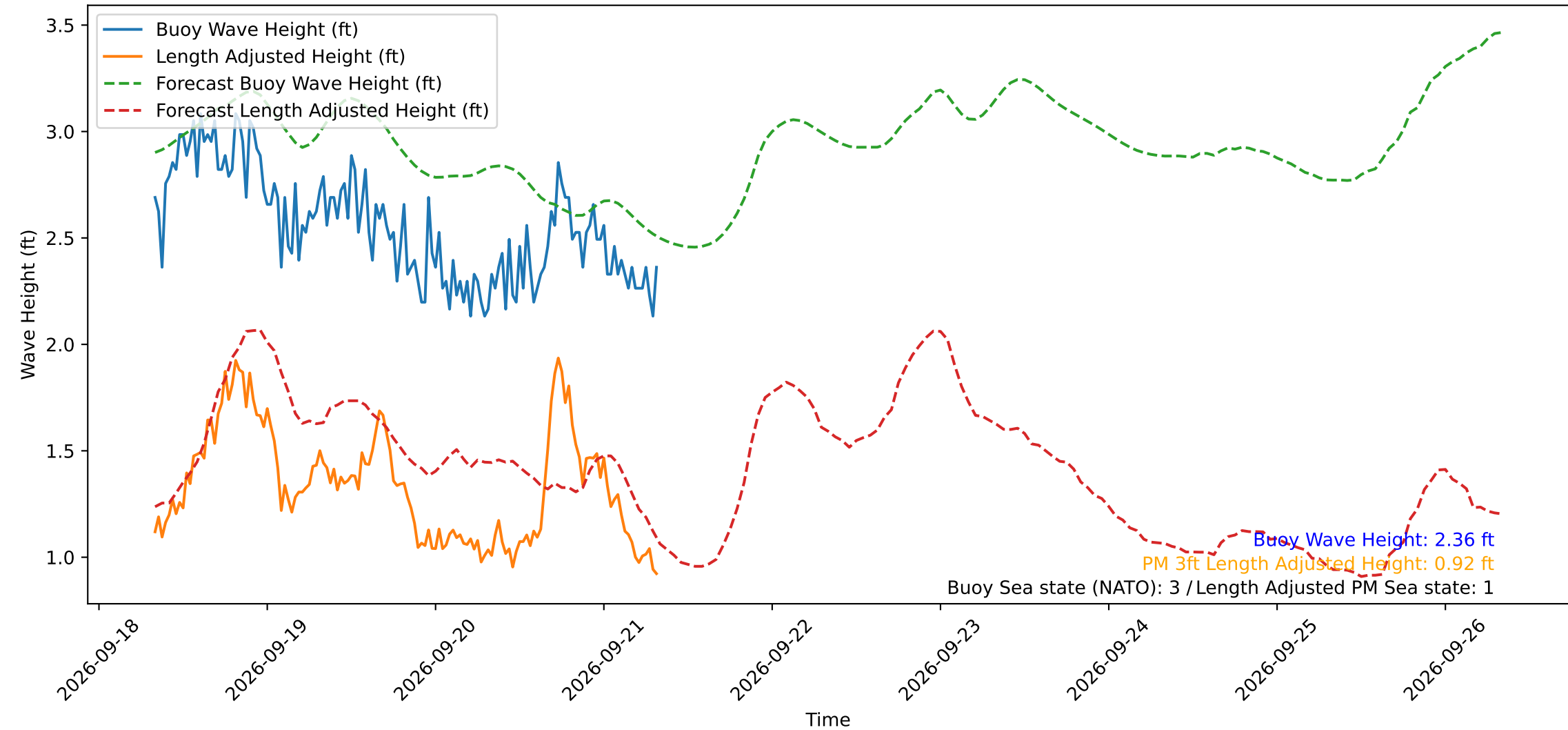
Wave Heights over Time for Oceanside Harbor at 2026-09-21 08:10:29
