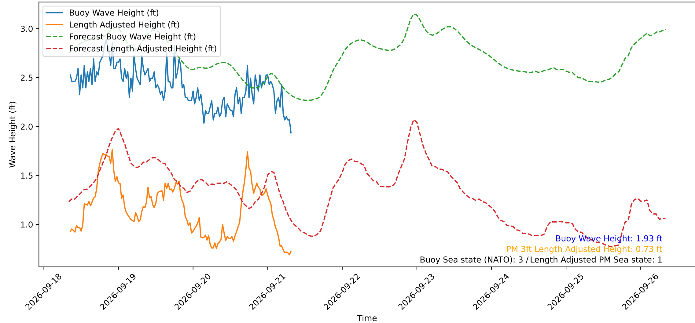
Wave Heights over Time for Red Beach at 2026-09-21 08:10:49
