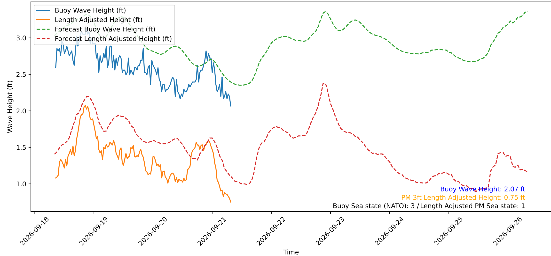
Wave Heights over Time for Green Beach at 2026-09-21 08:11:11
