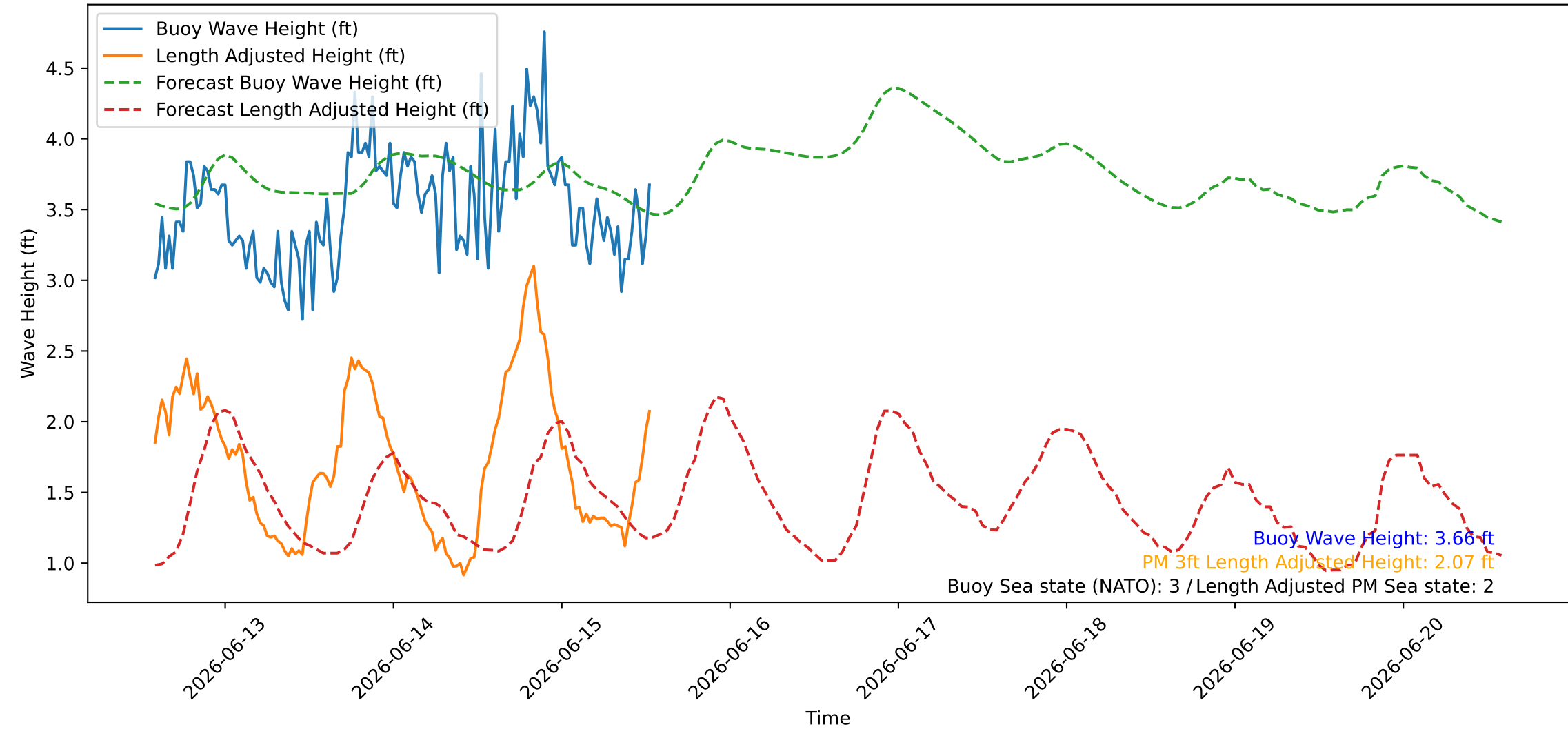
Wave Heights over Time for Red Beach at 2026-06-15 13:30:45
