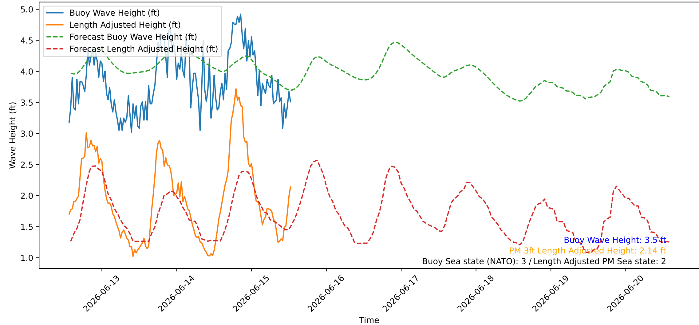
Wave Heights over Time for Green Beach at 2026-06-15 13:31:08
