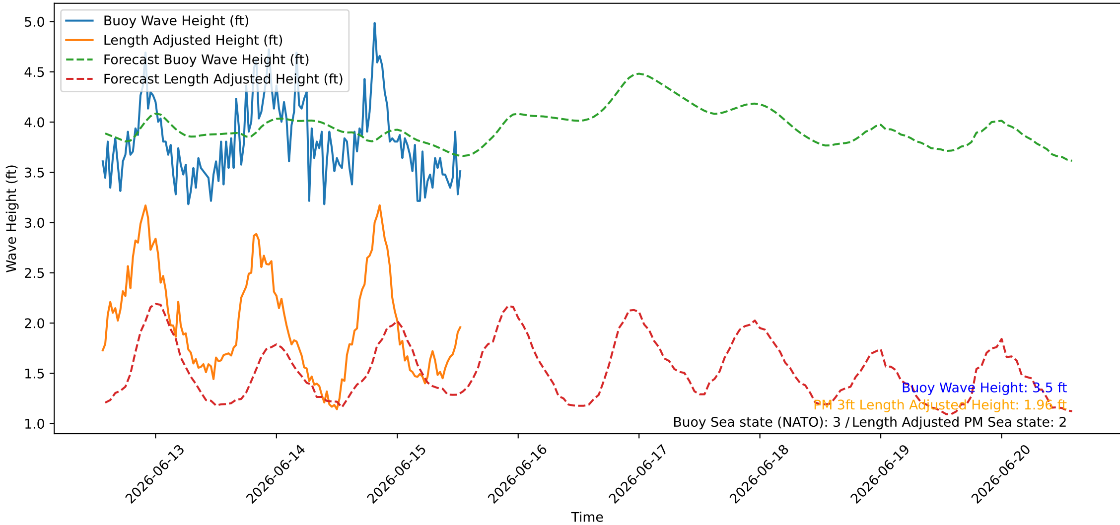
Wave Heights over Time for Oceanside Harbor at 2026-06-15 13:30:26
