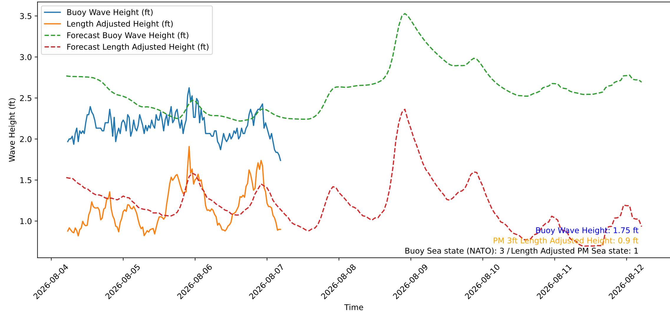
Wave Heights over Time for Green Beach at 2026-08-07 05:21:09
