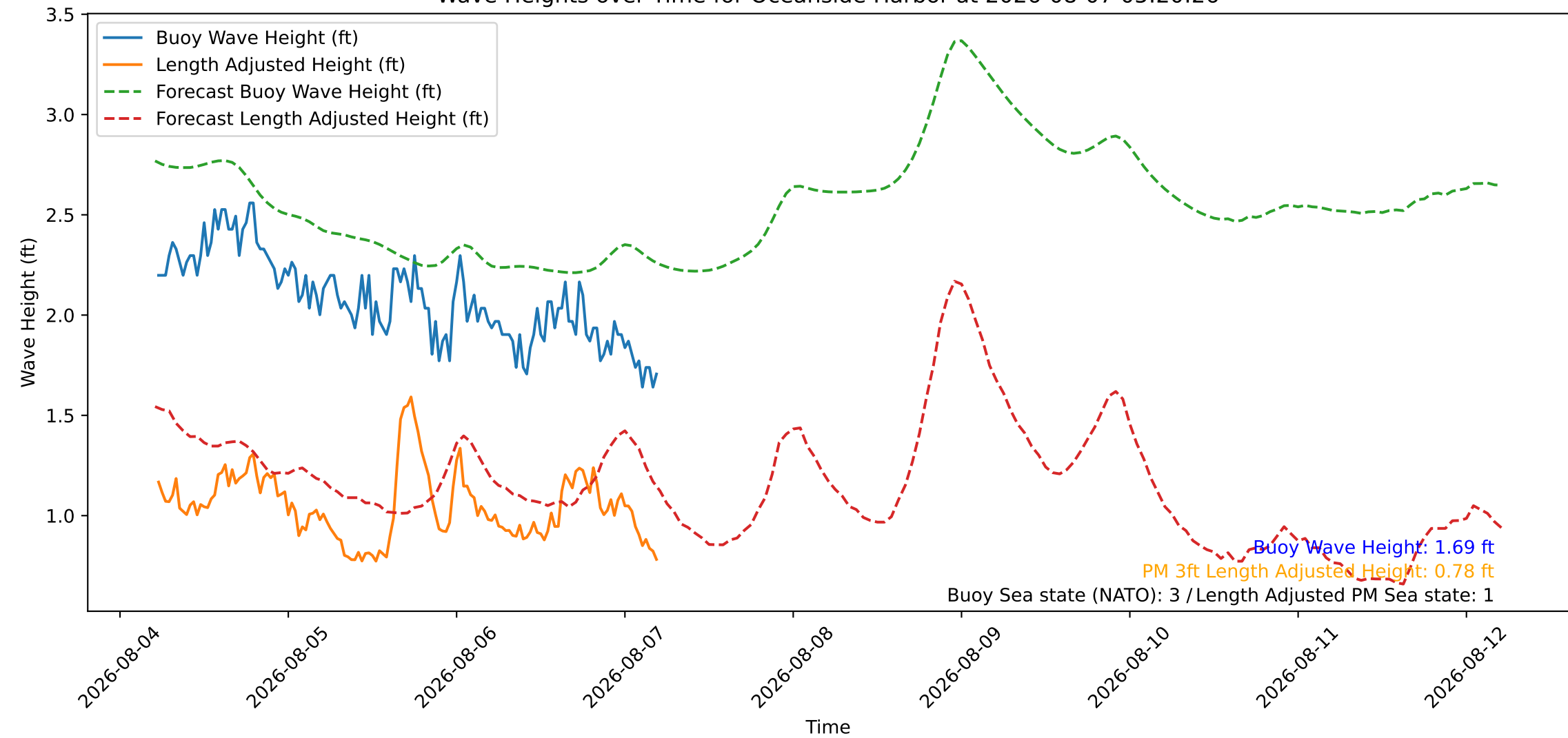
Wave Heights over Time for Oceanside Harbor at 2026-08-07 05:20:26
