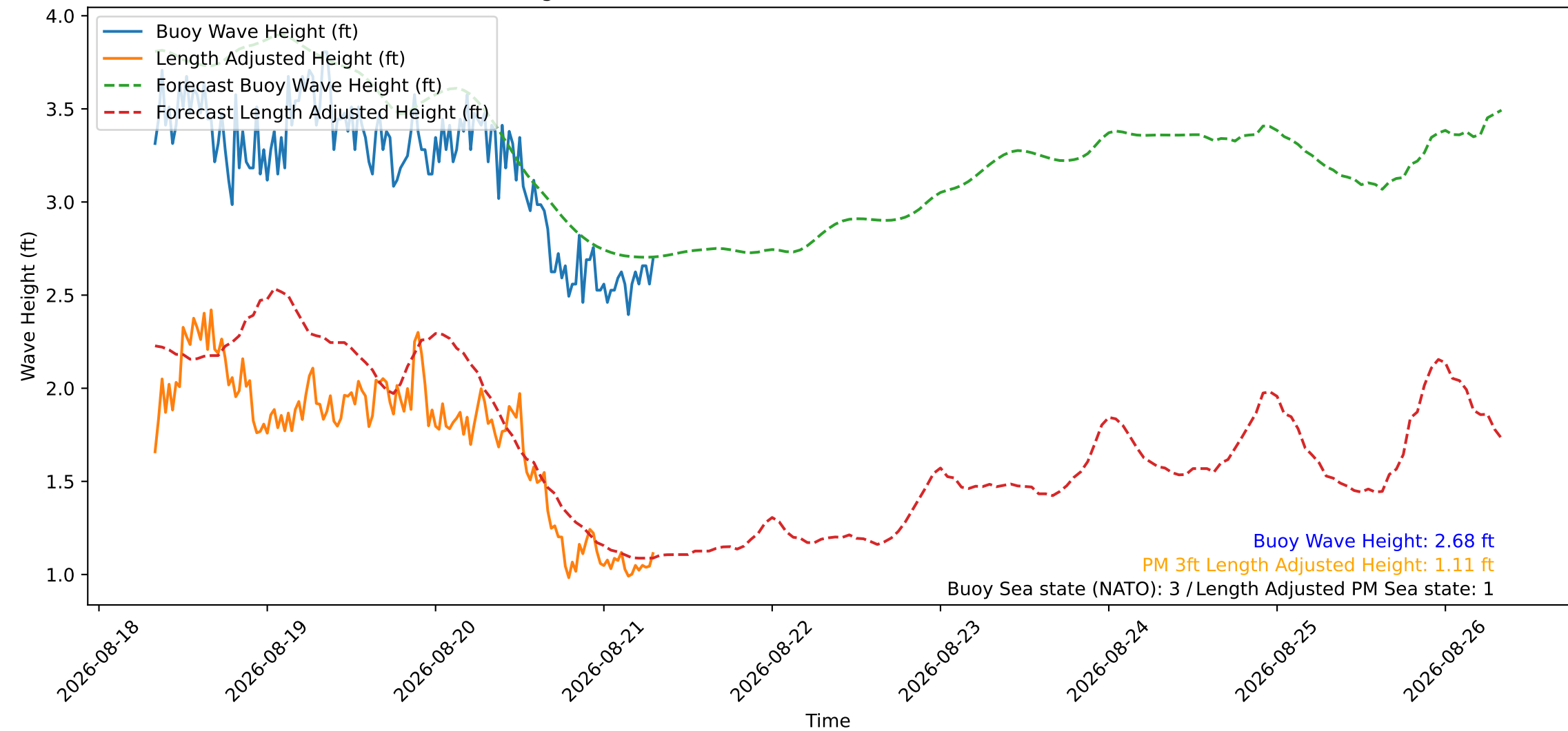
Wave Heights over Time for Oceanside Harbor at 2026-08-21 07:50:26
