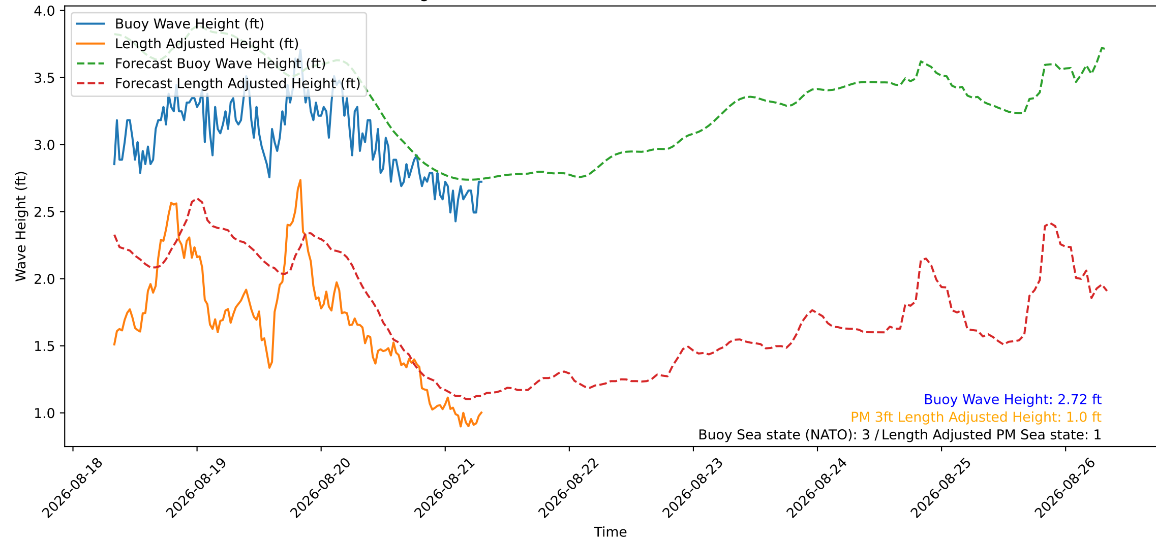
Wave Heights over Time for Green Beach at 2026-08-21 07:51:10
