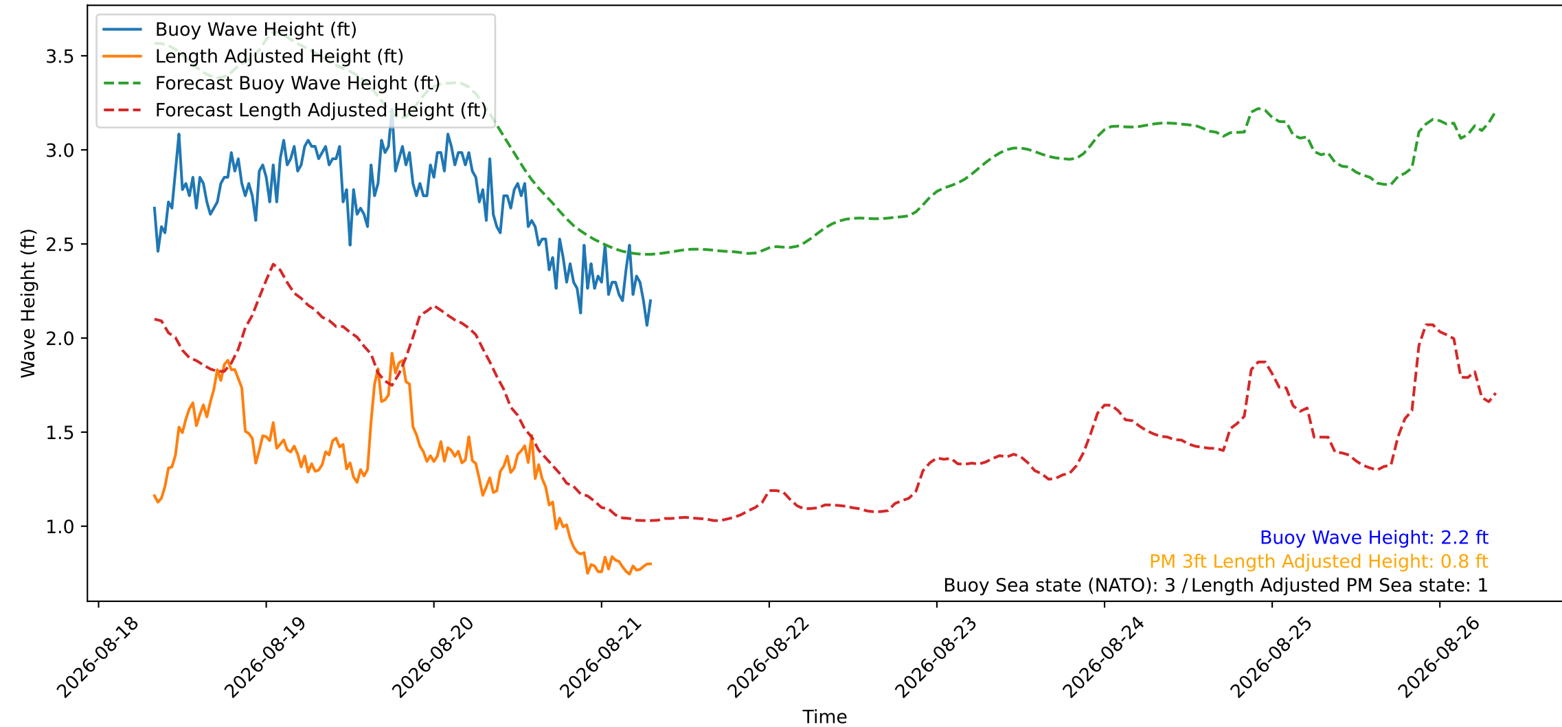
Wave Heights over Time for Red Beach at 2026-08-21 07:50:46
