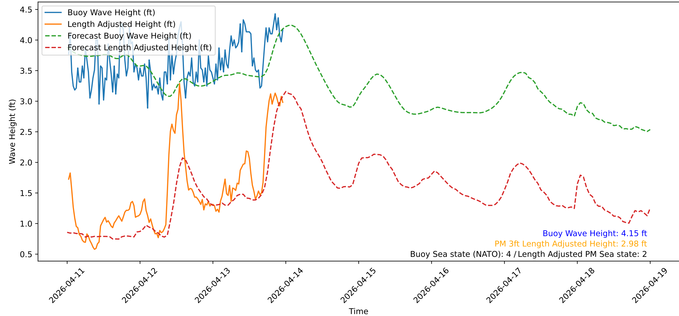
Wave Heights over Time for Red Beach at 2026-04-14 00:00:50
