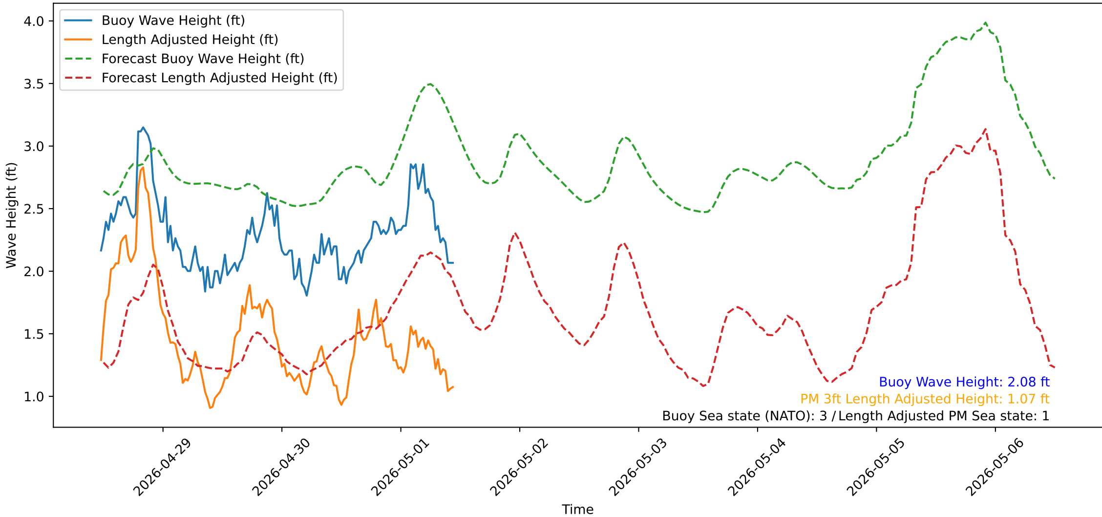
Wave Heights over Time for Green Beach at 2026-05-01 11:31:13
