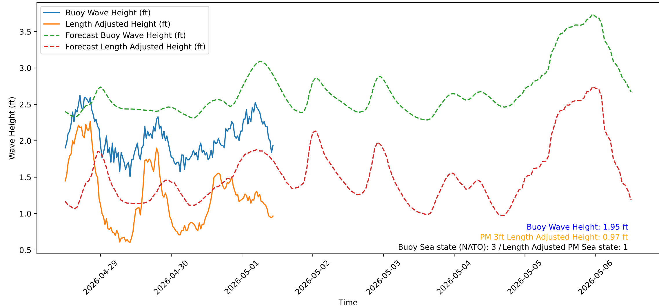
Wave Heights over Time for Red Beach at 2026-05-01 11:30:51
