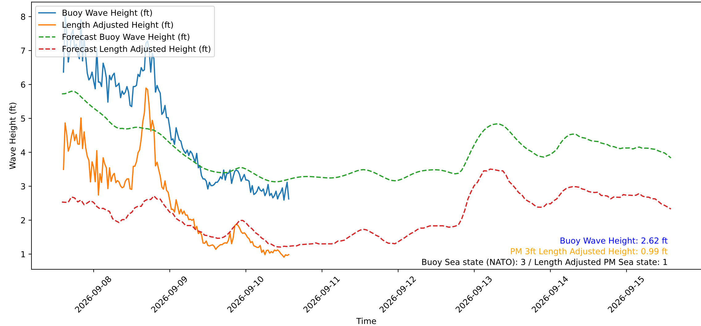
Wave Heights over Time for Green Beach at 2026-09-10 14:11:12
