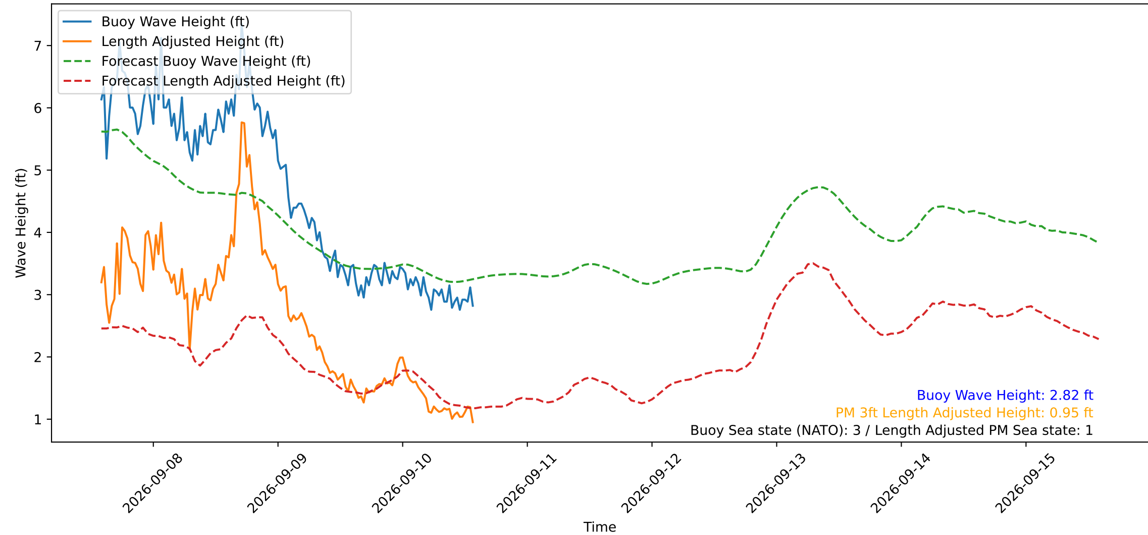
Wave Heights over Time for Oceanside Harbor at 2026-09-10 14:10:29
