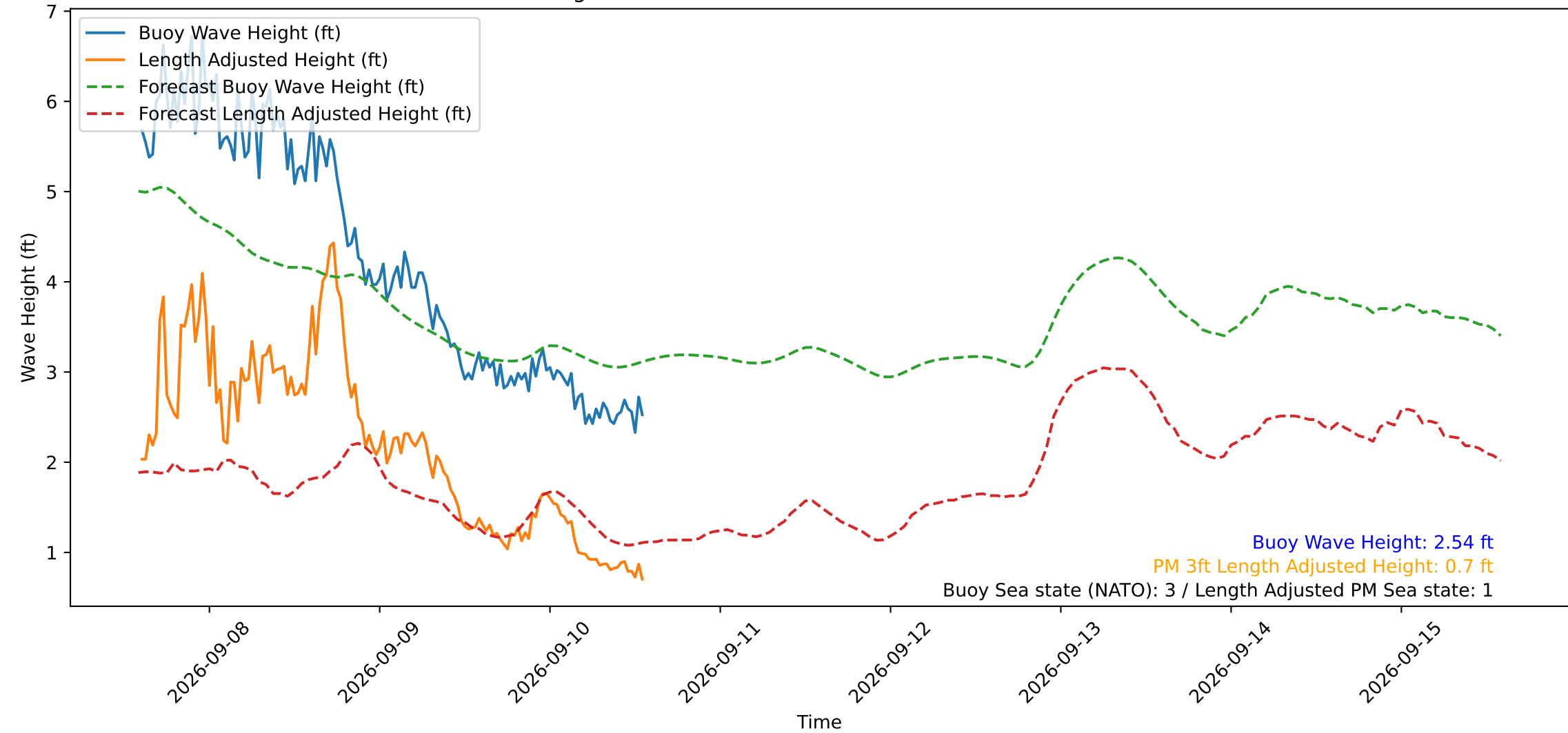
Wave Heights over Time for Red Beach at 2026-09-10 14:10:49
