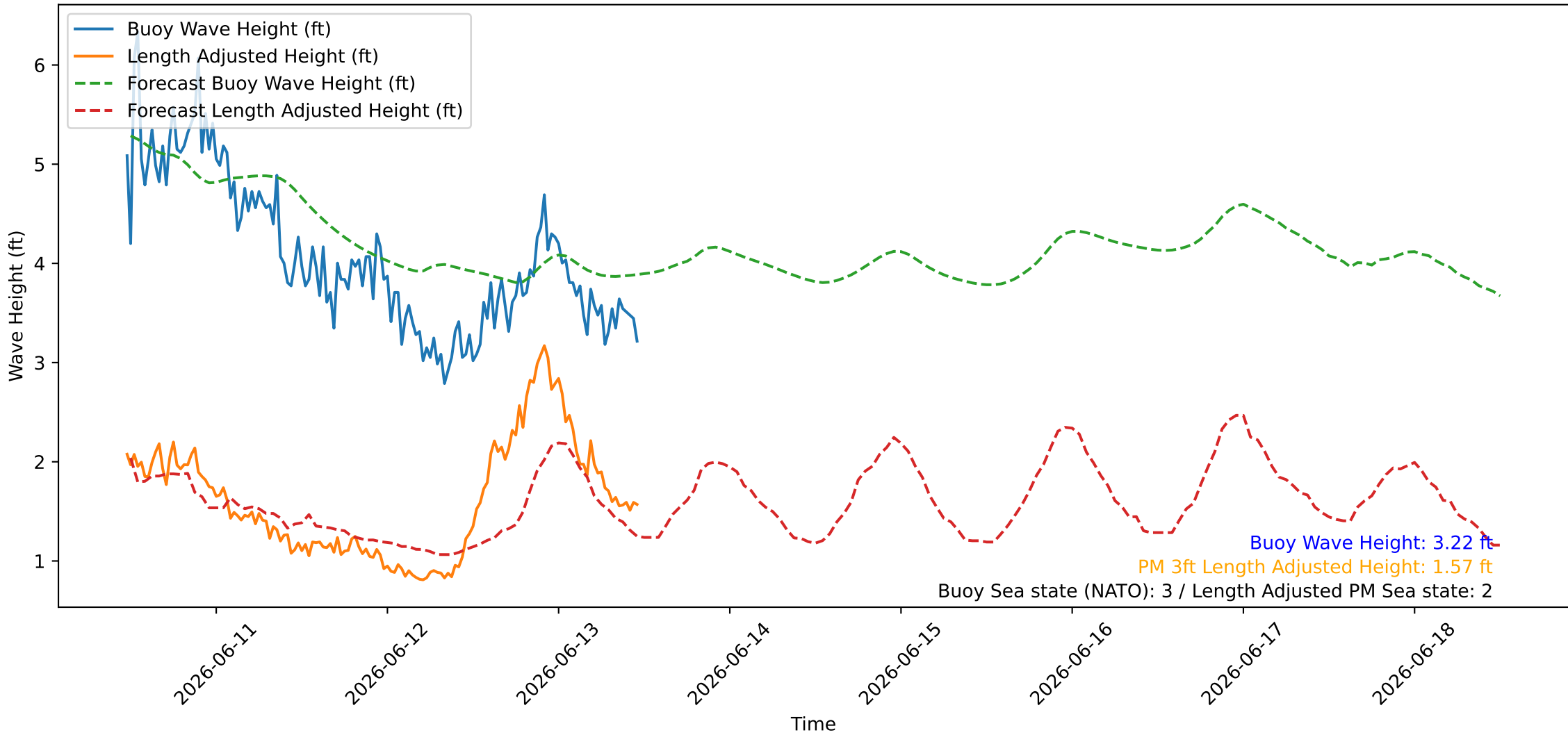
Wave Heights over Time for Oceanside Harbor at 2026-06-13 11:30:26
