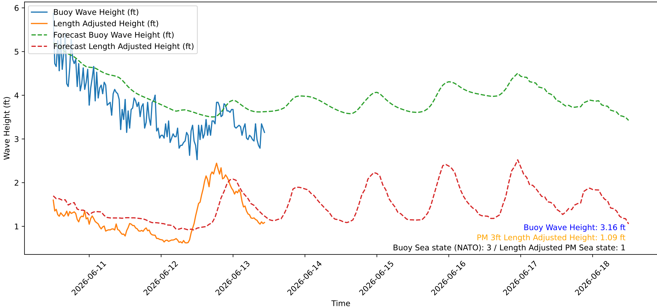
Wave Heights over Time for Red Beach at 2026-06-13 11:30:46
