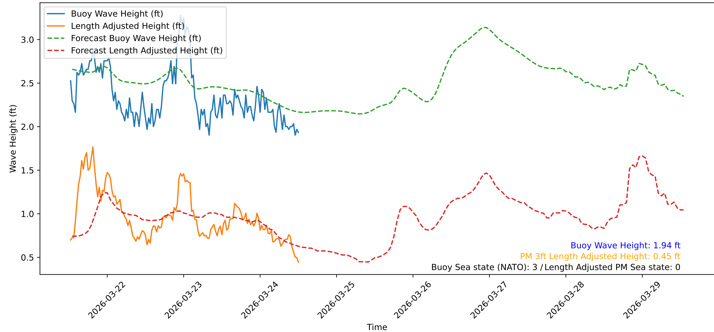
Wave Heights over Time for Green Beach at 2026-03-24 12:41:10
