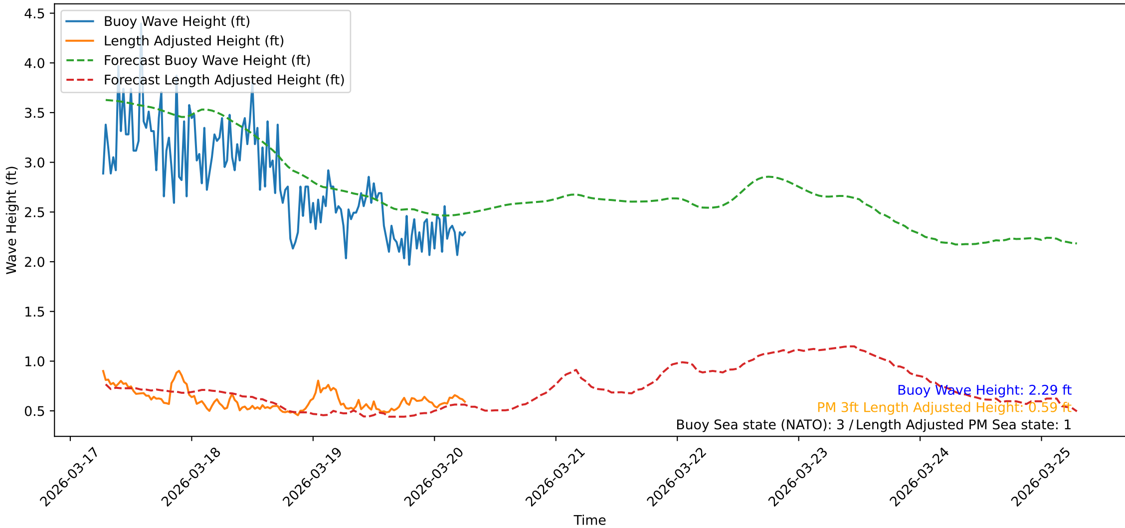
Wave Heights over Time for Oceanside Harbor at 2026-03-20 06:30:32
