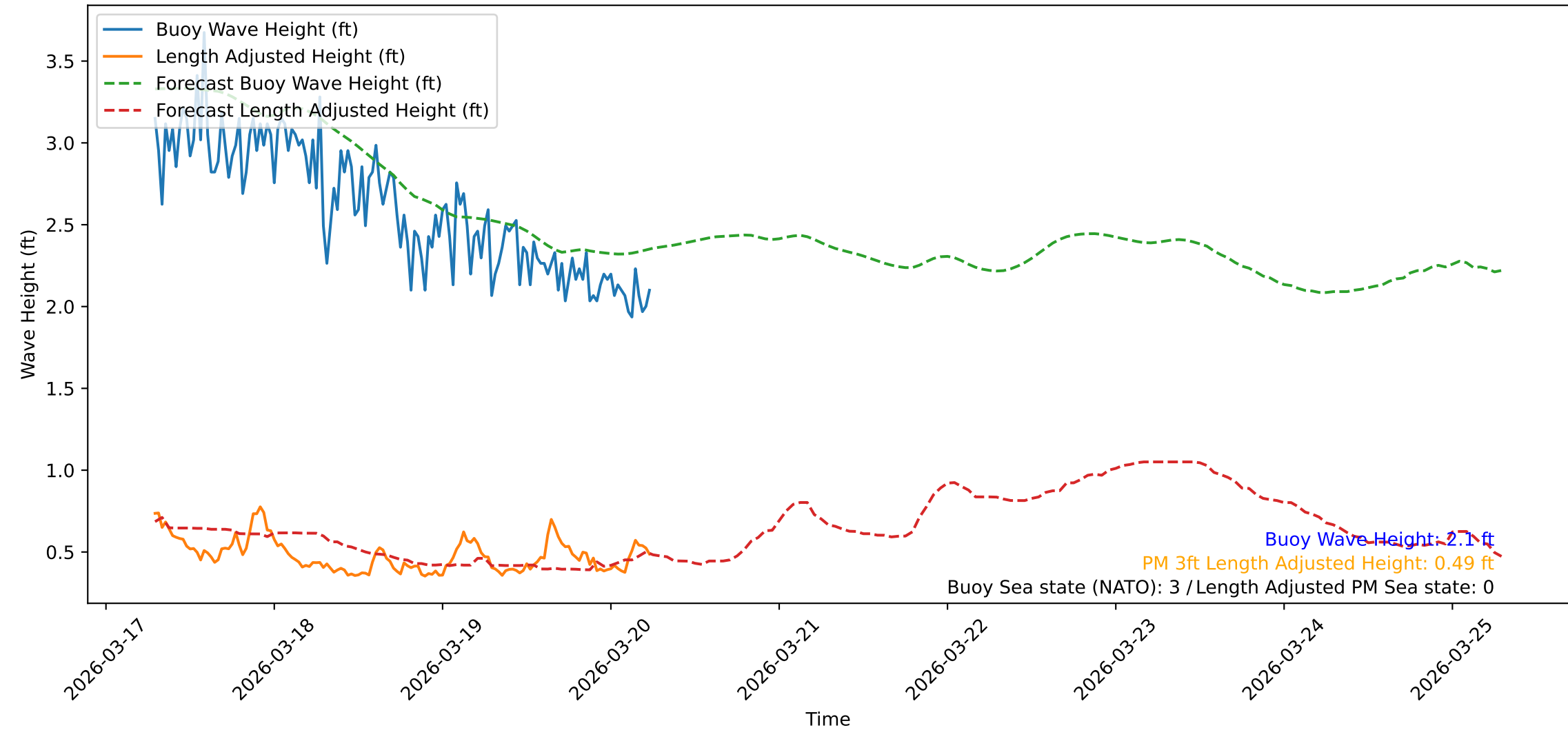
Wave Heights over Time for Red Beach at 2026-03-20 06:30:48
