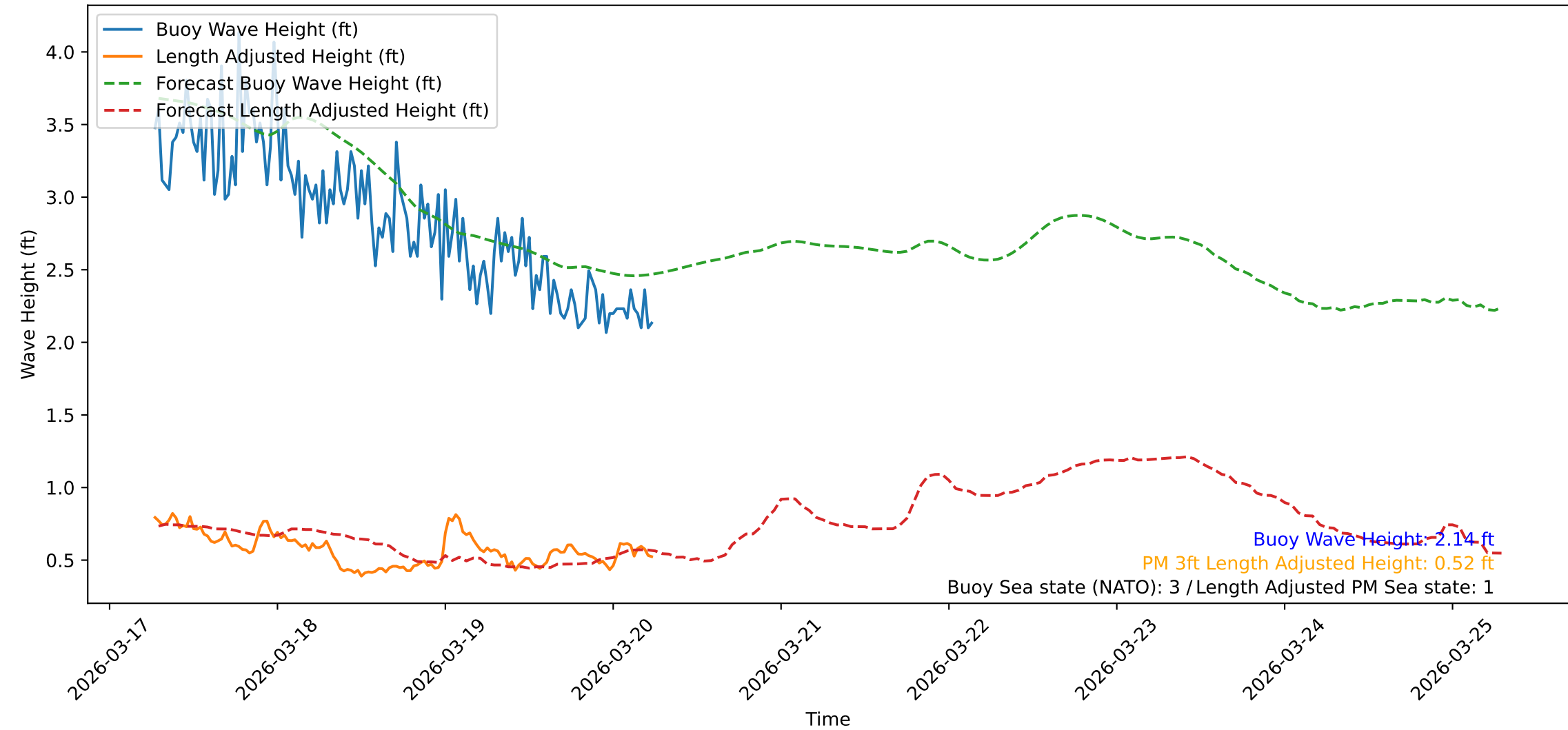
Wave Heights over Time for Green Beach at 2026-03-20 06:31:10
