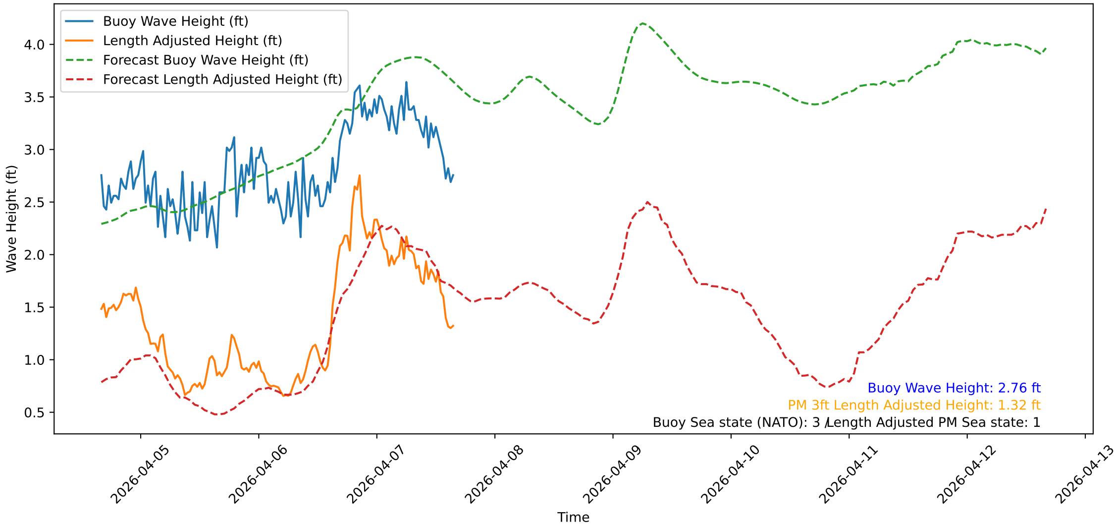
Wave Heights over Time for Oceanside Harbor at 2026-04-07 16:10:32
