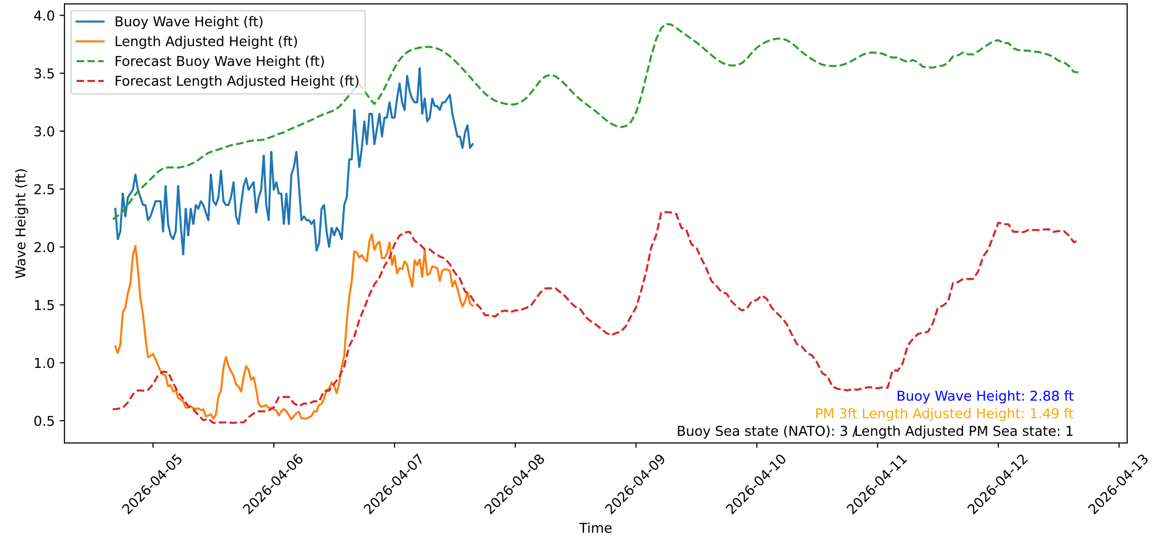
Wave Heights over Time for Red Beach at 2026-04-07 16:10:48
