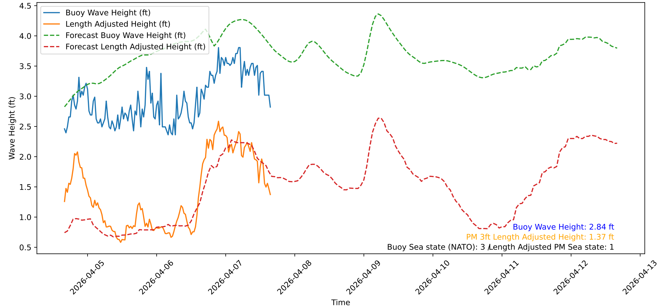
Wave Heights over Time for Green Beach at 2026-04-07 16:11:11
