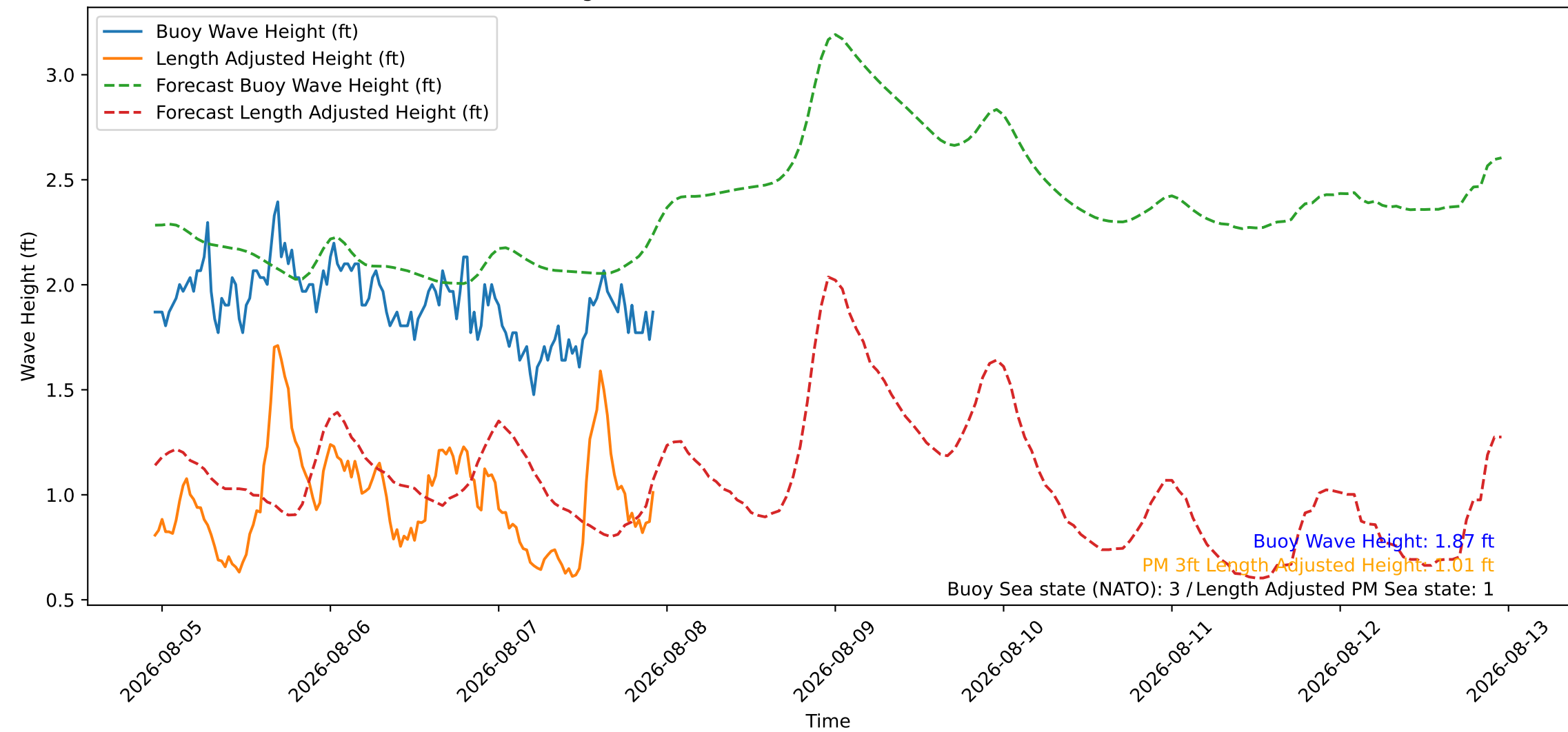
Wave Heights over Time for Red Beach at 2026-08-07 22:50:47
