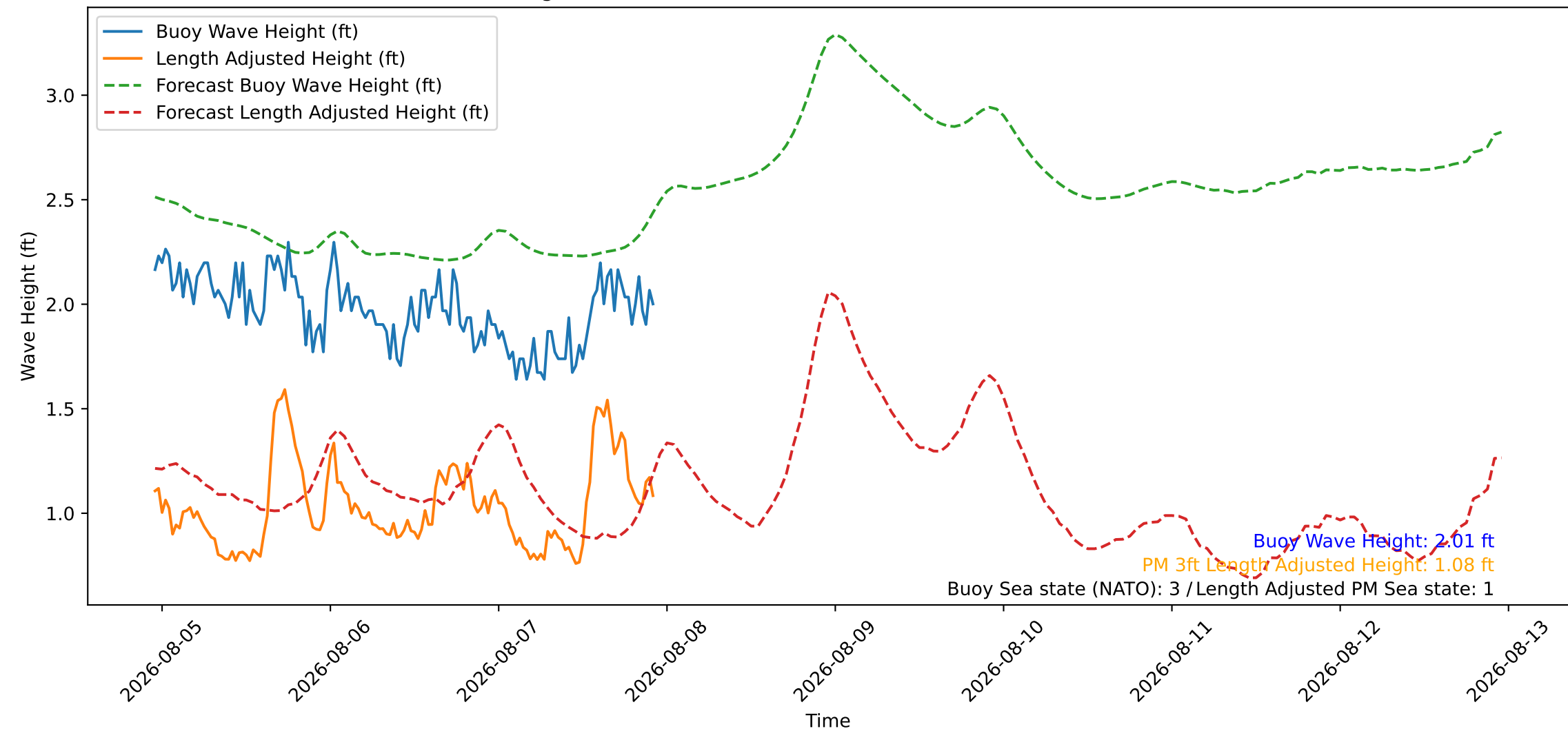
Wave Heights over Time for Oceanside Harbor at 2026-08-07 22:50:26
