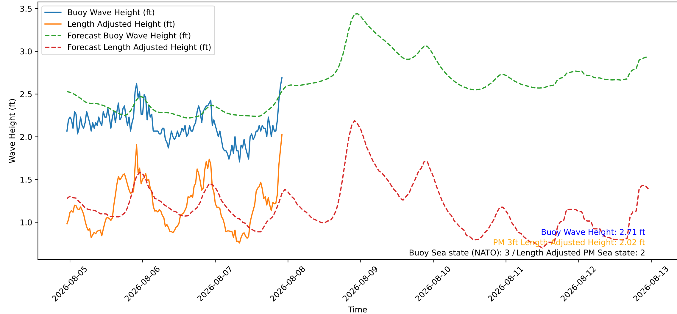
Wave Heights over Time for Green Beach at 2026-08-07 22:51:09
